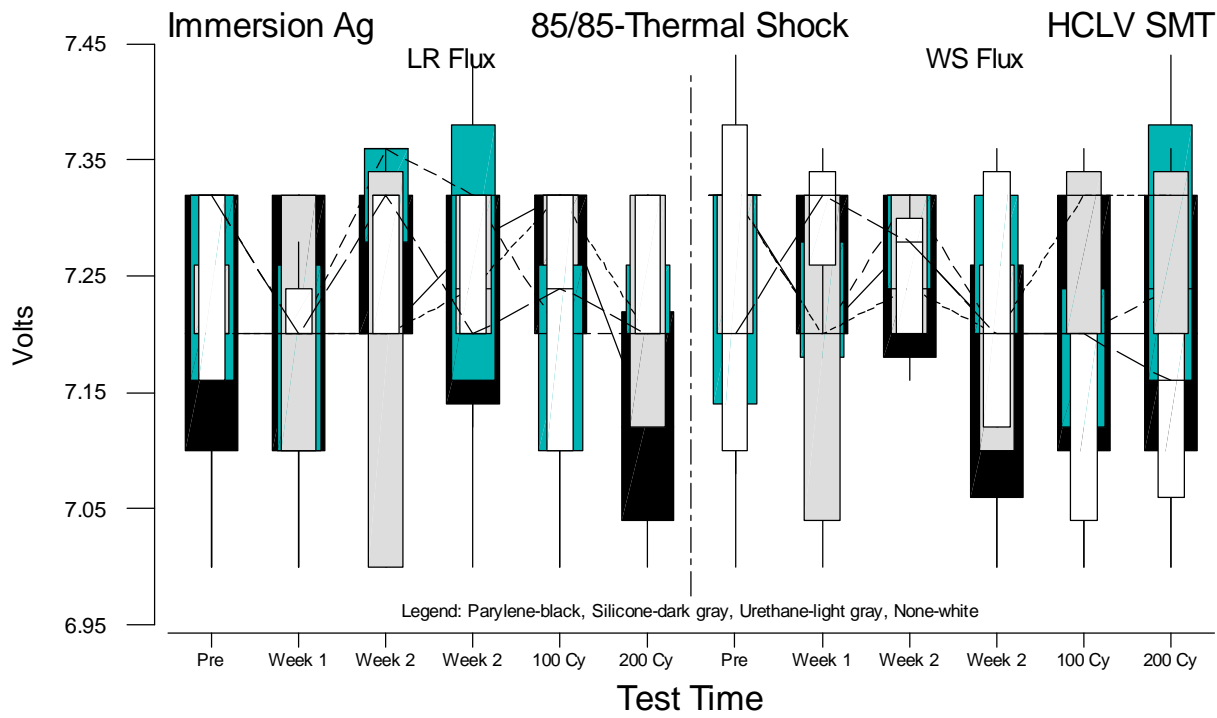
Figure F.7 Boxplots of HCLV SMT Voltage Measurements for Immersion Ag versus Test Time
