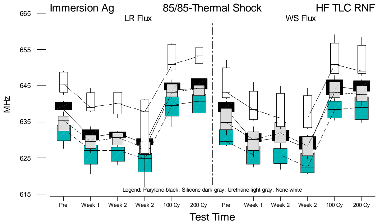
Figure F.63 Boxplots of HF TLC Rev. Null Frequency Measurements for Immersion Ag vs. Test Time
