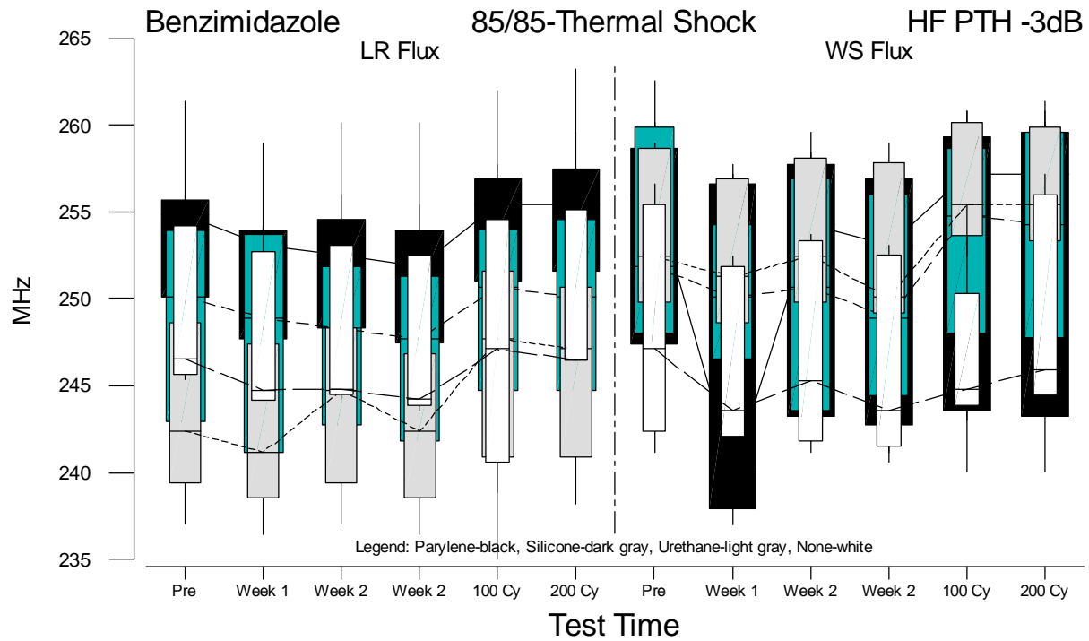
Figure F.30 Boxplots of HF PTH f(-3dB) Measurements for Benzimidazole versus Test Time
