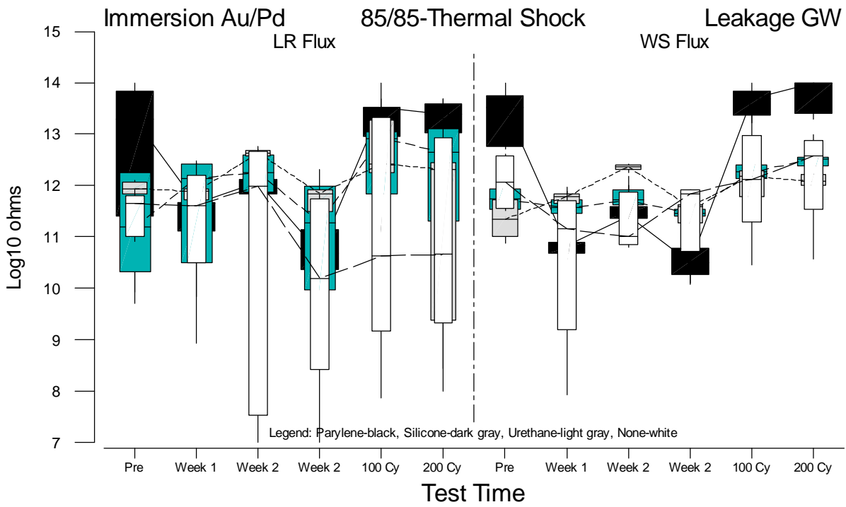
Figure F.84 Boxplots of Gull Wing Leakage Measurements for Immersion Au/Pd vs. Test Time
