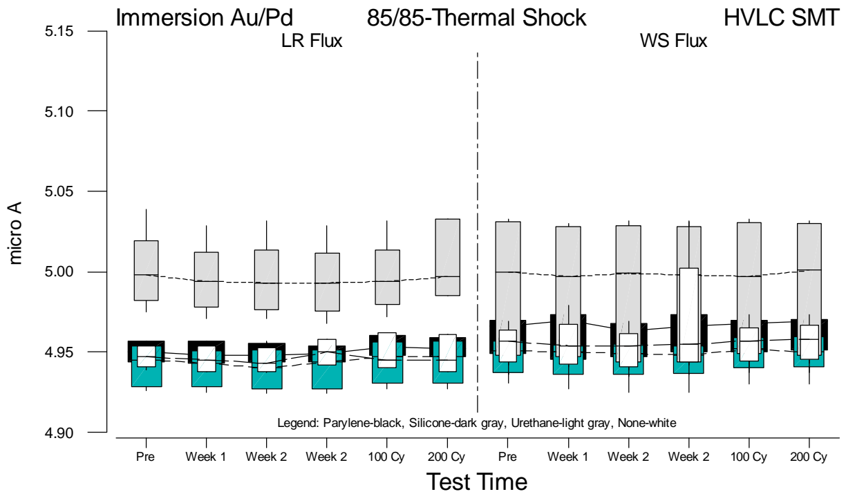
Figure F.16 Boxplots of HVLC SMT Current Measurements for Immersion Au/Pd vs. Test Time
