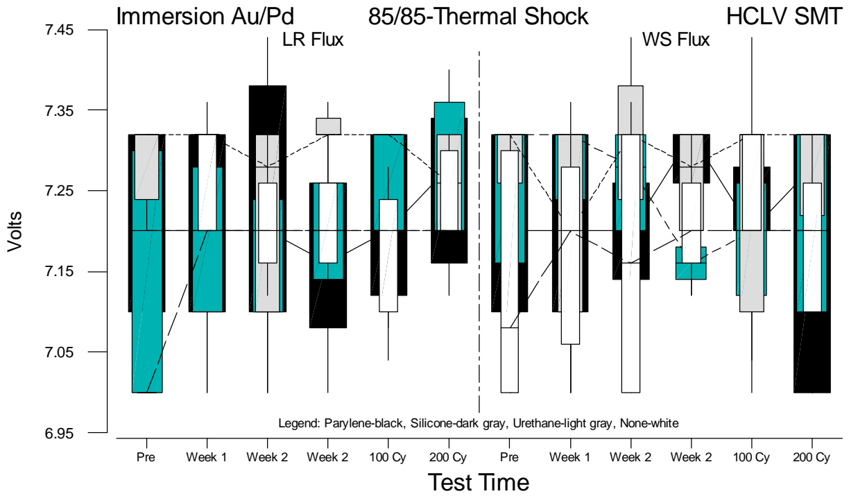
Figure F.8 Boxplots of HCLV SMT Voltage Measurements for Immersion Au/Pd versus Test Time
