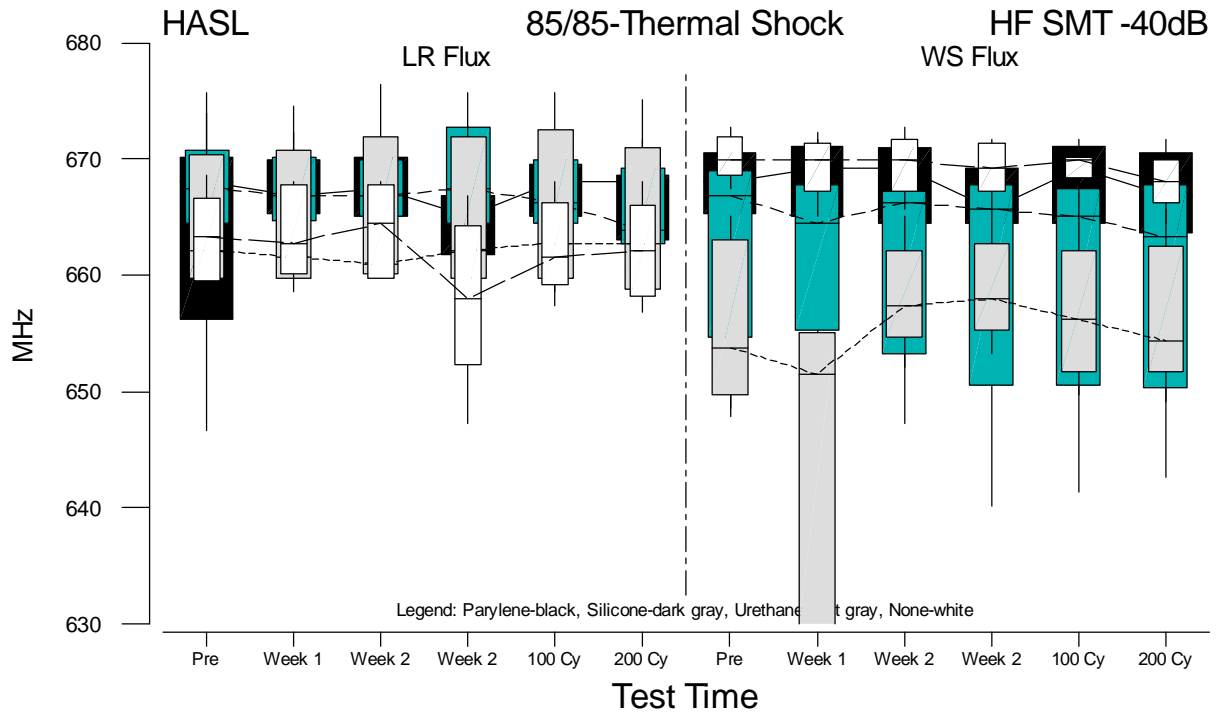
Figure F.45 Boxplots of HF SMT f(-40dB) Measurements for HASL versus Test Time
