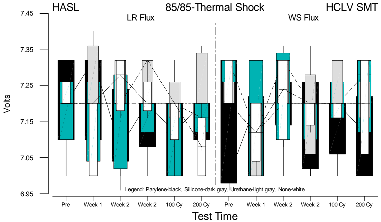
Figure F.5 Boxplots of HCLV SMT Voltage Measurements for HASL versus Test Time
