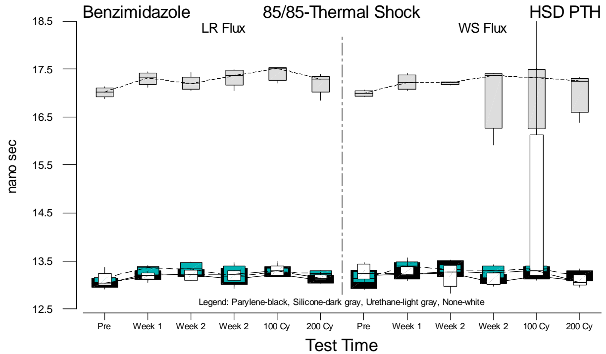
Figure F.18 Boxplots of HSD PTH Propagation Delay Measurements for Benzimidazole versus Test Time
