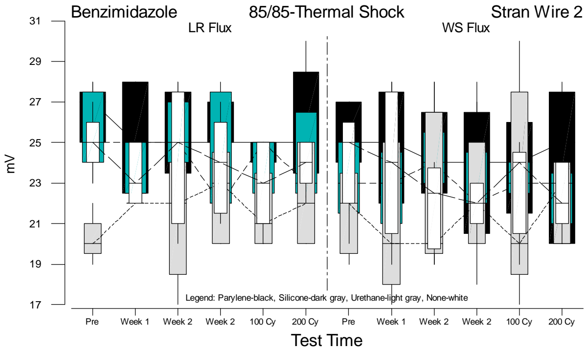
Figure F.90 Boxplots of Stranded Wire 2 Voltage Measurements for Benzimidazole versus Test Time
