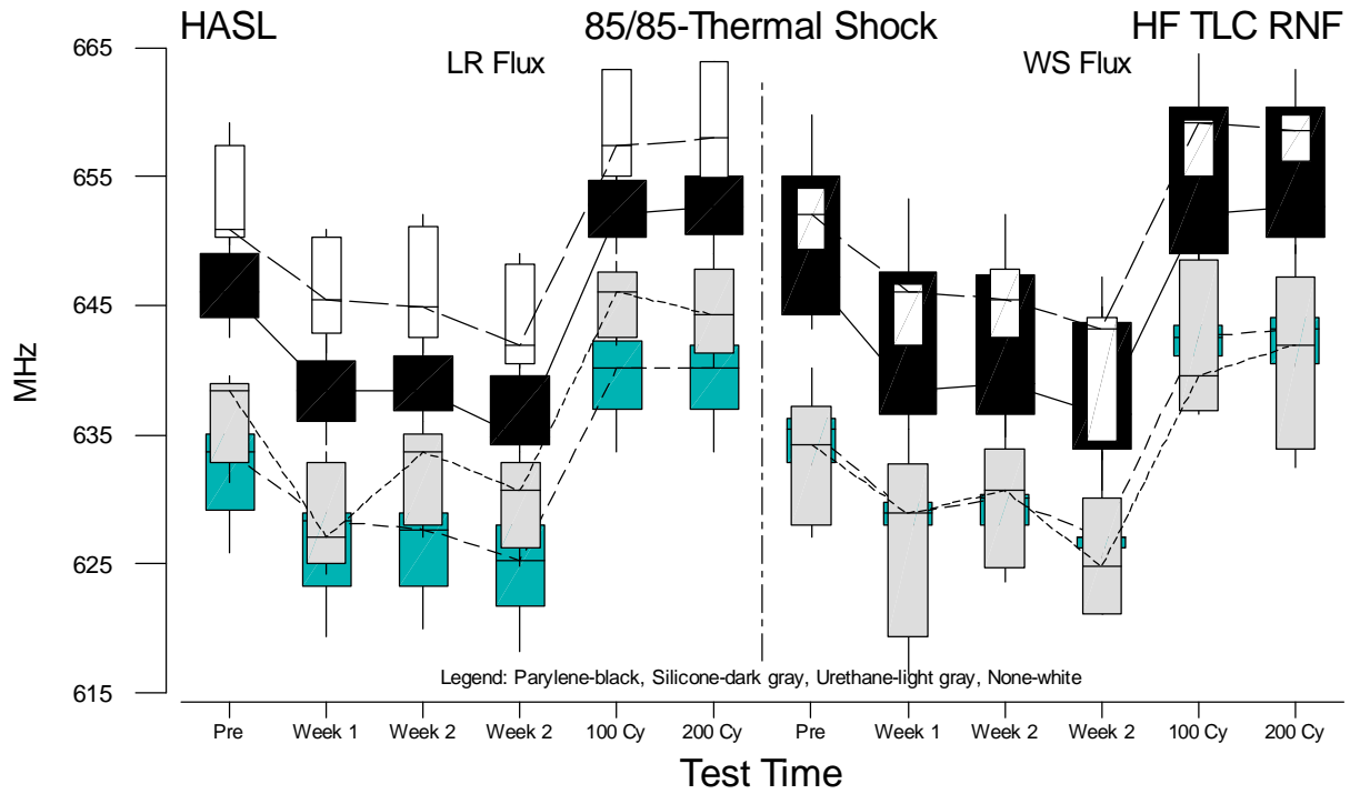
Figure F.61 Boxplots of HF TLC Rev. Null Frequency Measurements for HASL versus Test Time
