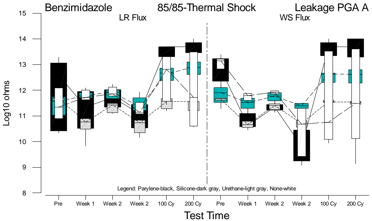
Figure F.74 Boxplots of PGA-A Leakage Measurements for Benzimidazole versus Test Time
