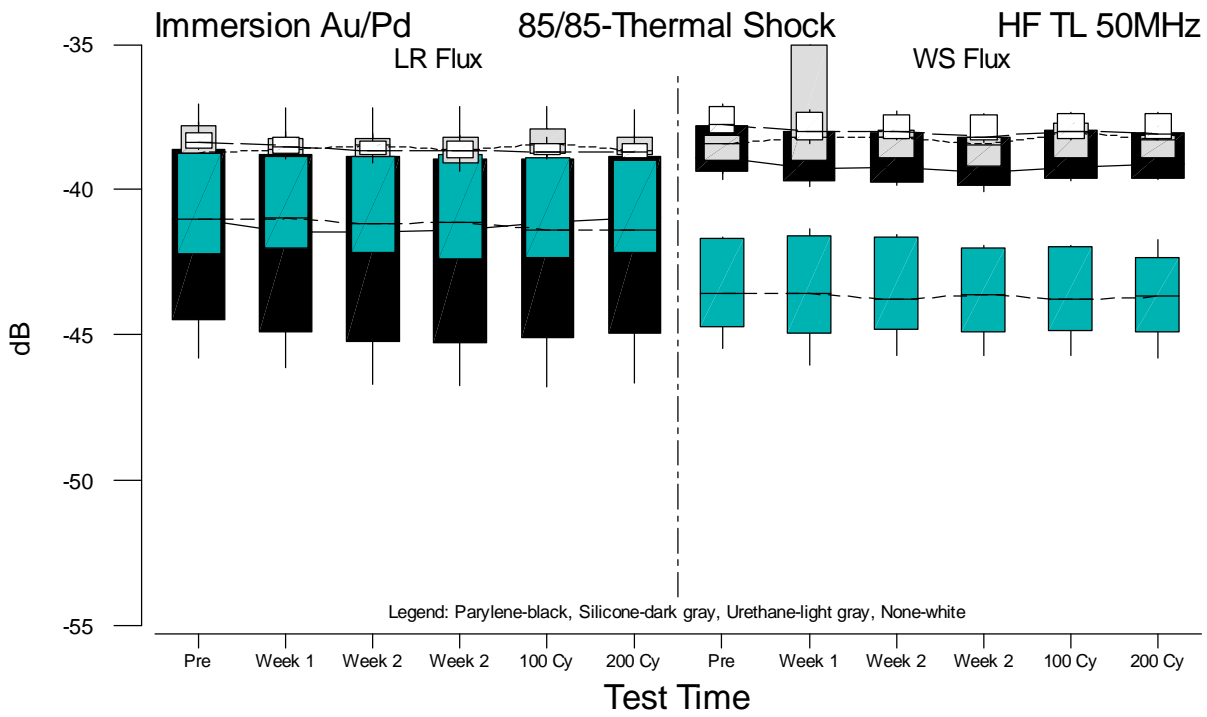
Figure F.52 Boxplots of HF TLC 50MHz Measurements for Immersion Au/Pd versus Test Time
