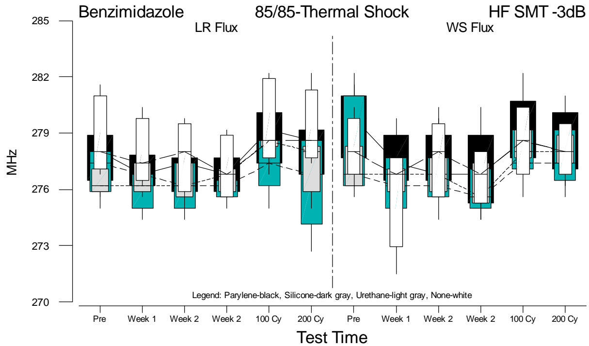
Figure F.42 Boxplots of HF SMT f(-3dB) Measurements for Benzimidazole versus Test Time
