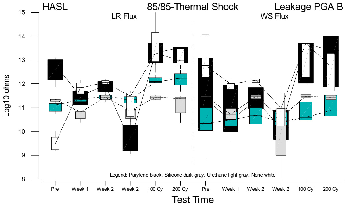
Figure F.77 Boxplots of PGA-B Leakage Measurements for HASL versus Test Time
