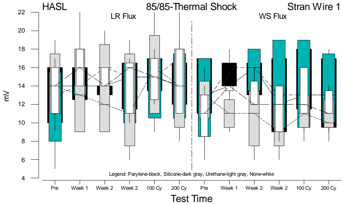
Figure F.85 Boxplots of Stranded Wire 1 Voltage Measurements for HASL versus Test Time
