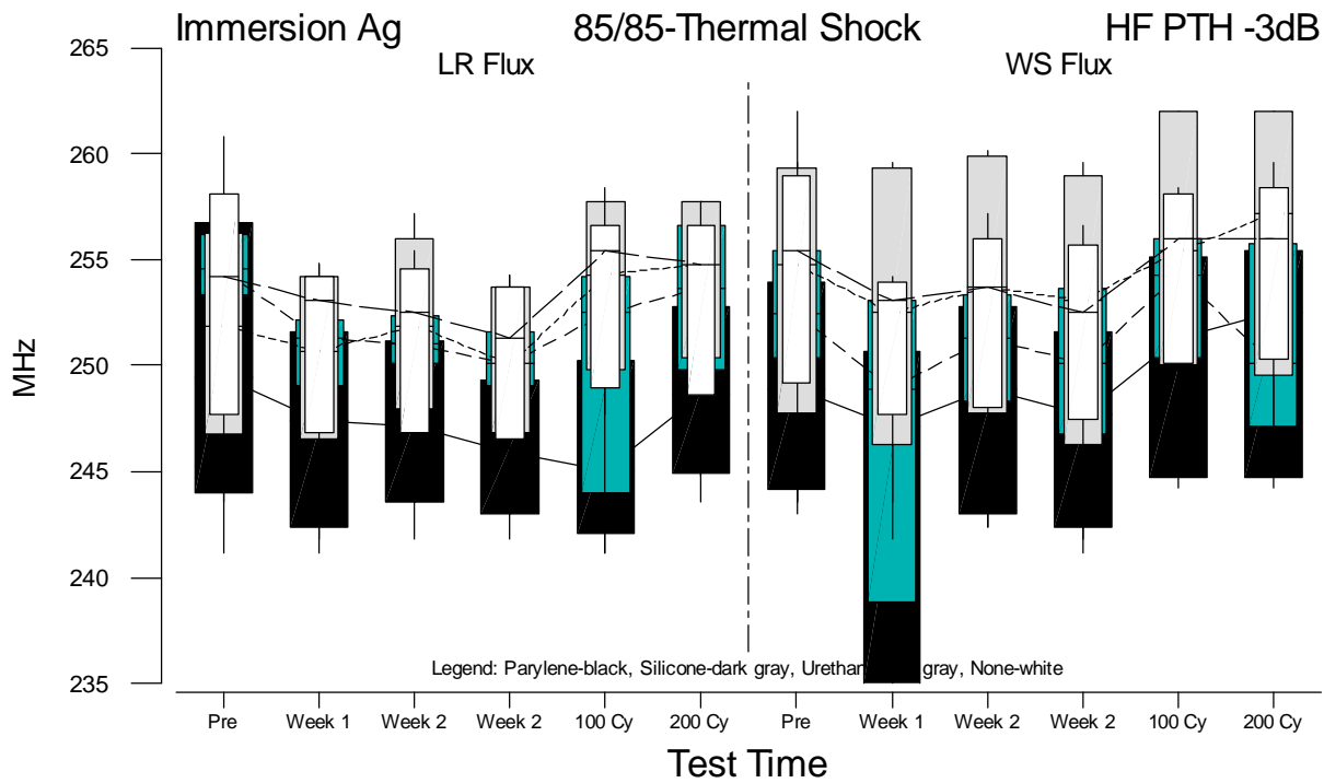
Figure F.31 Boxplots of HF PTH f(-3dB) Measurements for Immersion Ag versus Test Time
