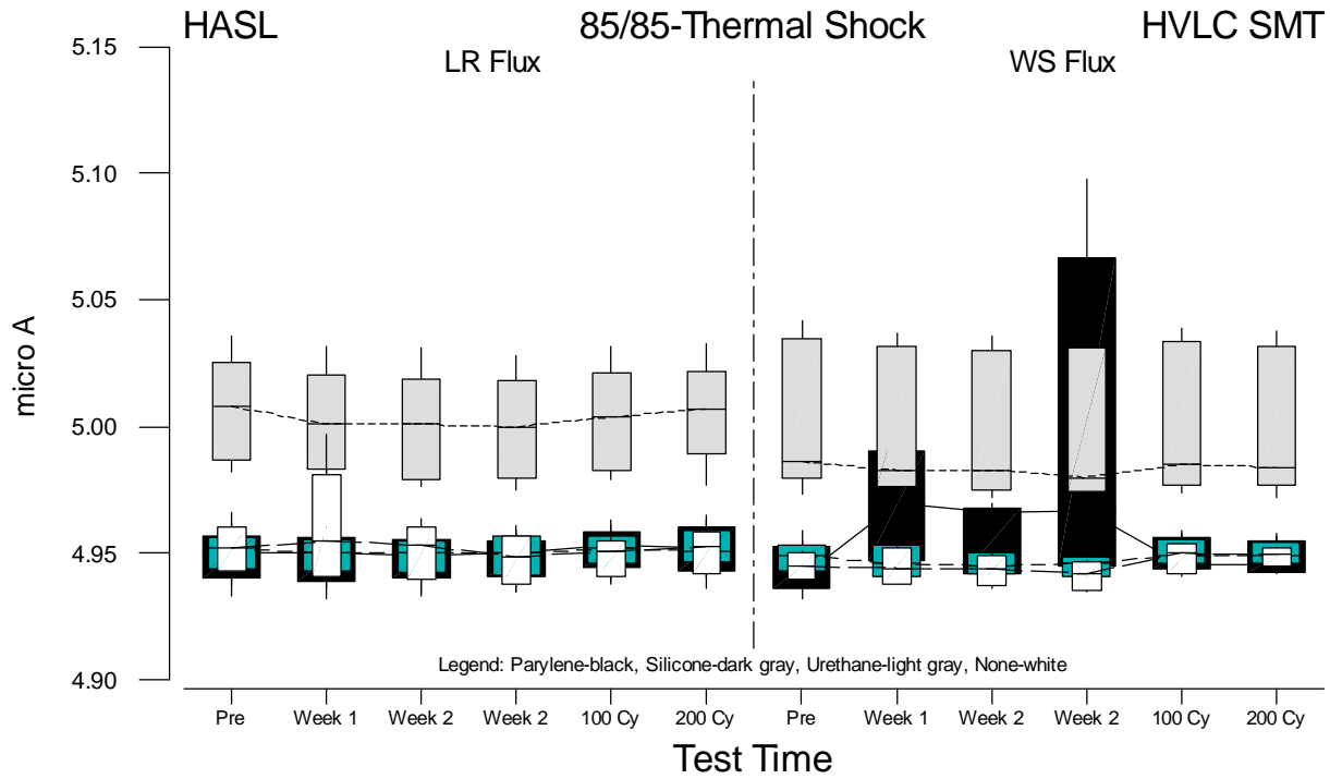
Figure F.13 Boxplots of HVLC SMT Current Measurements for HASL versus Test Time
