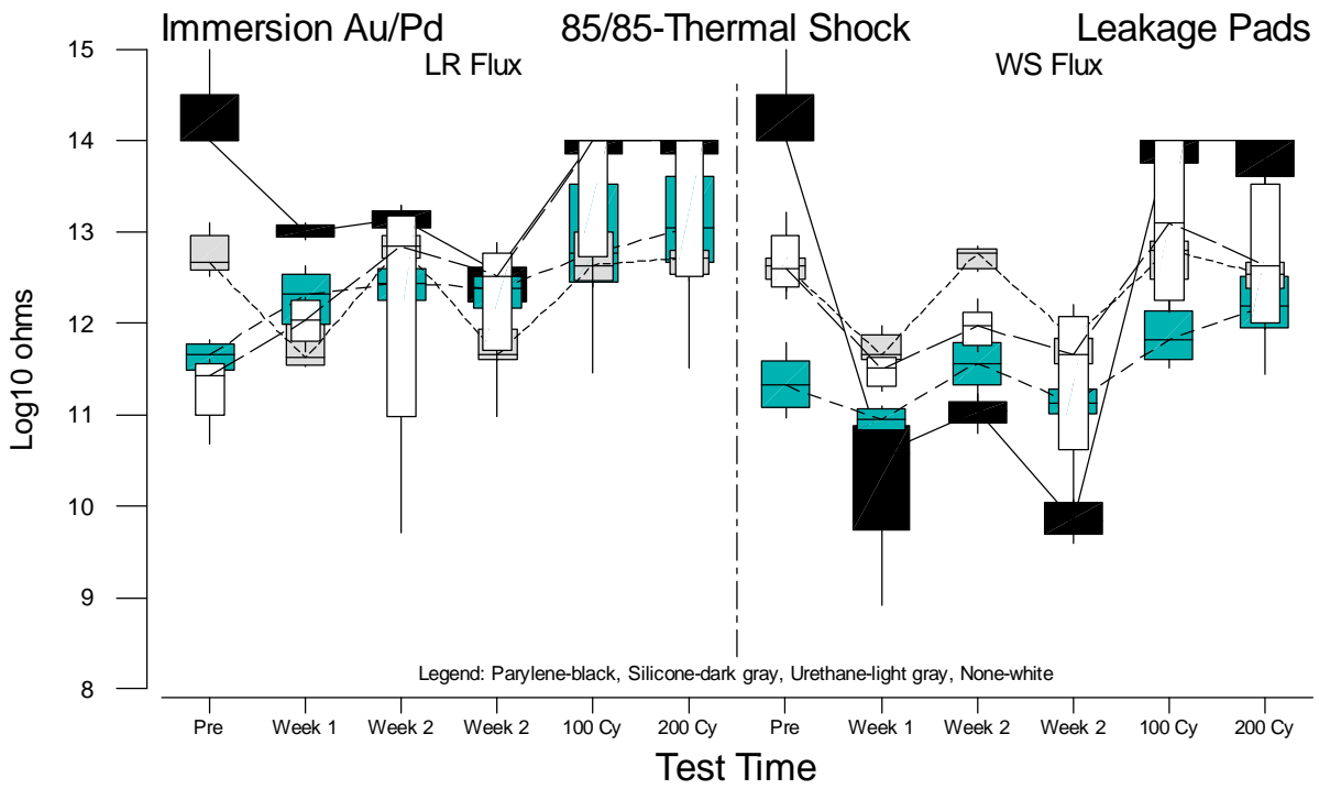
Figure F.72 Boxplots of 10-Mil Leakage Measurements for Immersion Au/Pd versus Test Time
