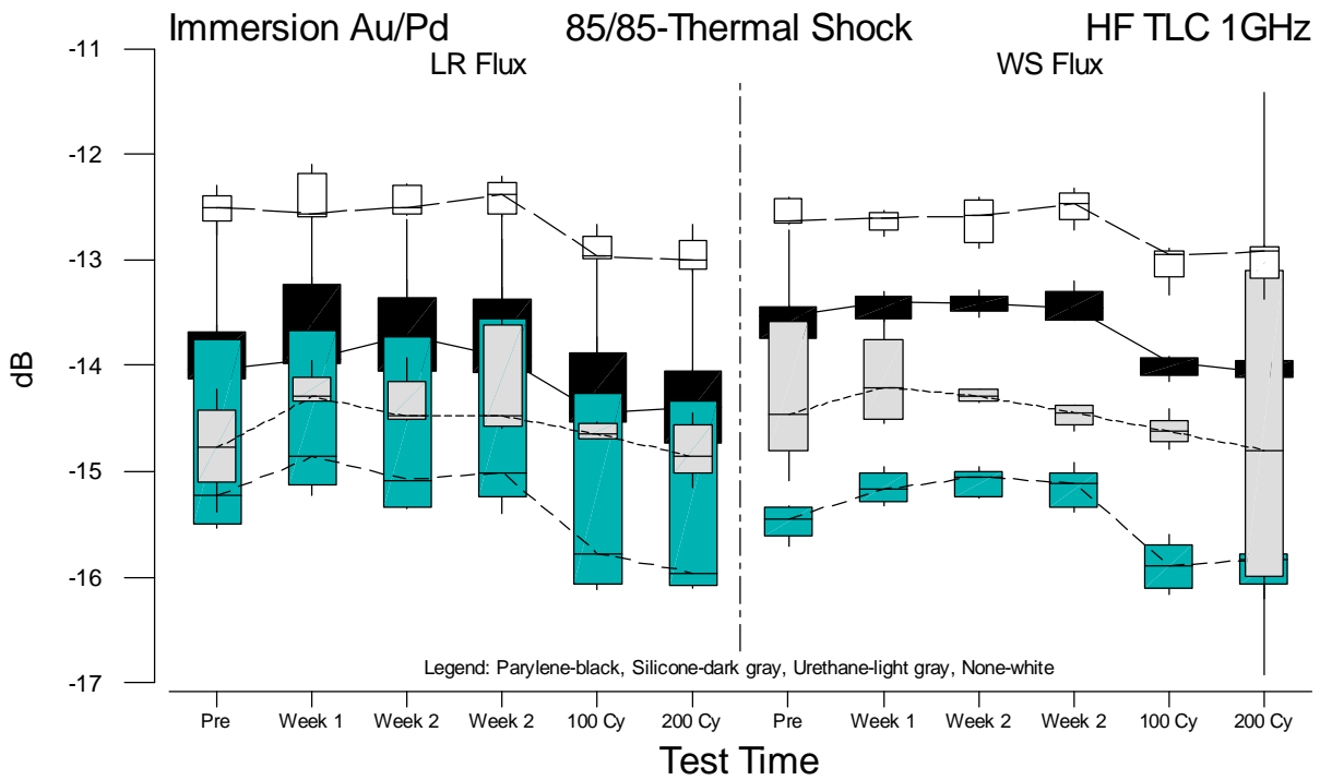
Figure F.60 Boxplots of HF TLC 1GHz Measurements for Immersion Au/Pd versus Test Time
