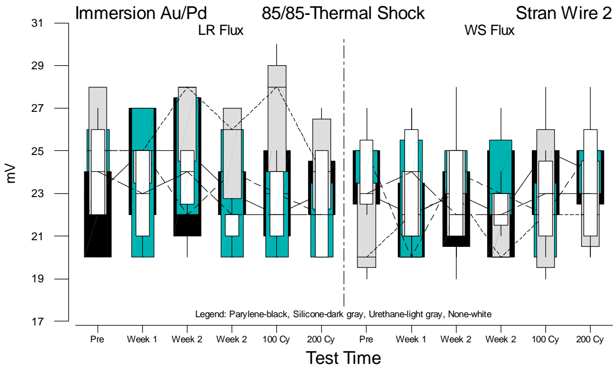
Figure F.92 Boxplots of Stranded Wire 2 Voltage Measurements for Immersion Au/Pd versus Test Time
