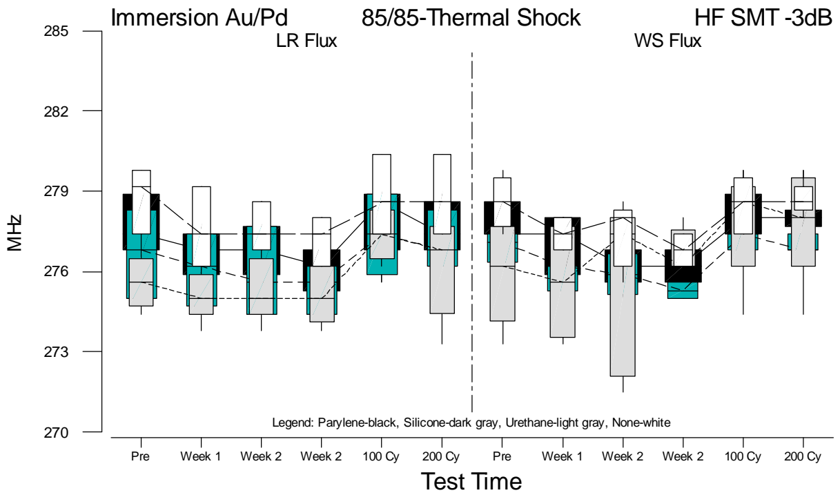
Figure F.44 Boxplots of HF SMT f(-3dB) Measurements for Immersion Au/Pd versus Test Time
