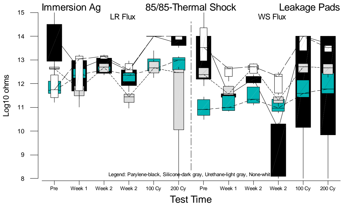
Figure F.71 Boxplots of 10-Mil Leakage Measurements for Immersion Ag versus Test Time
