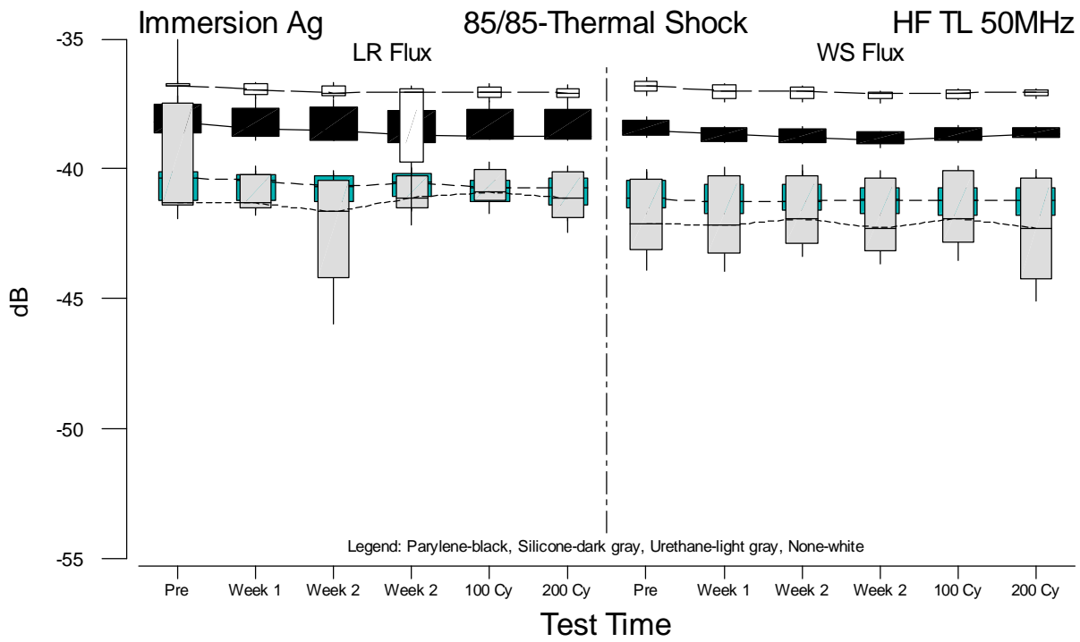
Figure F.51 Boxplots of HF TLC 50MHz Measurements for Immersion Ag versus Test Time
