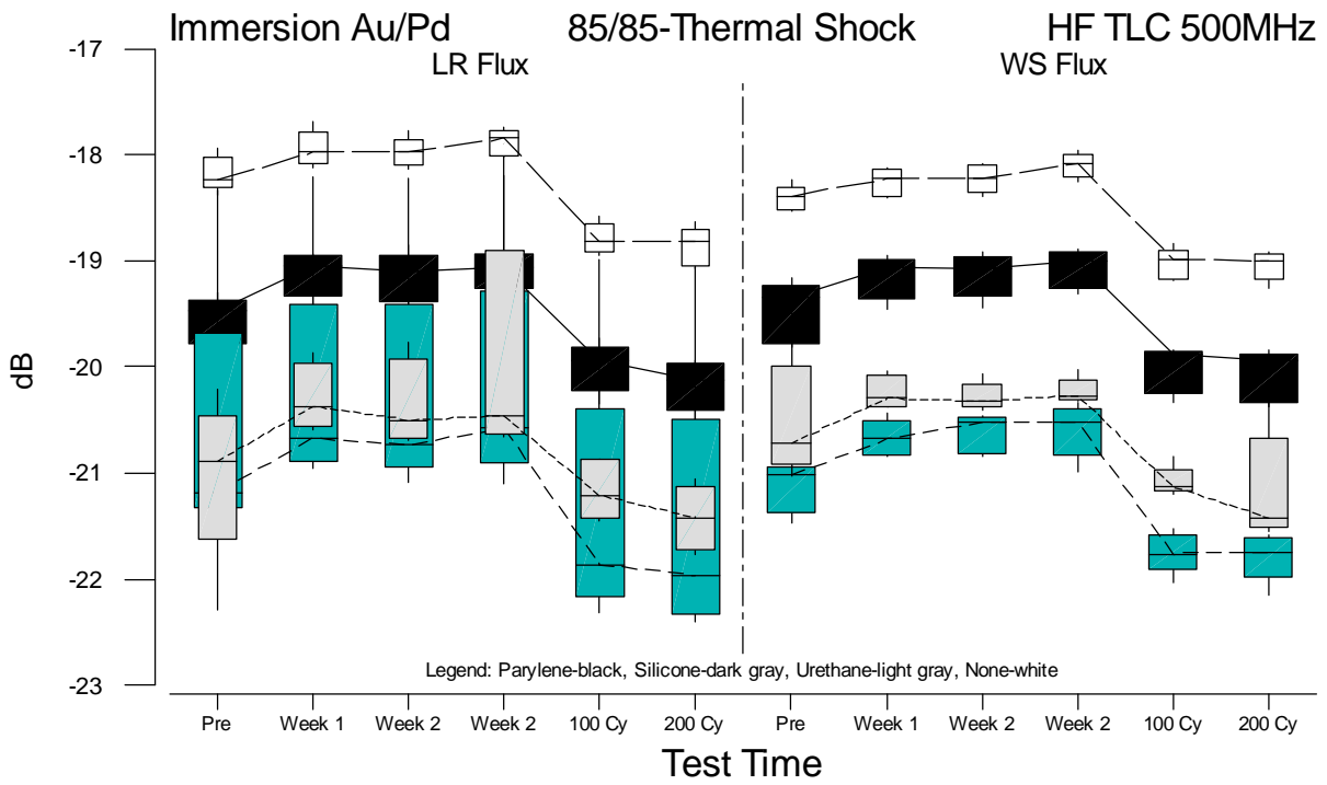
Figure F.56 Boxplots of HF TLC 500MHz Measurements for Immersion Au/Pd versus Test Time
