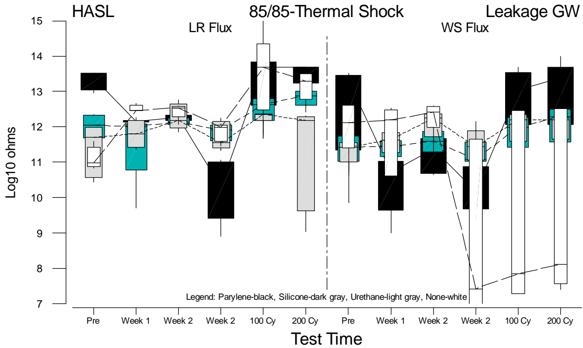
Figure F.81 Boxplots of Gull Wing Leakage Measurements for HASL versus Test Time
