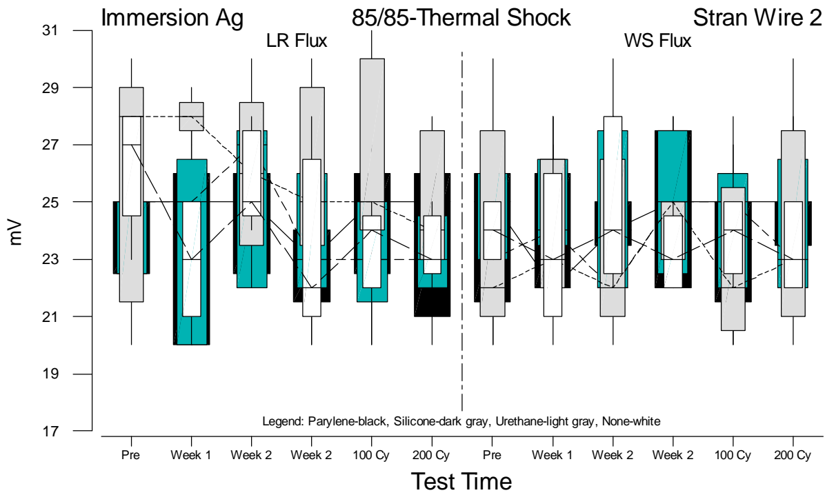
Figure F.91 Boxplots of Stranded Wire 2 Voltage Measurements for Immersion Ag versus Test Time
