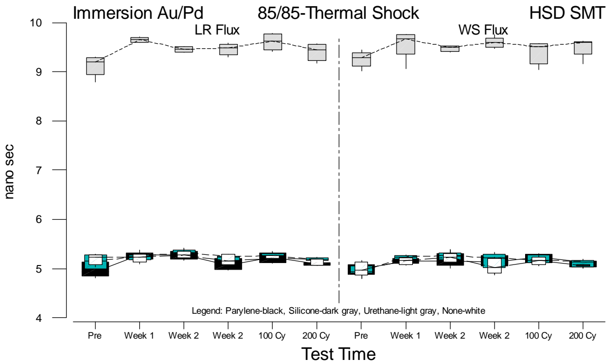
Figure F.24 Boxplots of HSD SMT Propagation Delay Measurements for Immersion Au/Pd vs. Test Time
