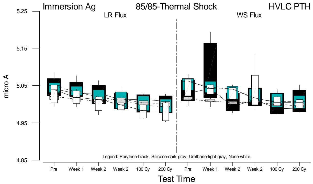
Figure F.11 Boxplots of HVLC PTH Current Measurements for Immersion Ag versus Test Time
