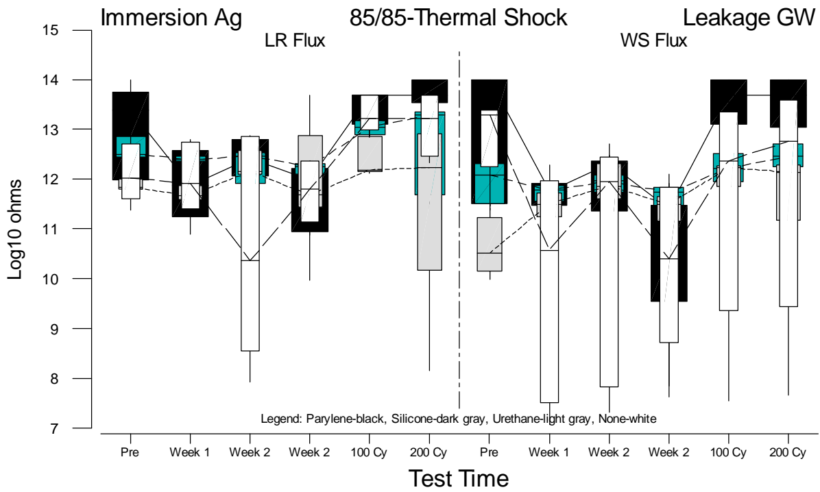
Figure F.83 Boxplots of Gull Wing Leakage Measurements for Immersion Ag versus Test Time
