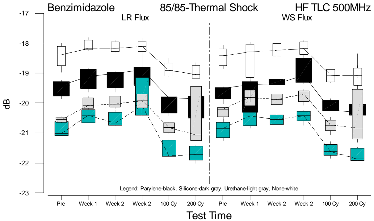
Figure F.54 Boxplots of HF TLC 500MHz Measurements for Benzimidazole versus Test Time
