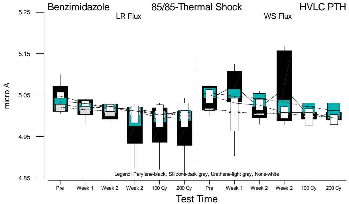
Figure F.10 Boxplots of HVLC PTH Current Measurements for Benzimidazole versus Test Time
