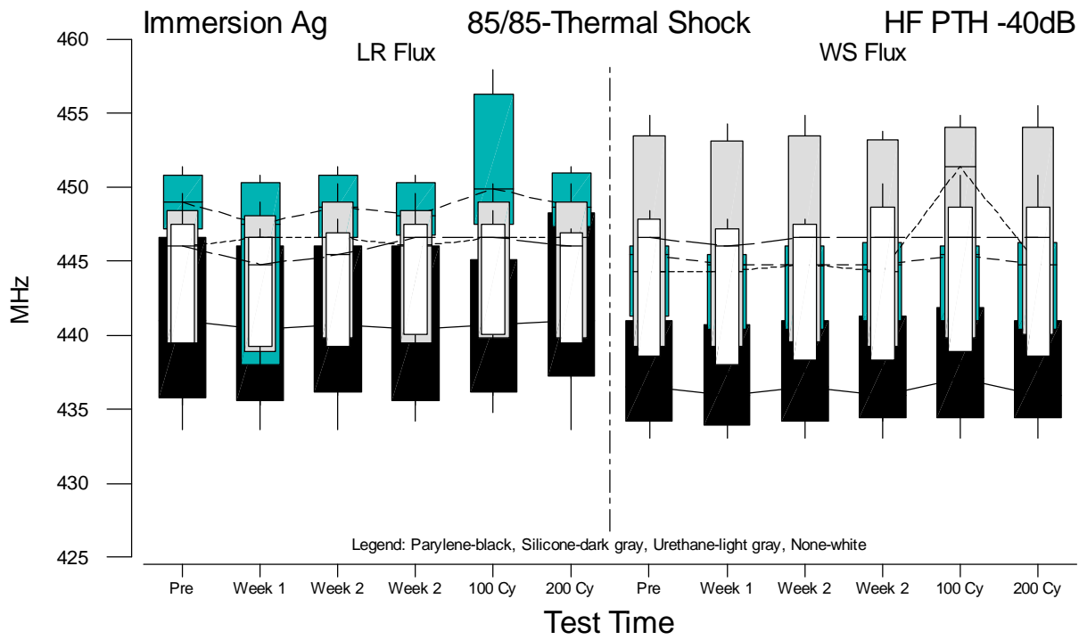
Figure F.35 Boxplots of HF PTH f(-40B) Measurements for Immersion Ag versus Test Time
