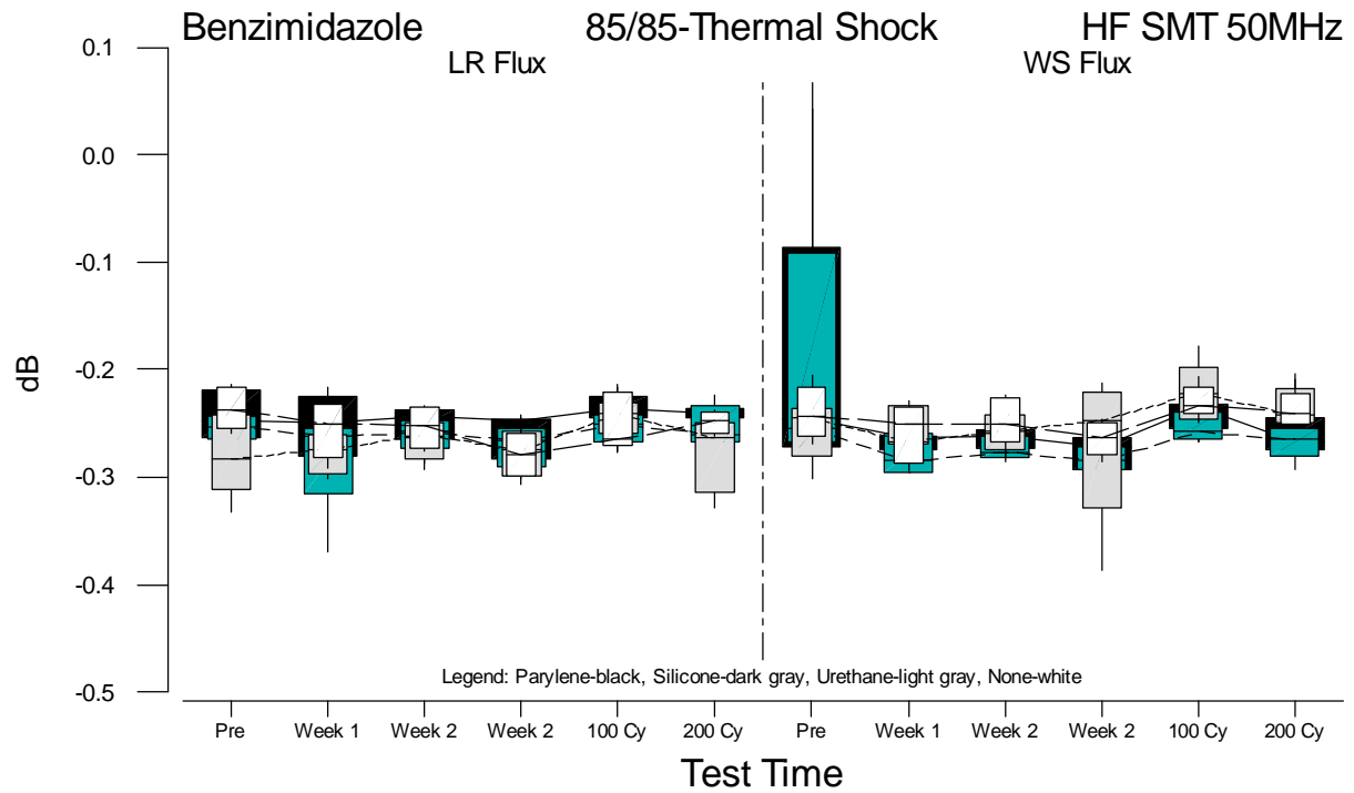
Figure F.38 Boxplots of HF SMT 50MHz Measurements for Benzimidazole versus Test Time
