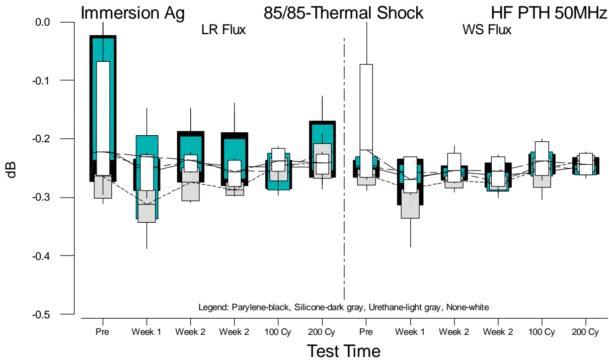
Figure F.27 Boxplots of HF PTH 50MHz Measurements for Immersion Ag versus Test Time
