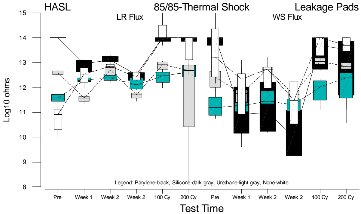
Figure F.69 Boxplots of 10-Mil Leakage Measurements for HASL versus Test Time
