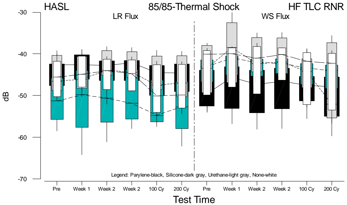
Figure F.65 Boxplots of HF TLC Rev. Null Response Measurements for HASL versus Test Time
