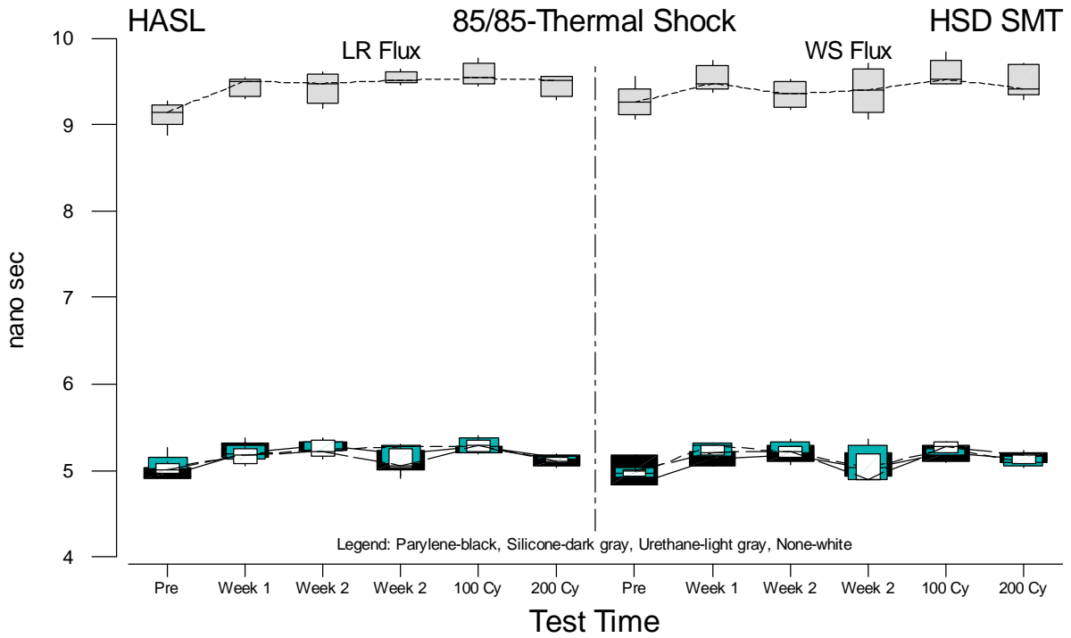
Figure F.21 Boxplots of HSD SMT Propagation Delay Measurements for HASL versus Test Time
