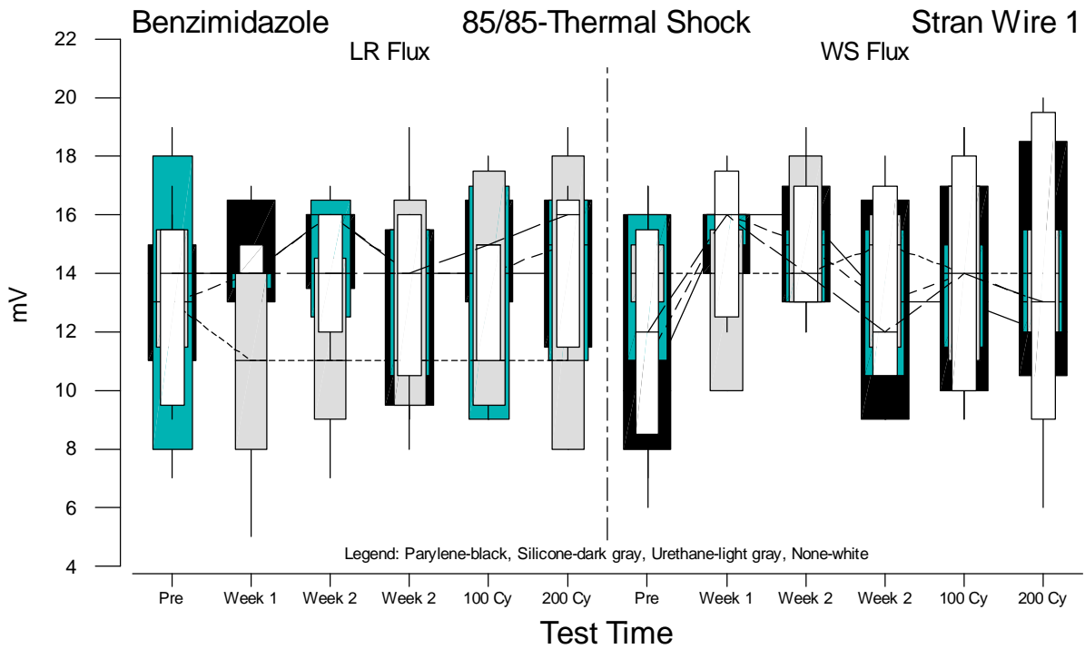
Figure F.86 Boxplots of Stranded Wire 1 Voltage Measurements for Benzimidazole versus Test Time
