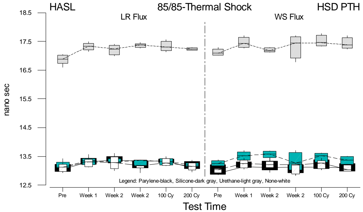
Figure F.17 Boxplots of HSD PTH Propagation Delay Measurements for HASL versus Test Time
