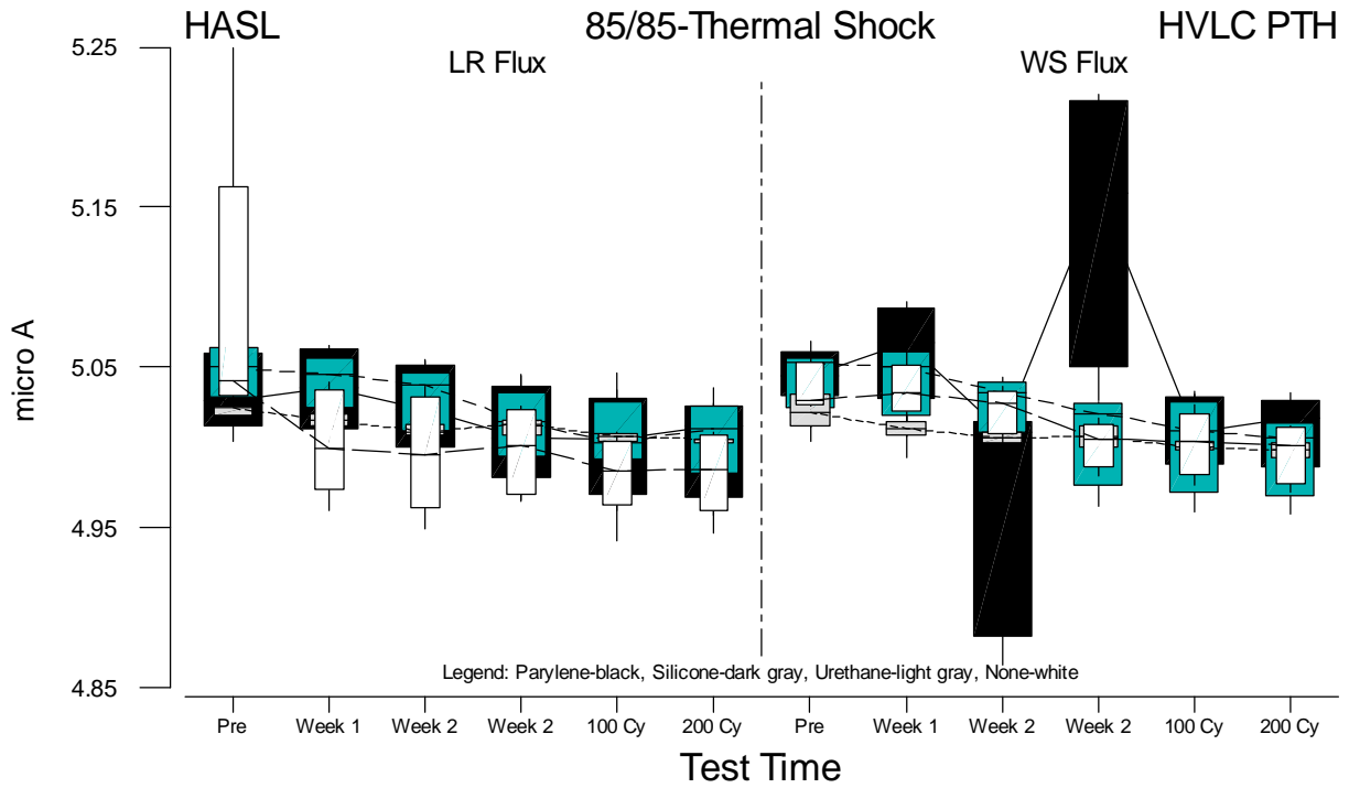
Figure F.9 Boxplots of HVLC PTH Current Measurements for HASL versus Test Time
