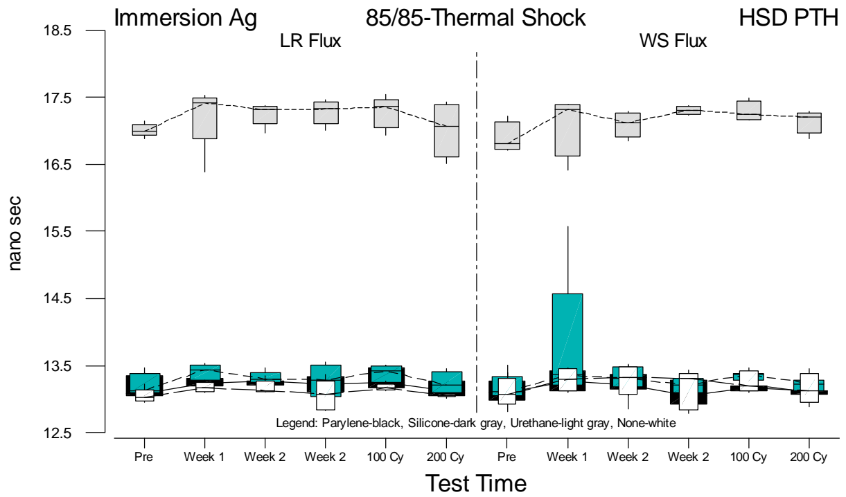
Figure F.19 Boxplots of HSD PTH Propagation Delay Measurements for Immersion Ag versus Test Time
