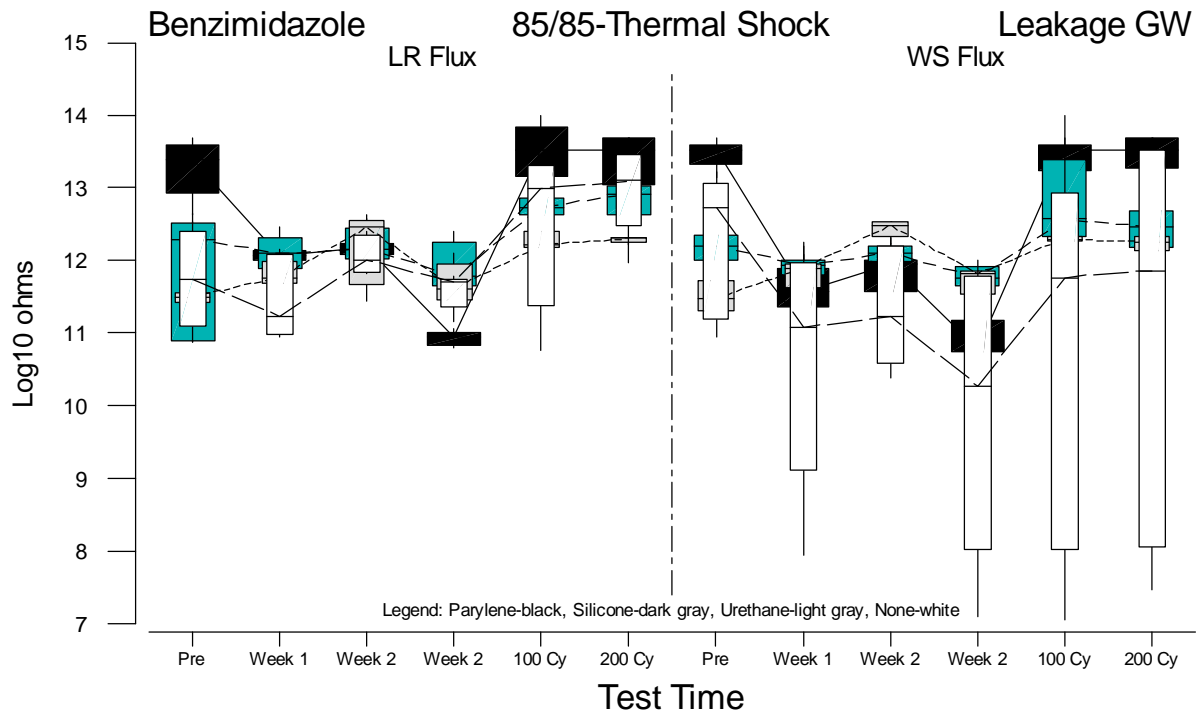
Figure F.82 Boxplots of Gull Wing Leakage Measurements for Benzimidazole versus Test Time
