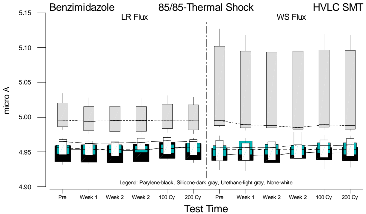
Figure F.14 Boxplots of HVLC SMT Current Measurements for Benzimidazole versus Test Time
