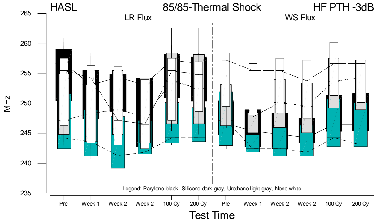
Figure F.29 Boxplots of HF PTH f(-3dB) Measurements for HASL versus Test Time
