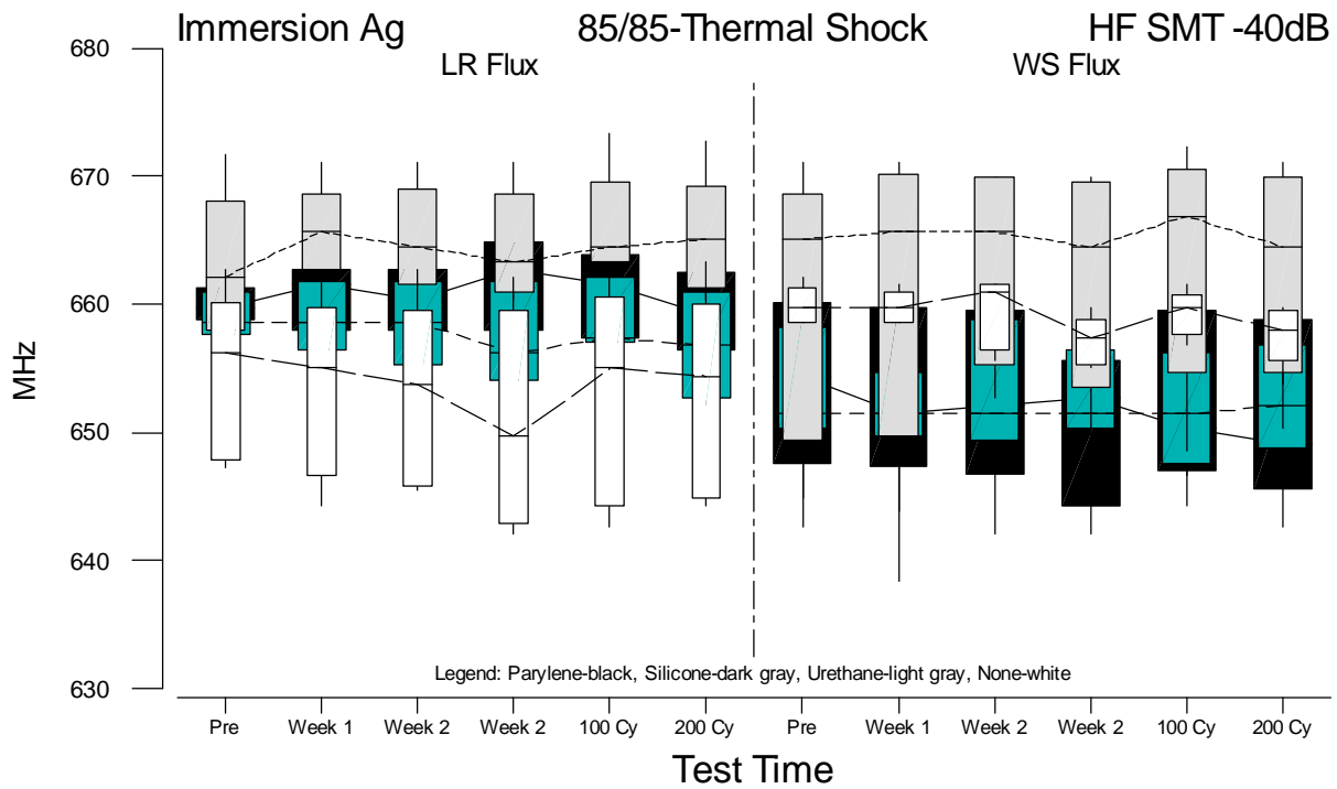
Figure F.47 Boxplots of HF SMT f(-40dB) Measurements for Immersion Ag versus Test Time
