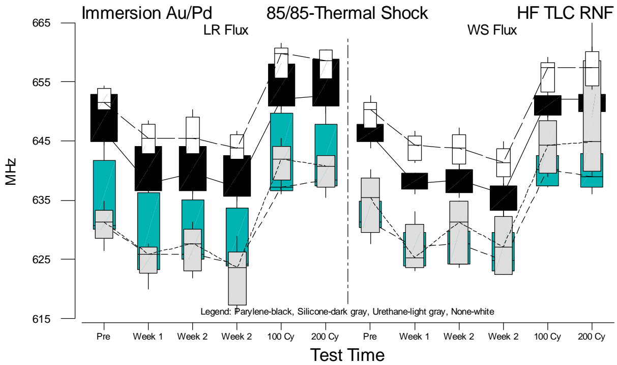
Figure F.64 Boxplots of HF TLC Rev. Null Frequency Measurements for Immersion Au/Pd vs. Test Time
