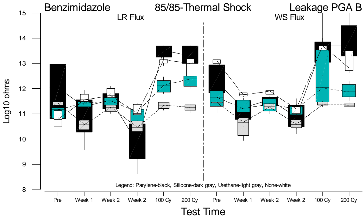
Figure F.78 Boxplots of PGA-B Leakage Measurements for Benzimidazole versus Test Time
