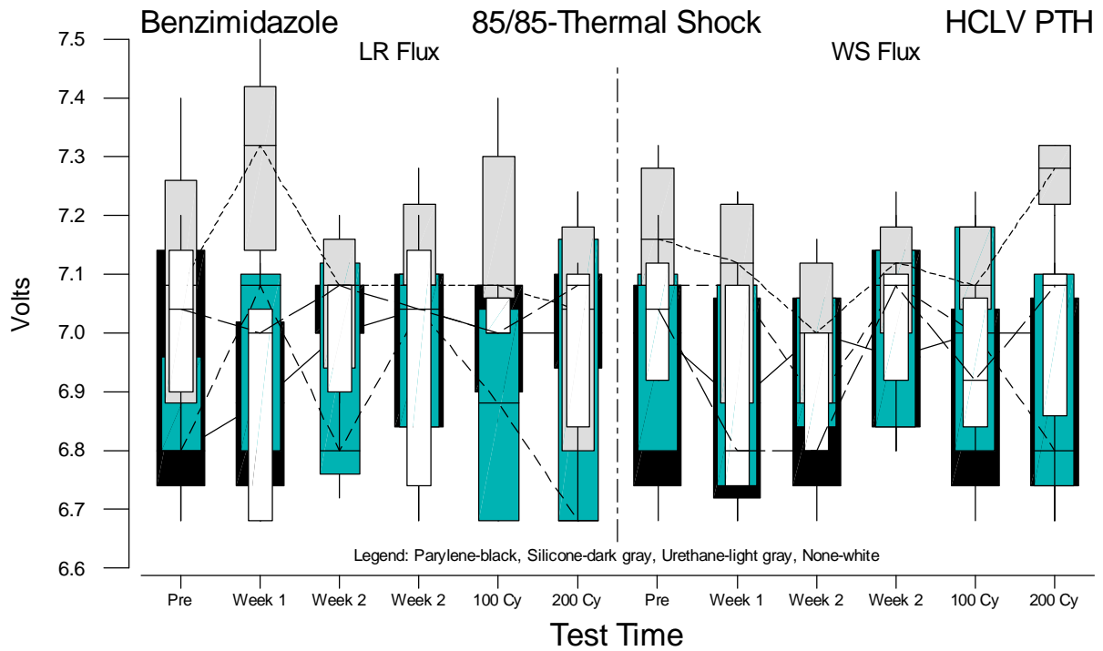
Figure F.2 Boxplots of HCLV PTH Voltage Measurements for Benzimidazole versus Test Time
