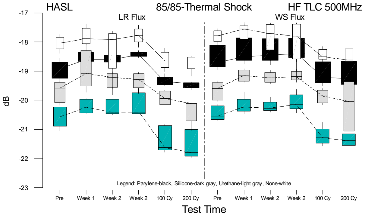
Figure F.53 Boxplots of HF TLC 500MHz Measurements for HASL versus Test Time
