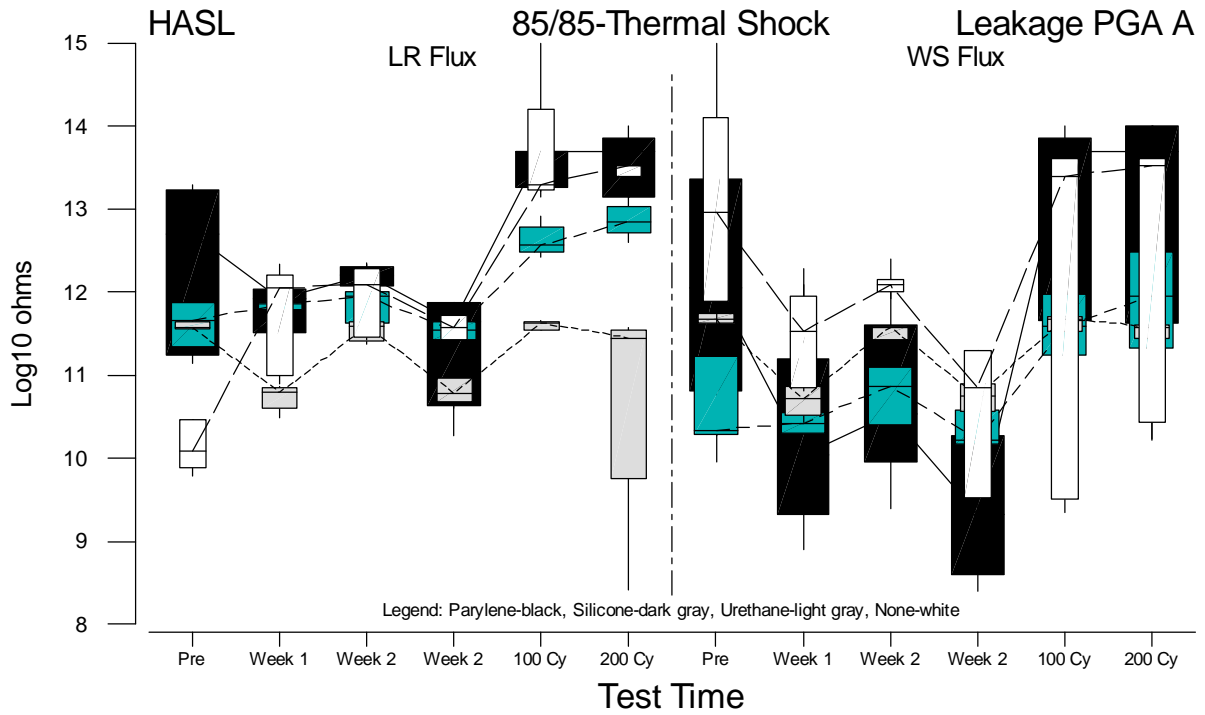
Figure F.73 Boxplots of PGA-A Leakage Measurements for HASL versus Test Time
