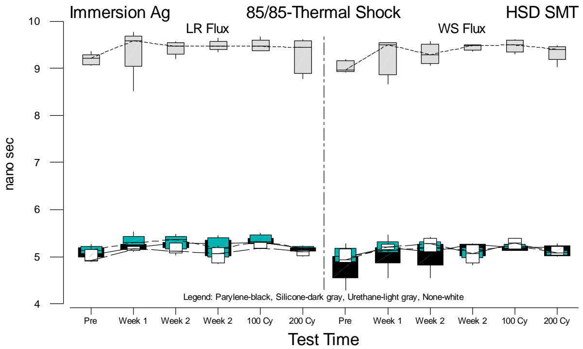
Figure F.23 Boxplots of HSD SMT Propagation Delay Measurements for Immersion Ag versus Test Time
