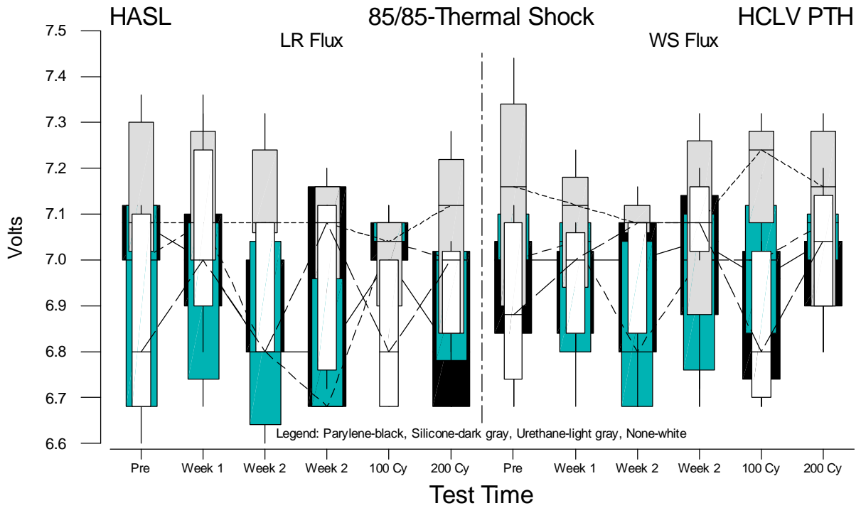
Figure F.1 Boxplots of HCLV PTH Voltage Measurements for HASL versus Test Time
