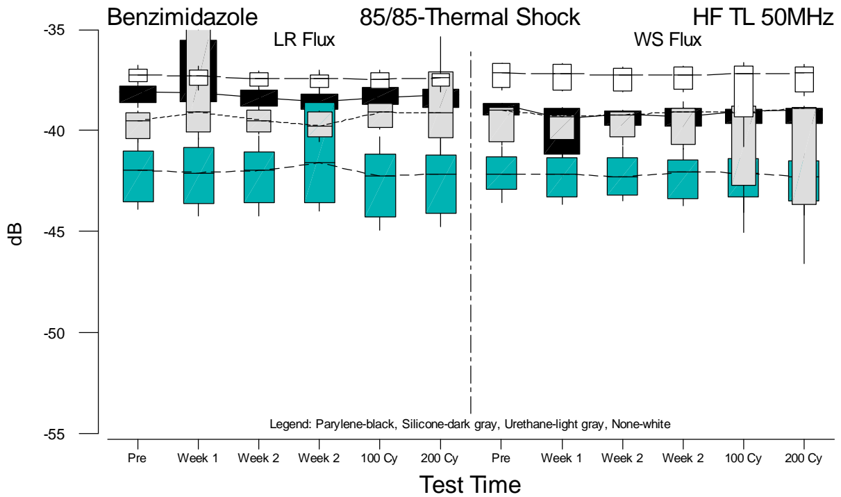
Figure F.50 Boxplots of HF TLC 50MHz Measurements for Benzimidazole versus Test Time
