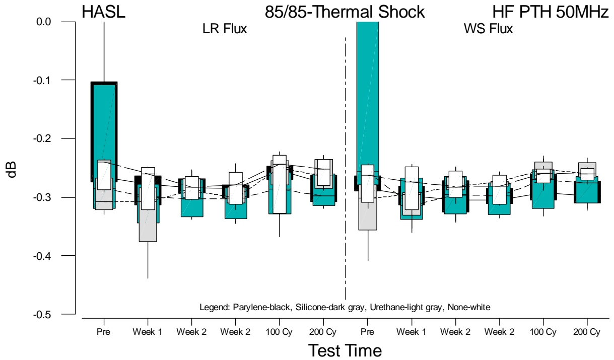
Figure F.25 Boxplots of HF PTH 50MHz Measurements for HASL versus Test Time
