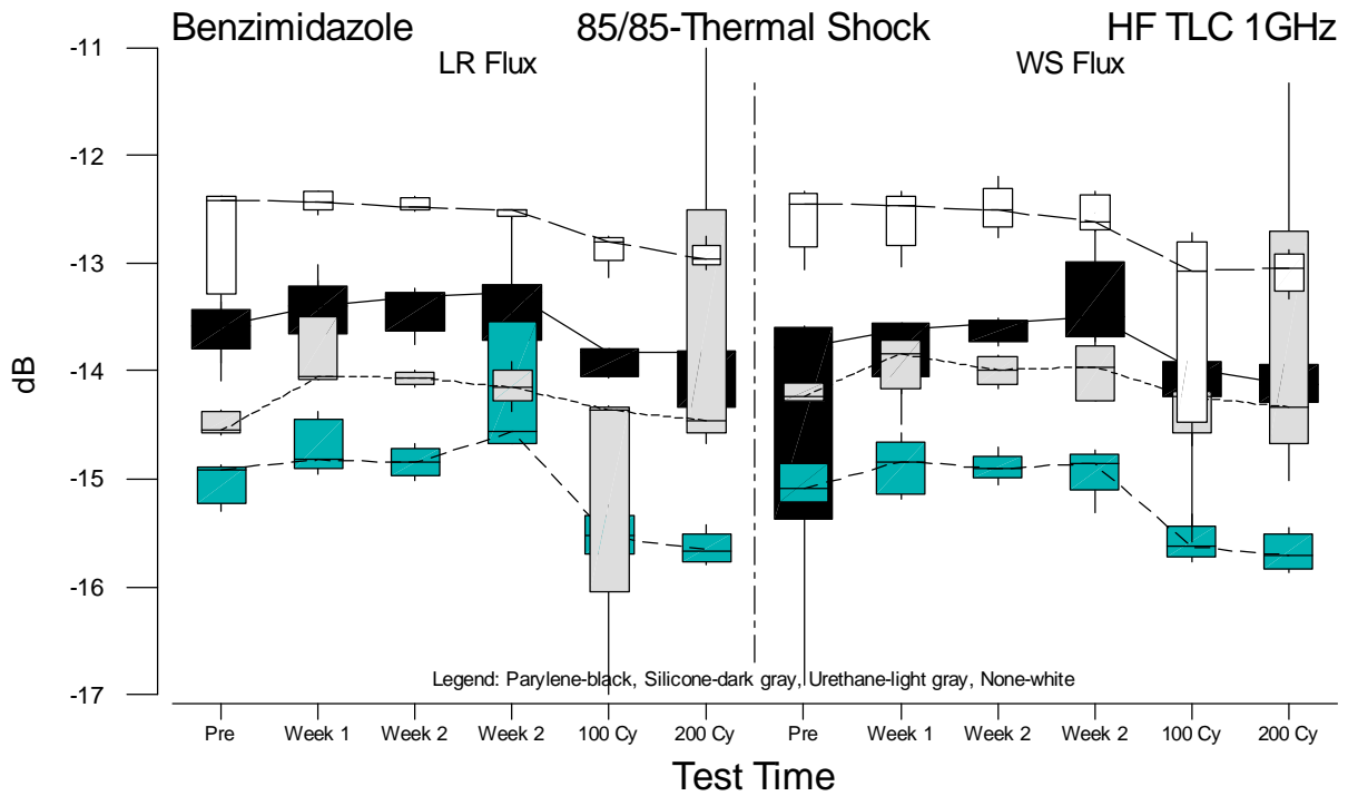
Figure F.58 Boxplots of HF TLC 1GHz Measurements for Benzimidazole versus Test Time
