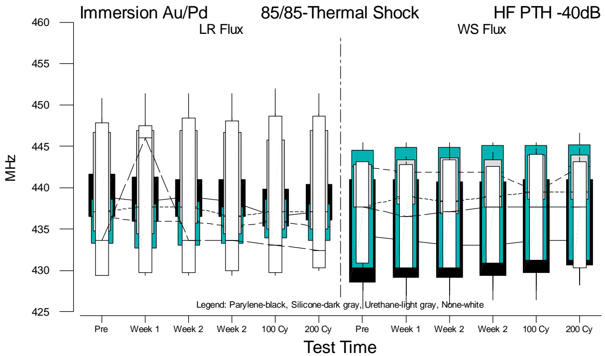
Figure F.36 Boxplots of HF PTH f(-40B) Measurements for Immersion Au/Pd versus Test Time
