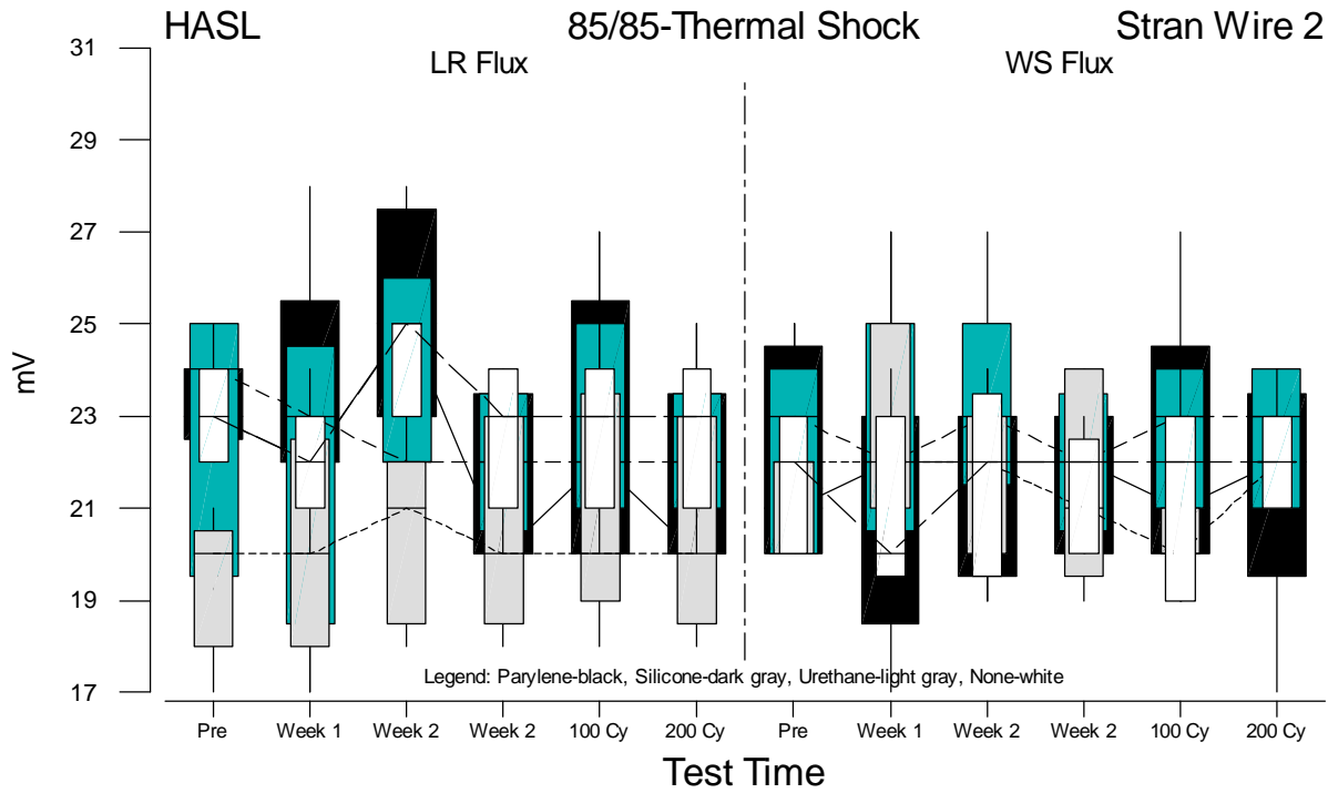
Figure F.89 Boxplots of Stranded Wire 2 Voltage Measurements for HASL versus Test Time
