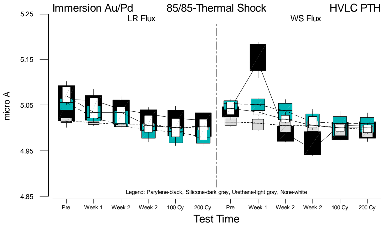
Figure F.12 Boxplots of HVLC PTH Current Measurements for Immersion Au/Pd versus Test Time
