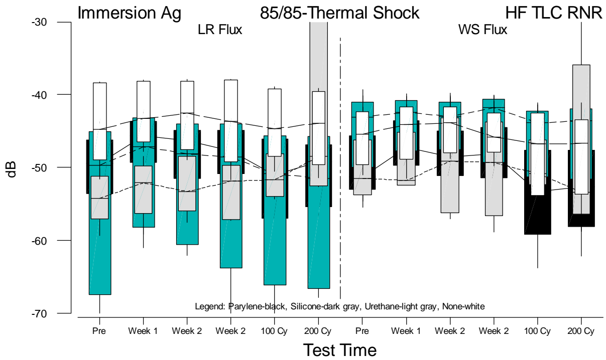
Figure F.67 Boxplots of HF TLC Rev. Null Response Measurements for Immersion Ag versus Test Time
