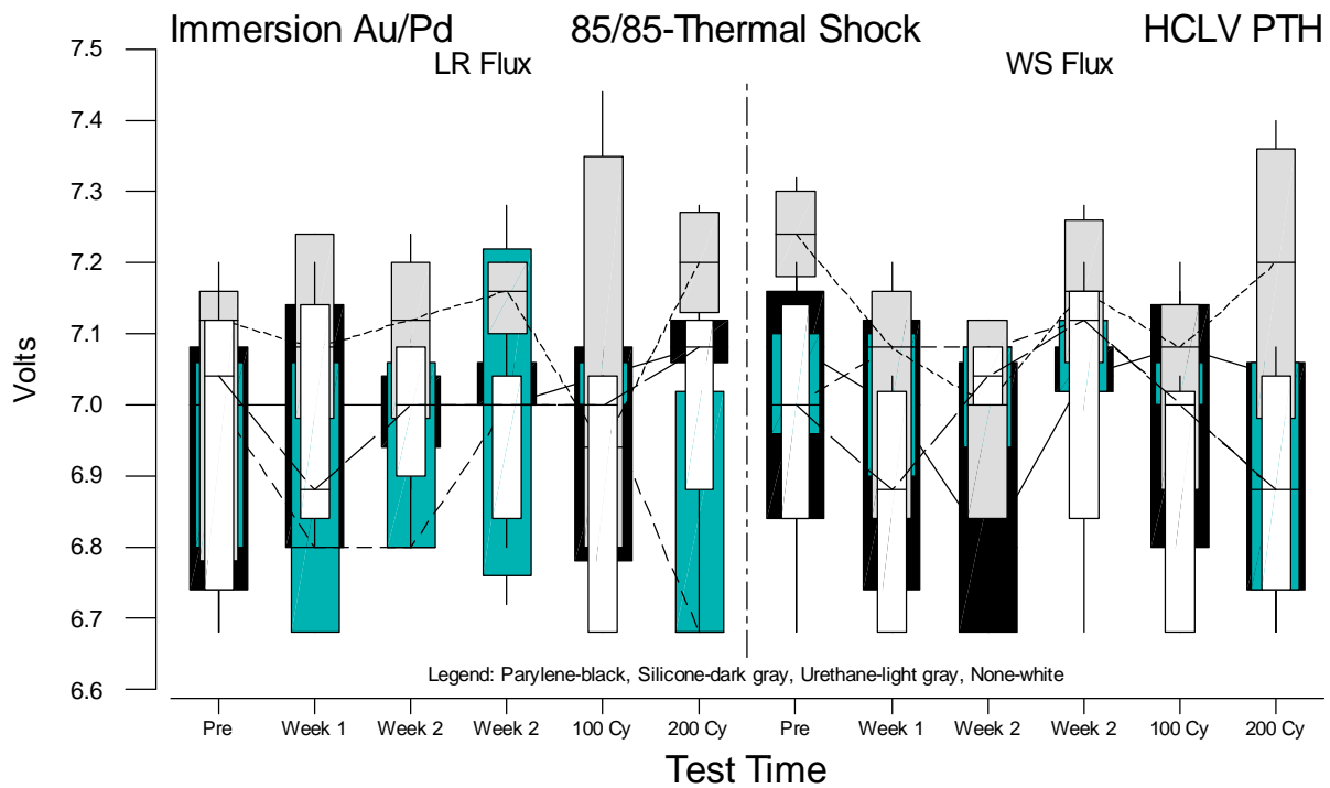
Figure F.4 Boxplots of HCLV PTH Voltage Measurements for Immersion Au/Pd versus Test Time
