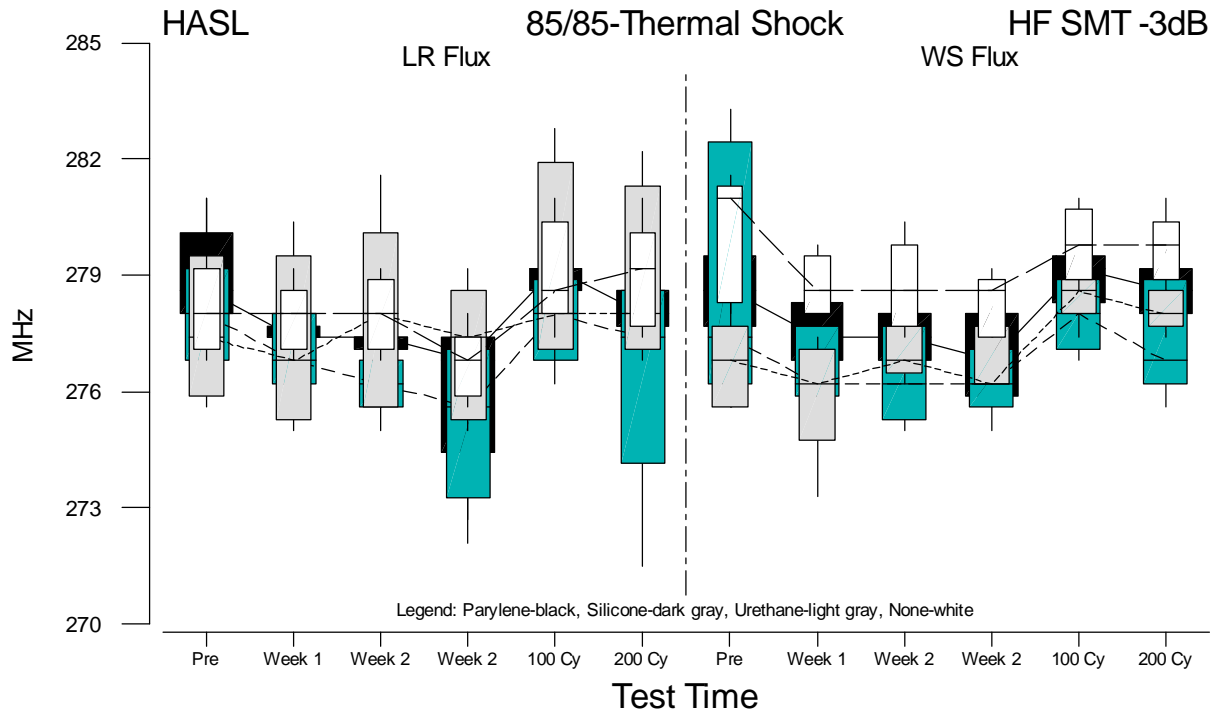
Figure F.41 Boxplots of HF SMT f(-3dB) Measurements for HASL versus Test Time
