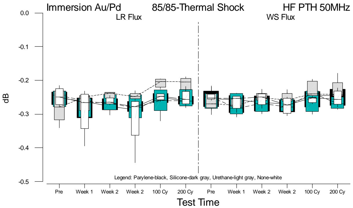
Figure F.28 Boxplots of HF PTH 50MHz Measurements for Immersion Au/Pd versus Test Time
