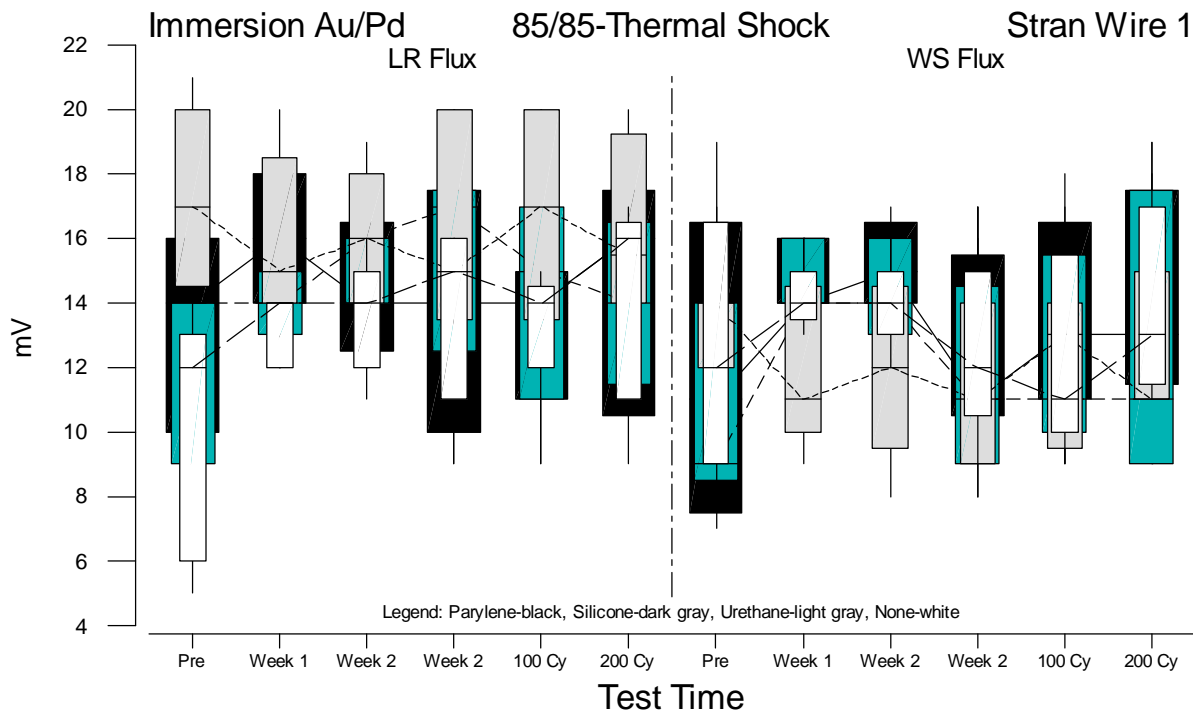
Figure F.88 Boxplots of Stranded Wire 1 Voltage Measurements for Immersion Au/Pd versus Test Time
