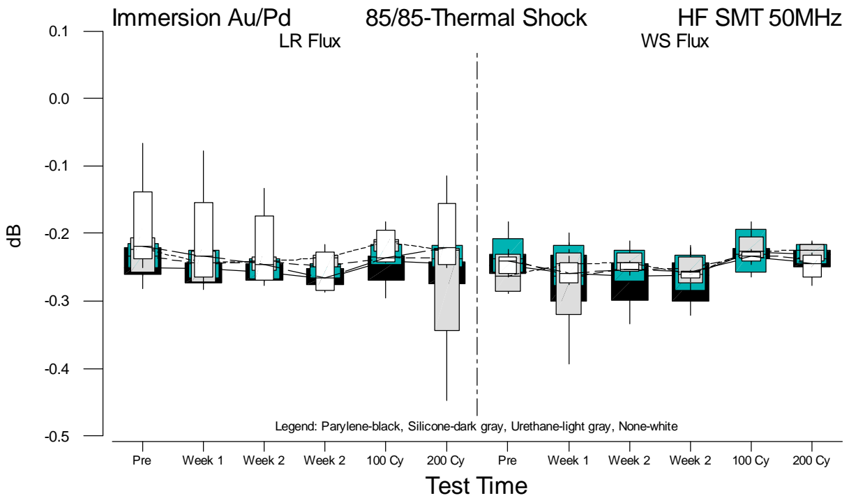
Figure F.40 Boxplots of HF SMT 50MHz Measurements for Immersion Au/Pd versus Test Time
