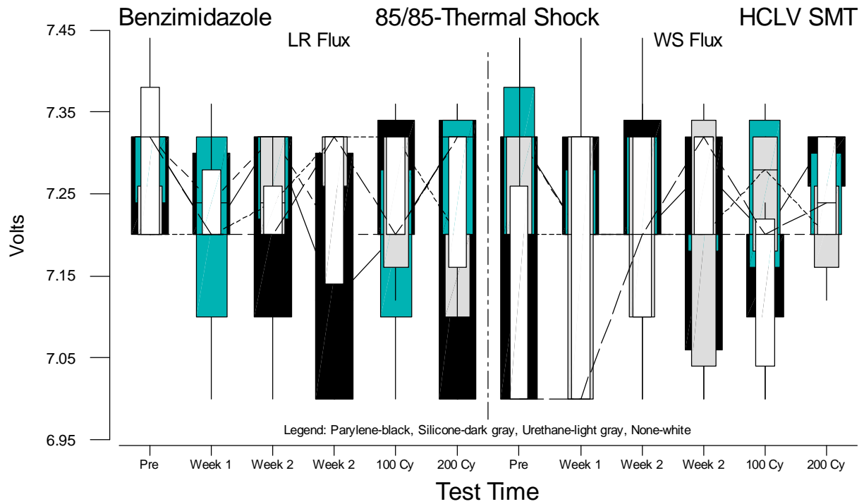
Figure F.6 Boxplots of HCLV SMT Voltage Measurements for Benzimidazole versus Test Time
