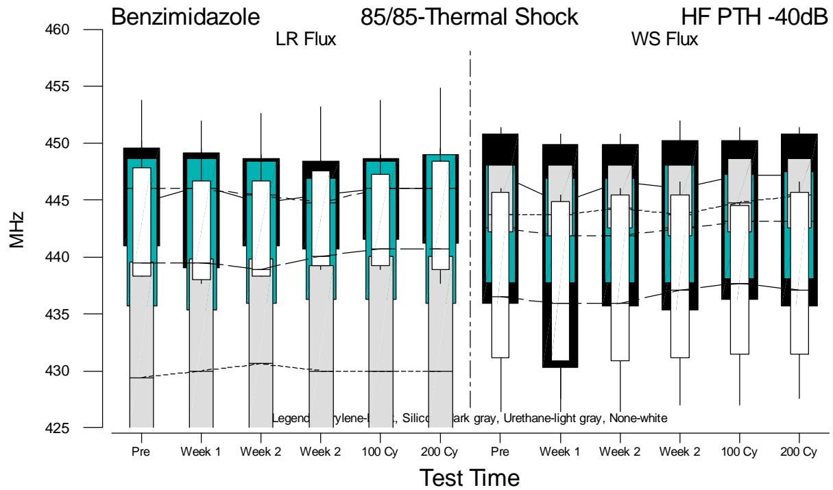
Figure F.34 Boxplots of HF PTH f(-40B) Measurements for Benzimidazole versus Test Time
