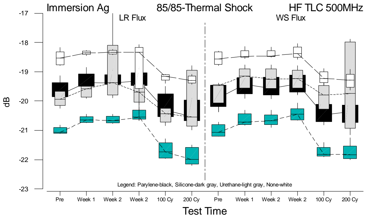
Figure F.55 Boxplots of HF TLC 500MHz Measurements for Immersion Ag versus Test Time
