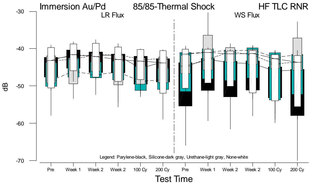
Figure F.68 Boxplots of HF TLC Rev. Null Response Measurements for Immersion Au/Pd vs. Test Time
