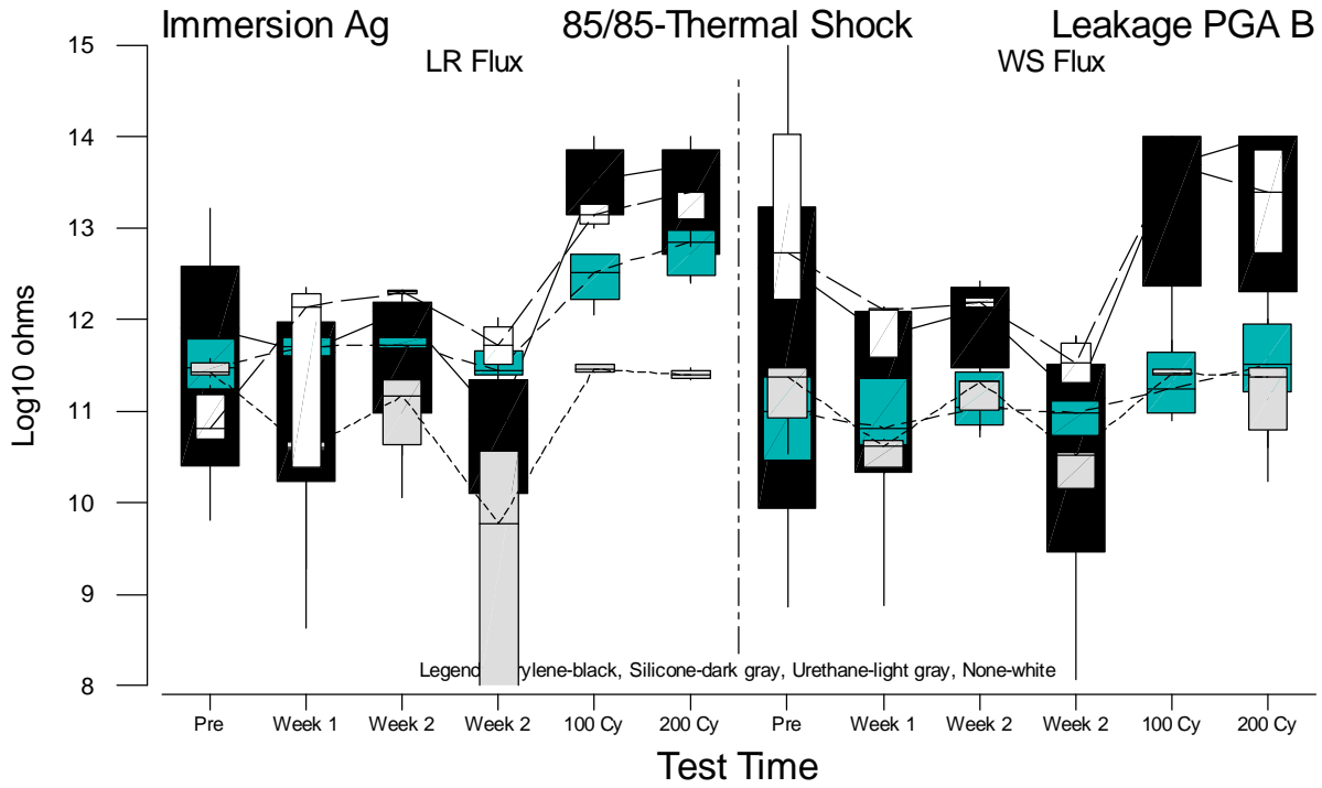
Figure F.79 Boxplots of PGA-B Leakage Measurements for Immersion Ag versus Test Time
