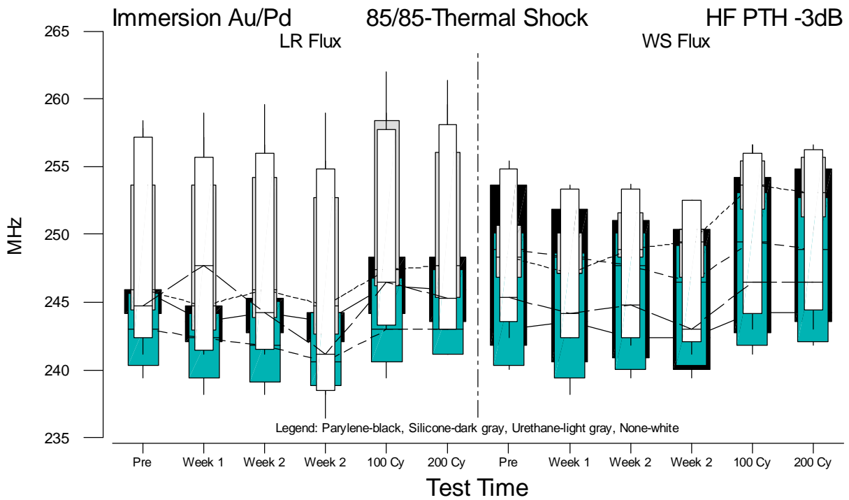
Figure F.32 Boxplots of HF PTH f(-3dB) Measurements for Immersion Au/Pd versus Test Time
