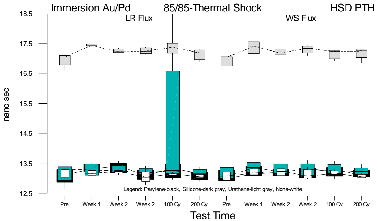
Figure F.20 Boxplots of HSD PTH Propagation Delay Measurements for Immersion Au/Pd vs. Test Time
