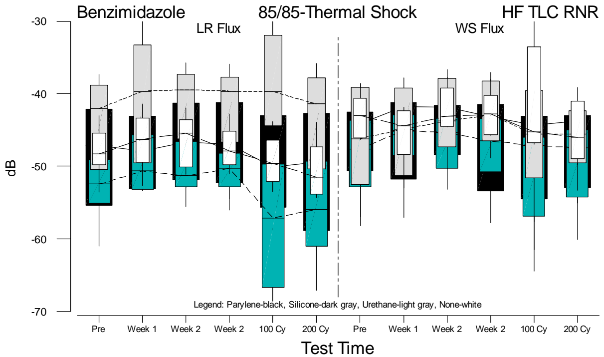
Figure F.66 Boxplots of HF TLC Rev. Null Response Measurements for Benzimidazole versus Test Time
