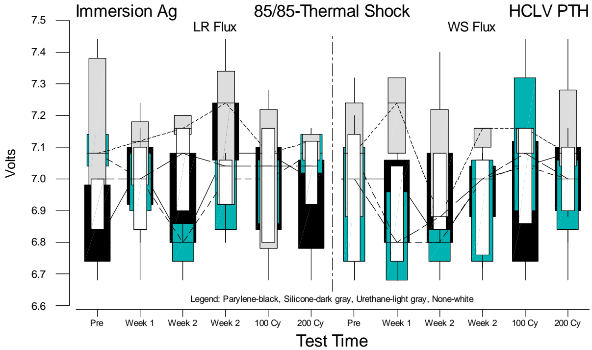
Figure F.3 Boxplots of HCLV PTH Voltage Measurements for Immersion Ag versus Test Time
