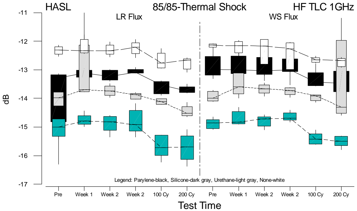
Figure F.57 Boxplots of HF TLC 1GHz Measurements for HASL versus Test Time
