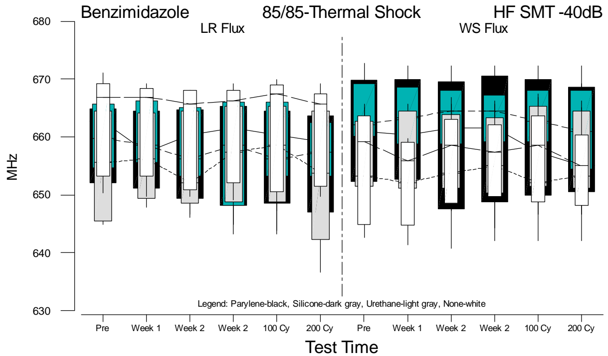
Figure F.46 Boxplots of HF SMT f(-40dB) Measurements for Benzimidazole versus Test Time
