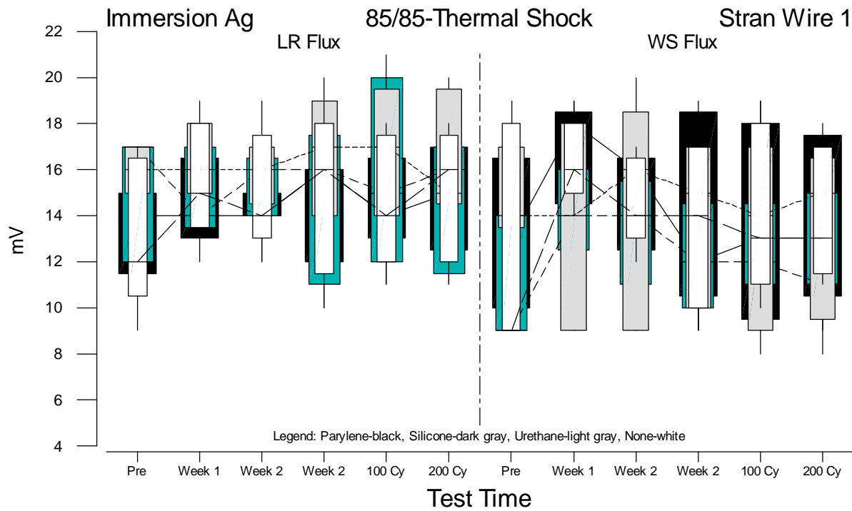
Figure F.87 Boxplots of Stranded Wire 1 Voltage Measurements for Immersion Ag versus Test Time
