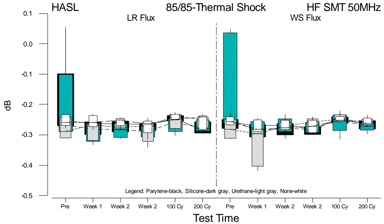
Figure F.37 Boxplots of HF SMT 50MHz Measurements for HASL versus Test Time
