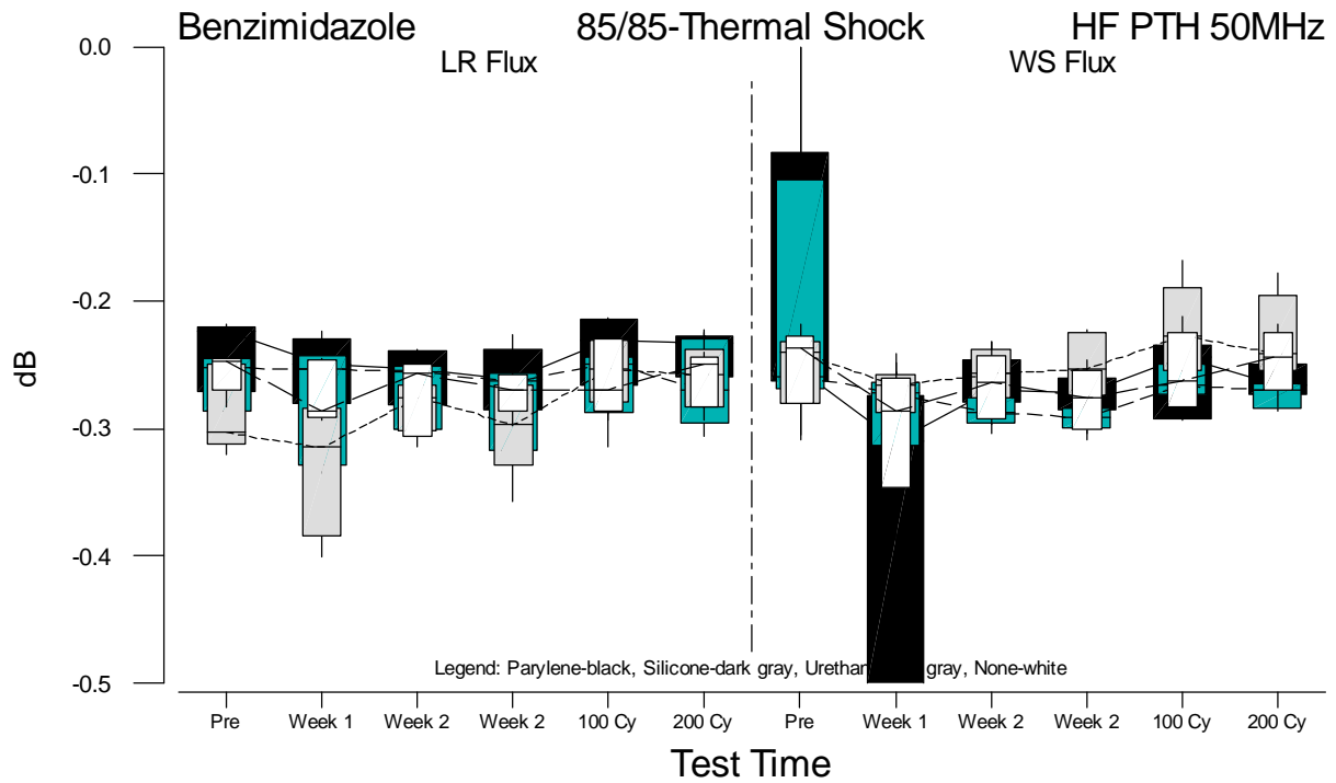
Figure F.26 Boxplots of HF PTH 50MHz Measurements for Benzimidazole versus Test Time
