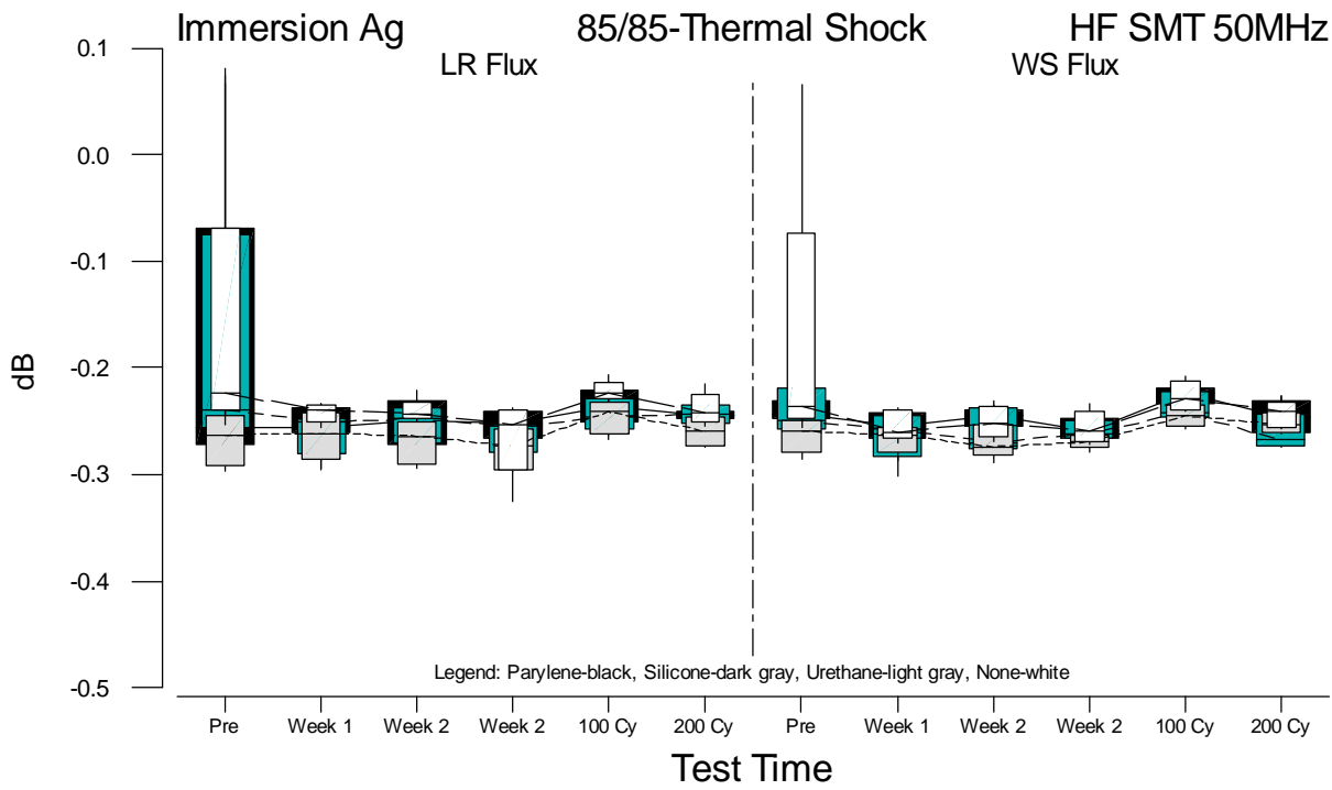
Figure F.39 Boxplots of HF SMT 50MHz Measurements for Immersion Ag versus Test Time
