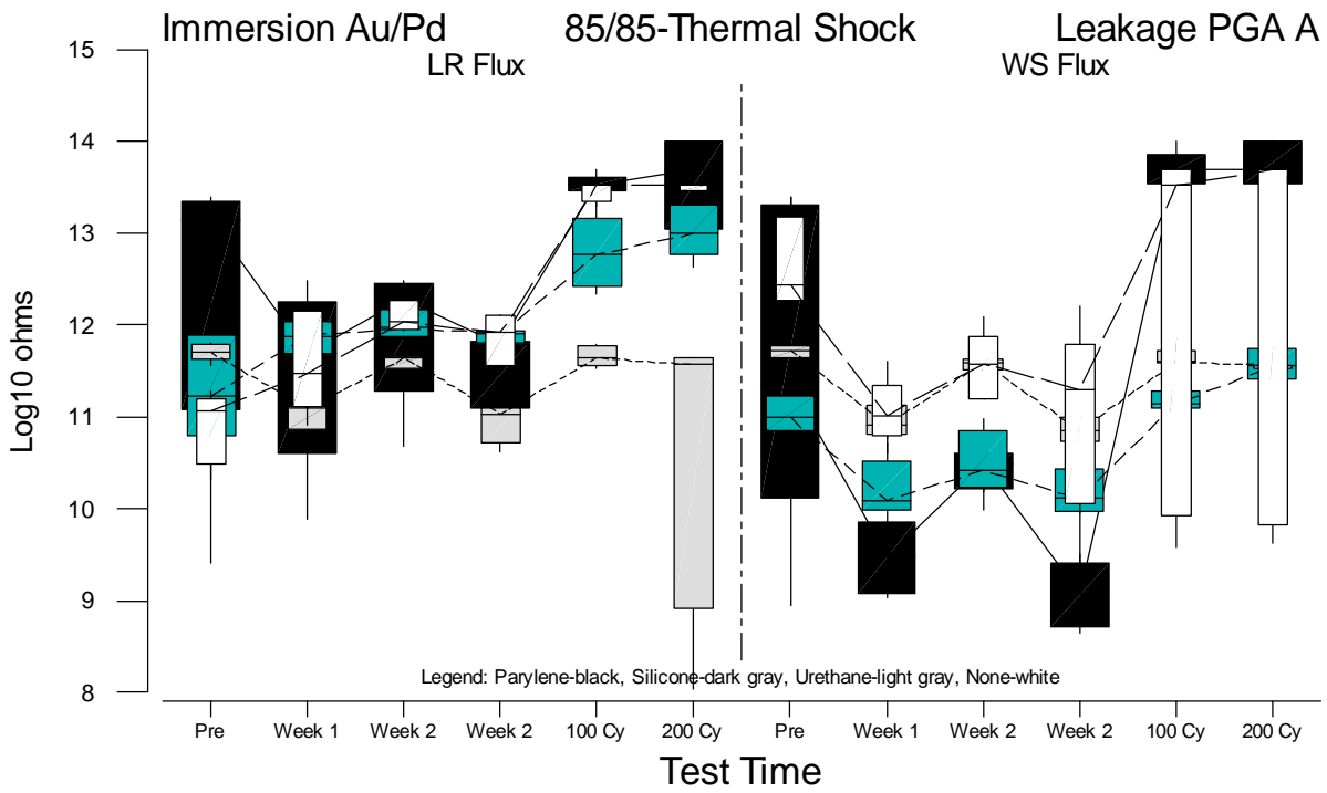
Figure F.76 Boxplots of PGA-A Leakage Measurements for Immersion Au/Pd vs. Test Time
