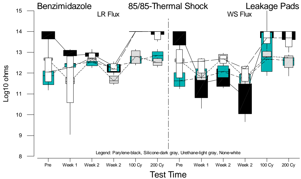
Figure F.70 Boxplots of 10-Mil Leakage Measurements for Benzimidazole versus Test Time
