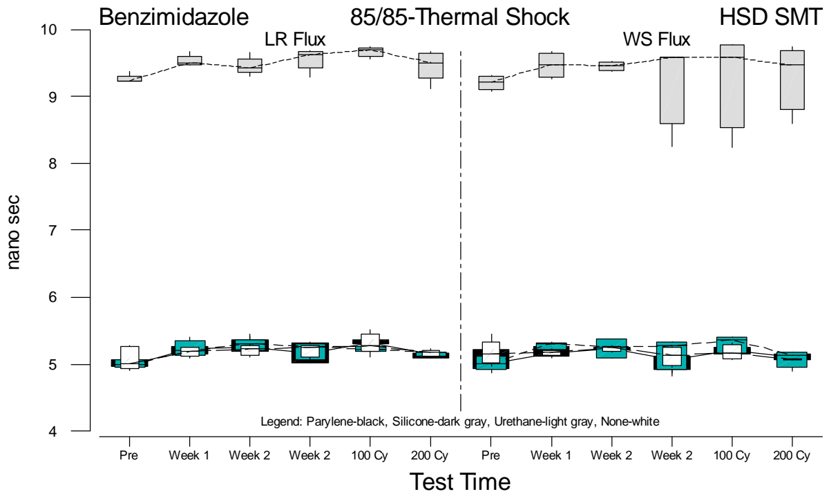
Figure F.22 Boxplots of HSD SMT Propagation Delay Measurements for Benzimidazole versus Test Time
