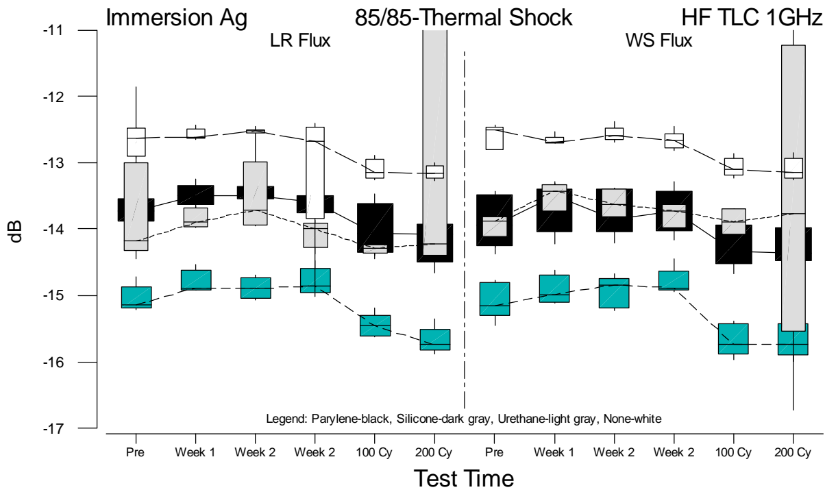
Figure F.59 Boxplots of HF TLC 1GHz Measurements for Immersion Ag versus Test Time
