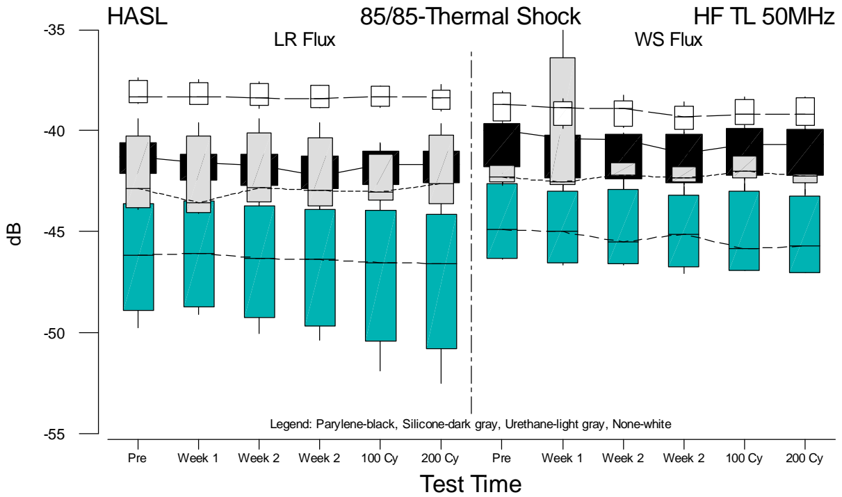
Figure F.49 Boxplots of HF TLC 50MHz Measurements for HASL versus Test Time
