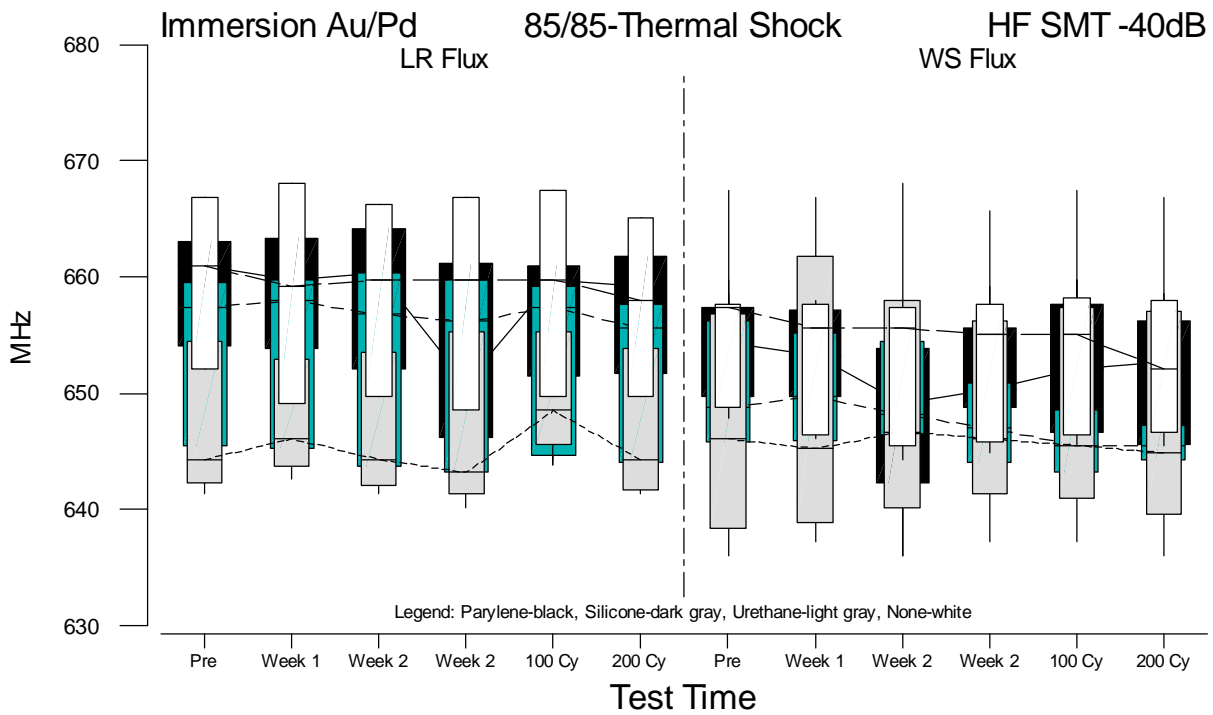
Figure F.48 Boxplots of HF SMT f(-40dB) Measurements for Immersion Au/Pd versus Test Time
