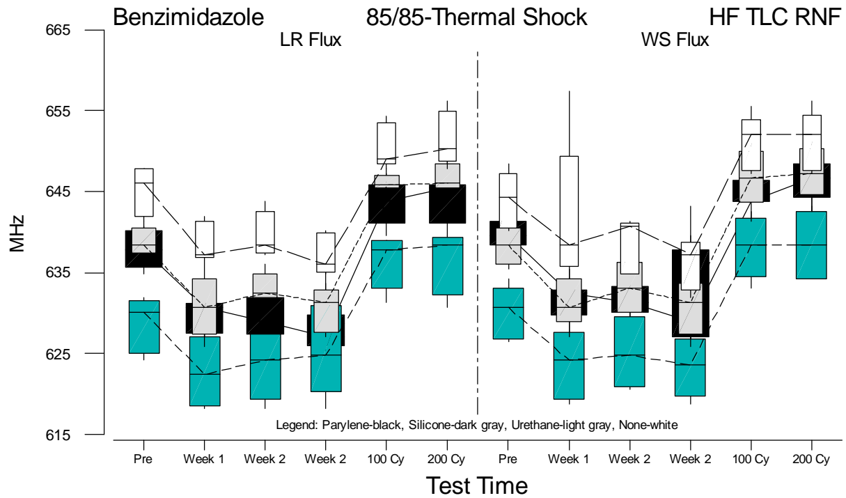
Figure F.62 Boxplots of HF TLC Rev. Null Frequency Measurements for Benzimidazole vs. Test Time
