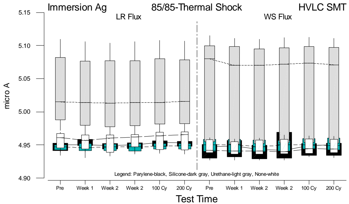
Figure F.15 Boxplots of HVLC SMT Current Voltage Measurements for Immersion Ag versus Test Time
