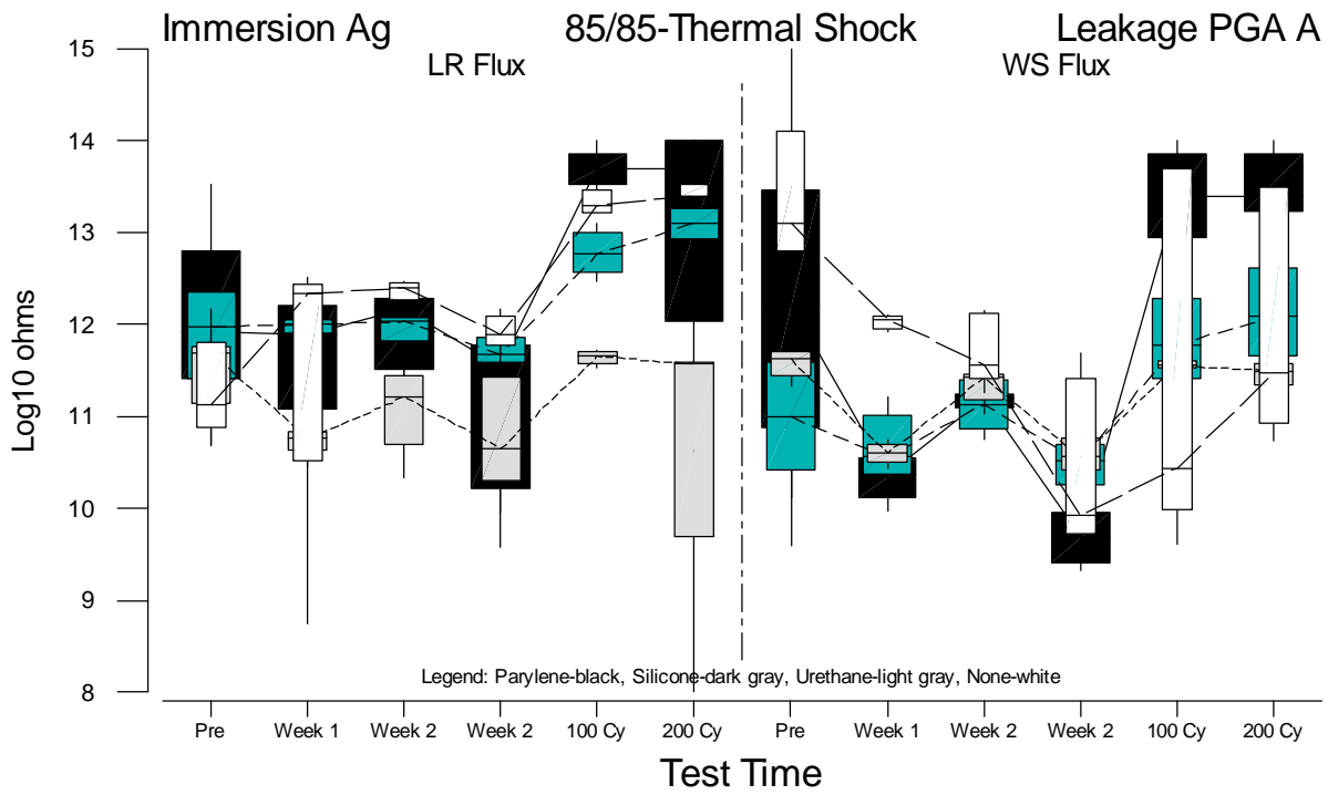
Figure F.75 Boxplots of PGA-A Leakage Measurements for Immersion Ag versus Test Time
