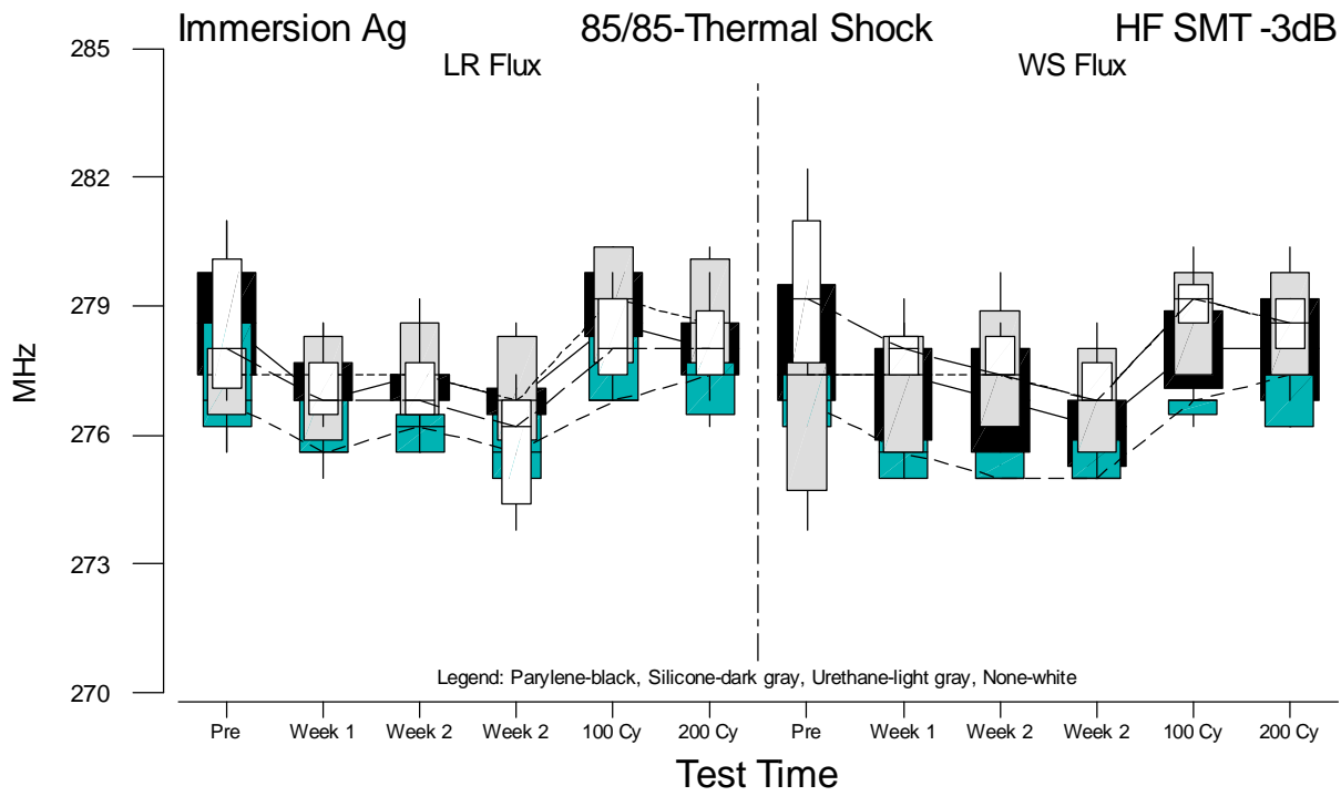
Figure F.43 Boxplots of HF SMT f(-3dB) Measurements for Immersion Ag versus Test Time
