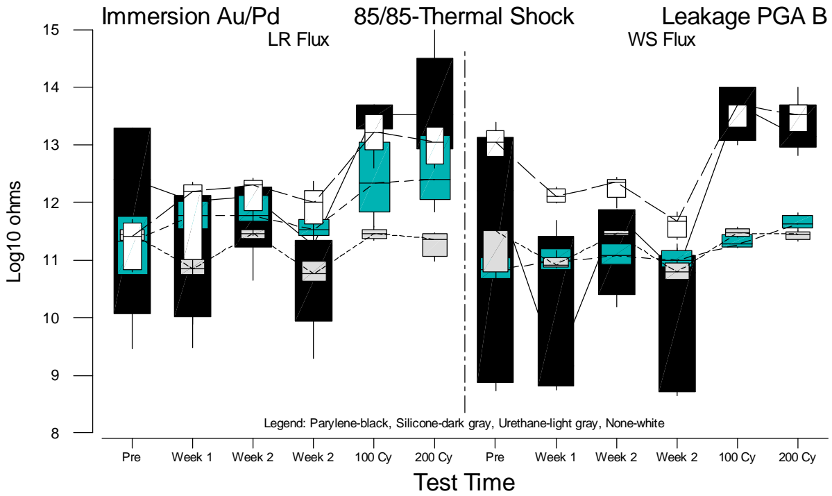
Figure F.80 Boxplots of PGA-B Leakage Measurements for Immersion Au/Pd versus Test Time
