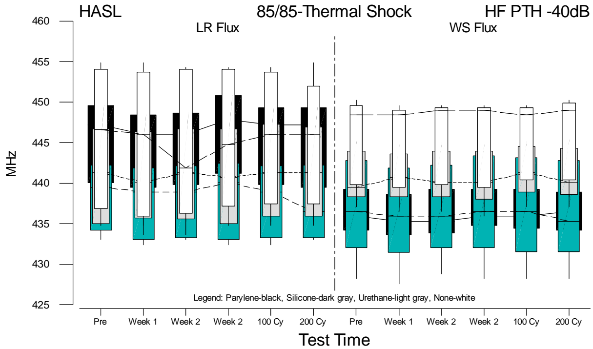
Figure F.33 Boxplots of HF PTH f(-40B) Measurements for HASL versus Test Time
