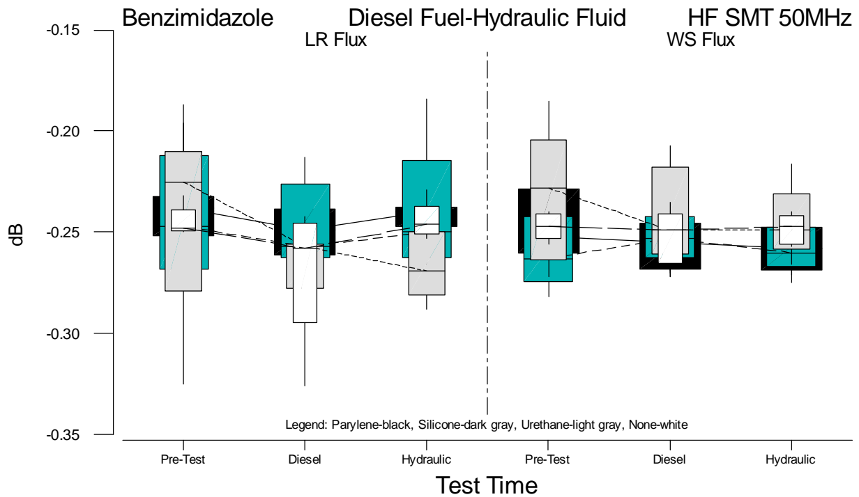
Figure B.38 Boxplots of HF SMT 50MHz Measurements for Benzimidazole versus Test Time
