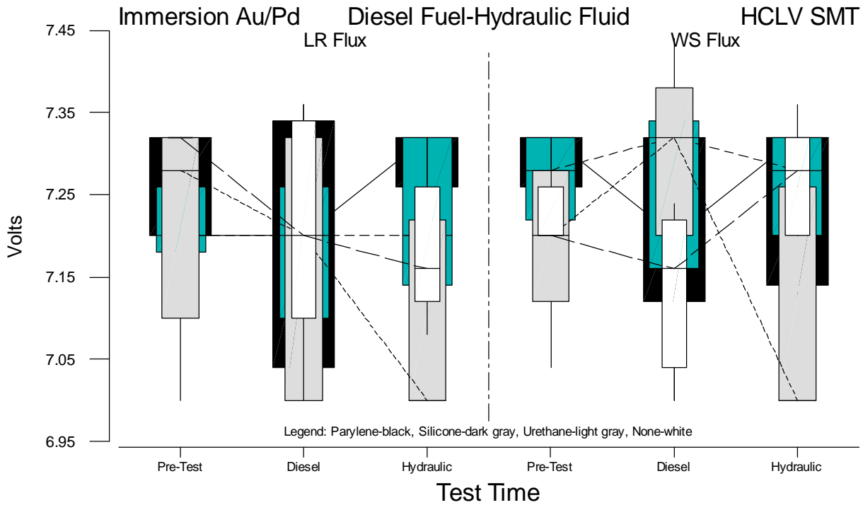
Figure B.8 Boxplots of HCLV SMT Voltage Measurements for Immersion Au/Pd versus Test Time
