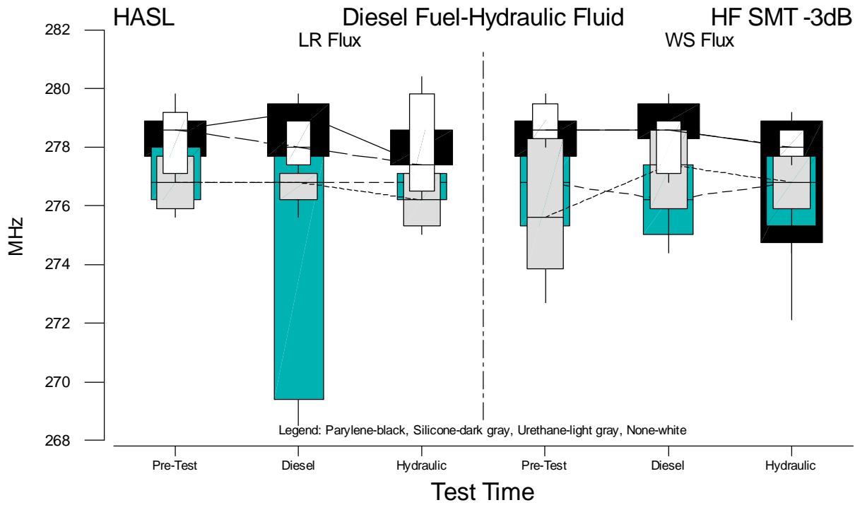
Figure B.41 Boxplots of HF SMT f(-3dB) Measurements for HASL versus Test Time
