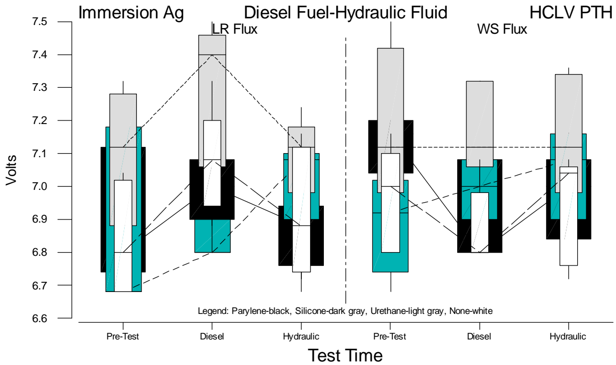
Figure B.3 Boxplots of HCLV PTH Voltage Measurements for Immersion Ag versus Test Time
