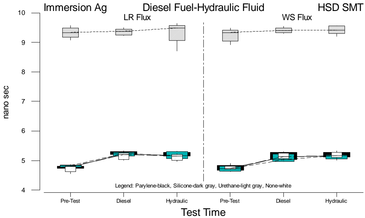
Figure B.23 Boxplots of HSD SMT Propagation Delay Measurements for Immersion Ag versus Test Time
