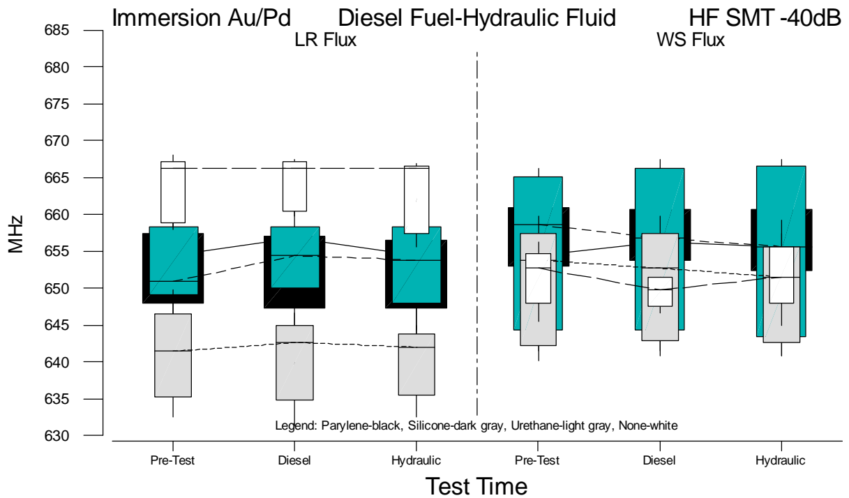
Figure B.48 Boxplots of HF SMT f(-40dB) Measurements for Immersion Au/Pd versus Test Time
