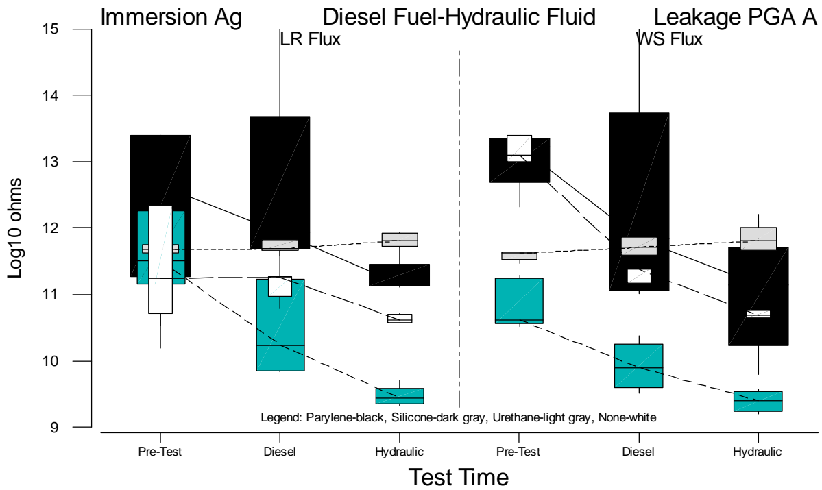
Figure B.75 Boxplots of PGA-A Leakage Measurements for Immersion Ag versus Test Time
