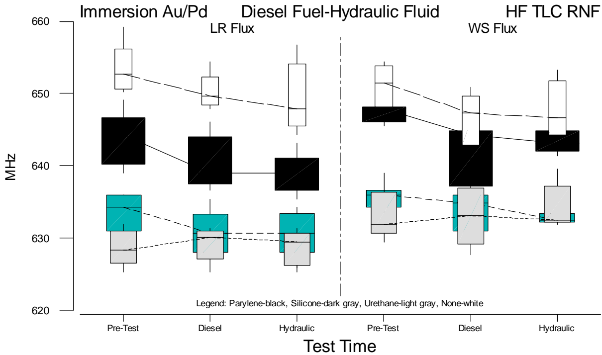
Figure B.64 Boxplots of HF TLC Rev. Null Frequency Measurements for Immersion Au/Pd vs. Test Time
