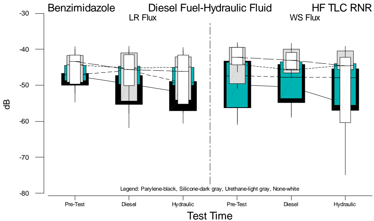
Figure B.66 Boxplots of HF TLC Rev. Null Response Measurements for Benzimidazole versus Test Time
