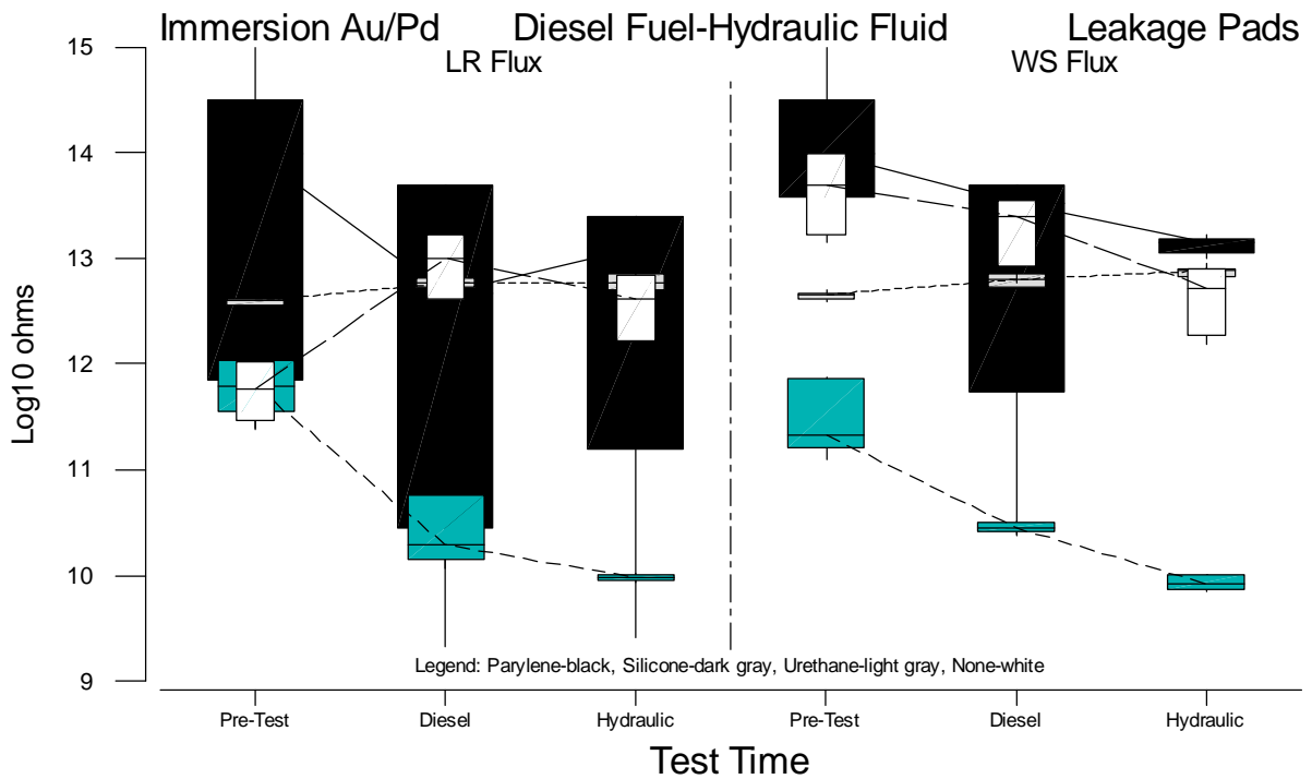
Figure B.72 Boxplots of 10-Mil Leakage Measurements for Immersion Au/Pd versus Test Time
