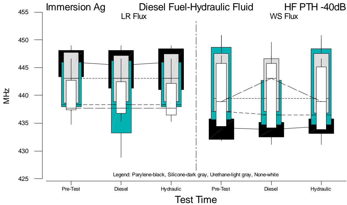
Figure B.35 Boxplots of HF PTH f(-40B) Measurements for Immersion Ag versus Test Time
