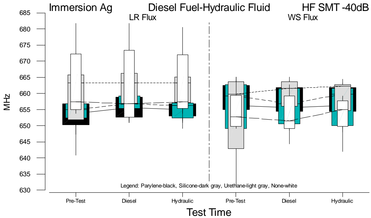
Figure B.47 Boxplots of HF SMT f(-40dB) Measurements for Immersion Ag versus Test Time
