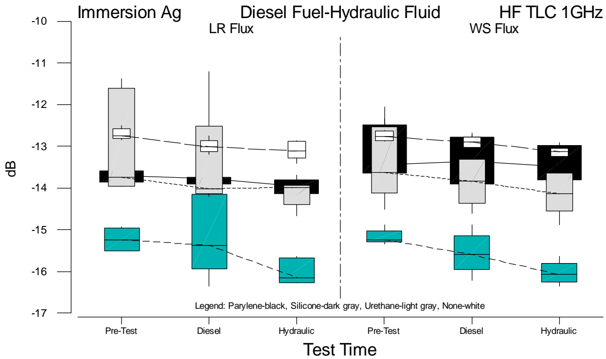
Figure B.59 Boxplots of HF TLC 1GHz Measurements for Immersion Ag versus Test Time
