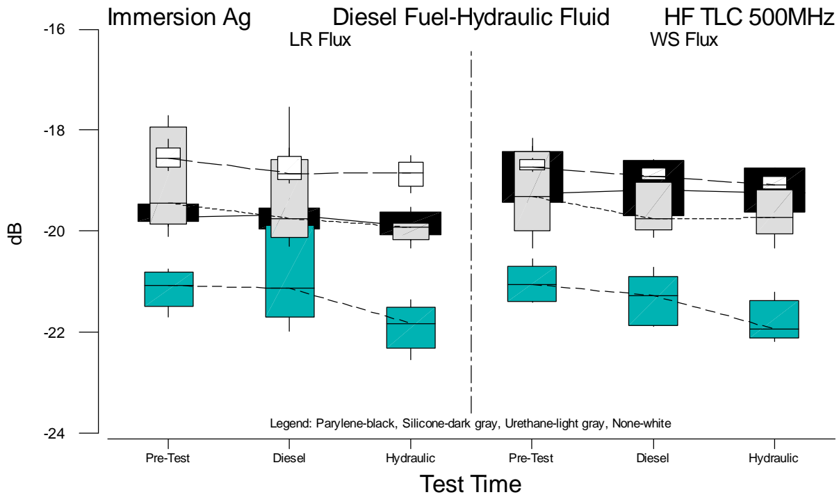
Figure B.55 Boxplots of HF TLC 500MHz Measurements for Immersion Ag versus Test Time
