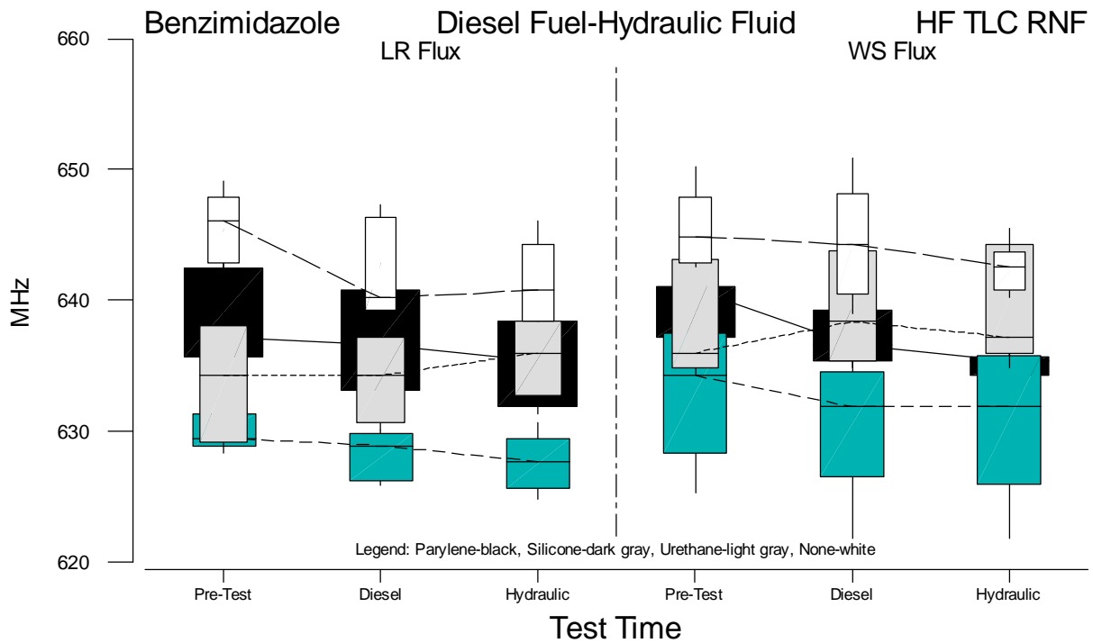
Figure B.62 Boxplots of HF TLC Rev. Null Frequency Measurements for Benzimidazole vs. Test Time
