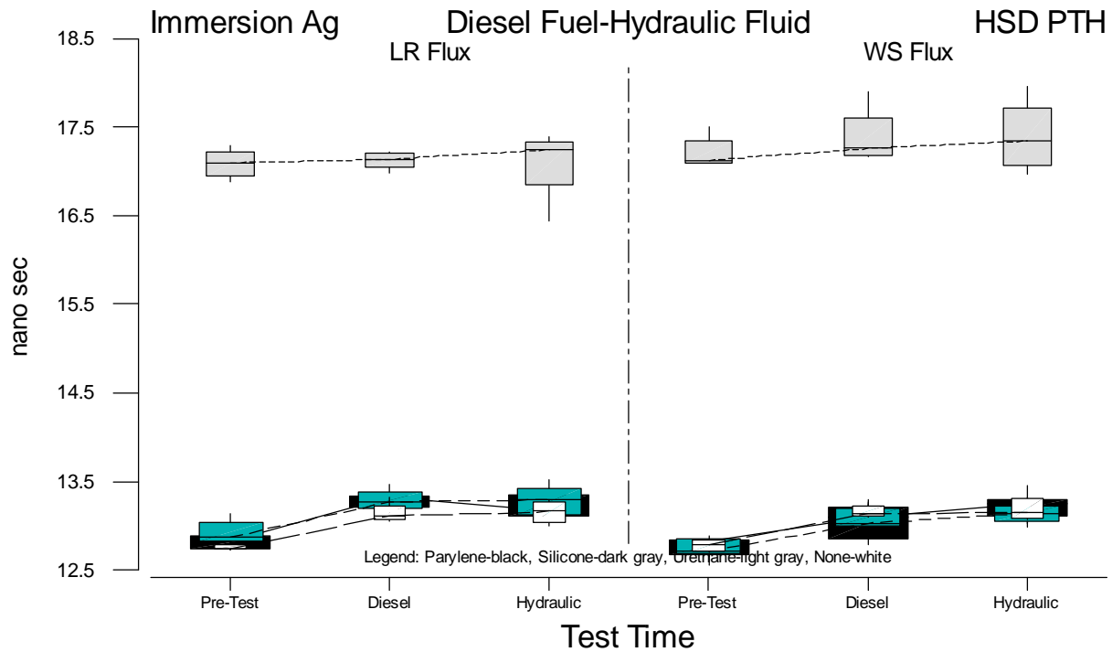
Figure B.19 Boxplots of HSD PTH Propagation Delay Measurements for Immersion Ag versus Test Time
