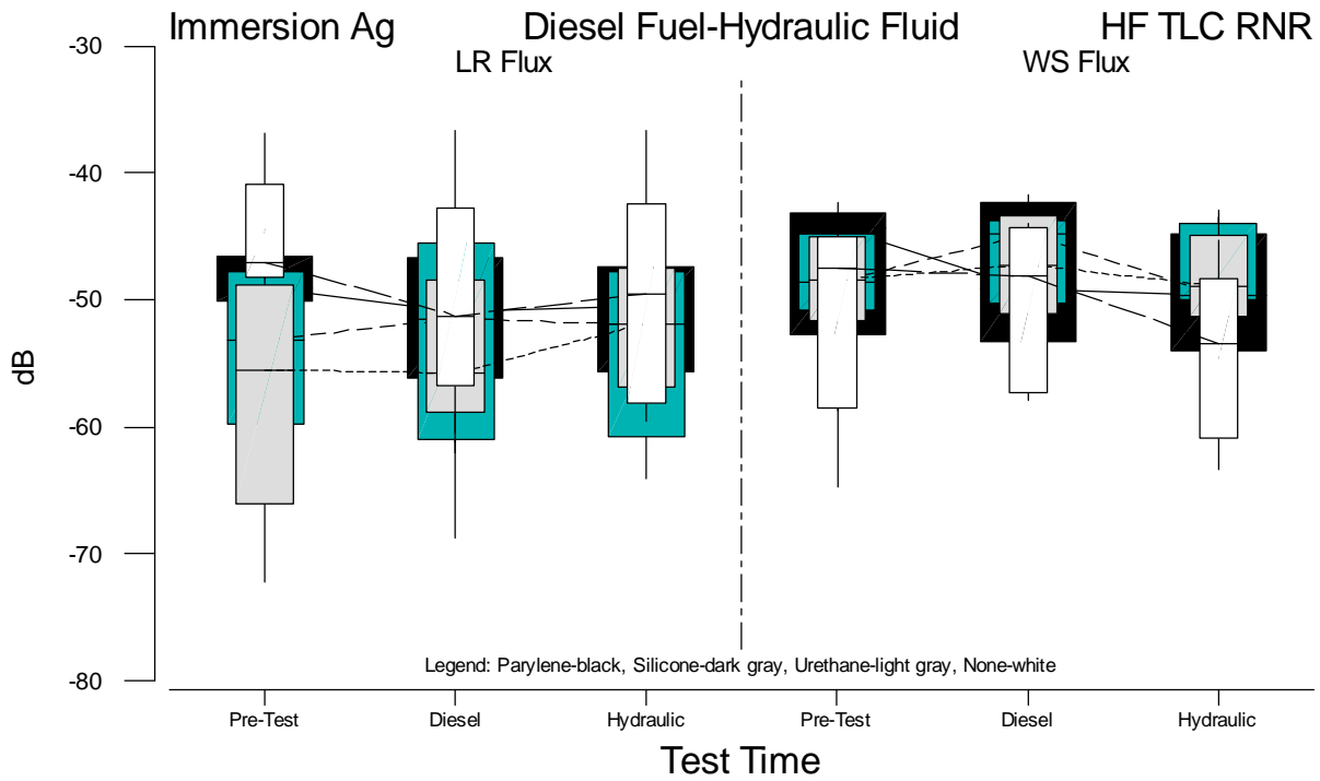
Figure B.67 Boxplots of HF TLC Rev. Null Response Measurements for Immersion Ag versus Test Time
