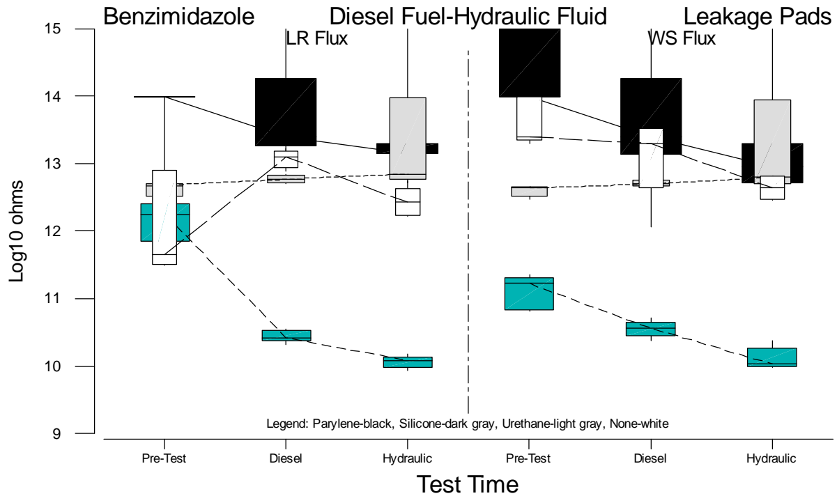
Figure B.70 Boxplots of 10-Mil Leakage Measurements for Benzimidazole versus Test Time
