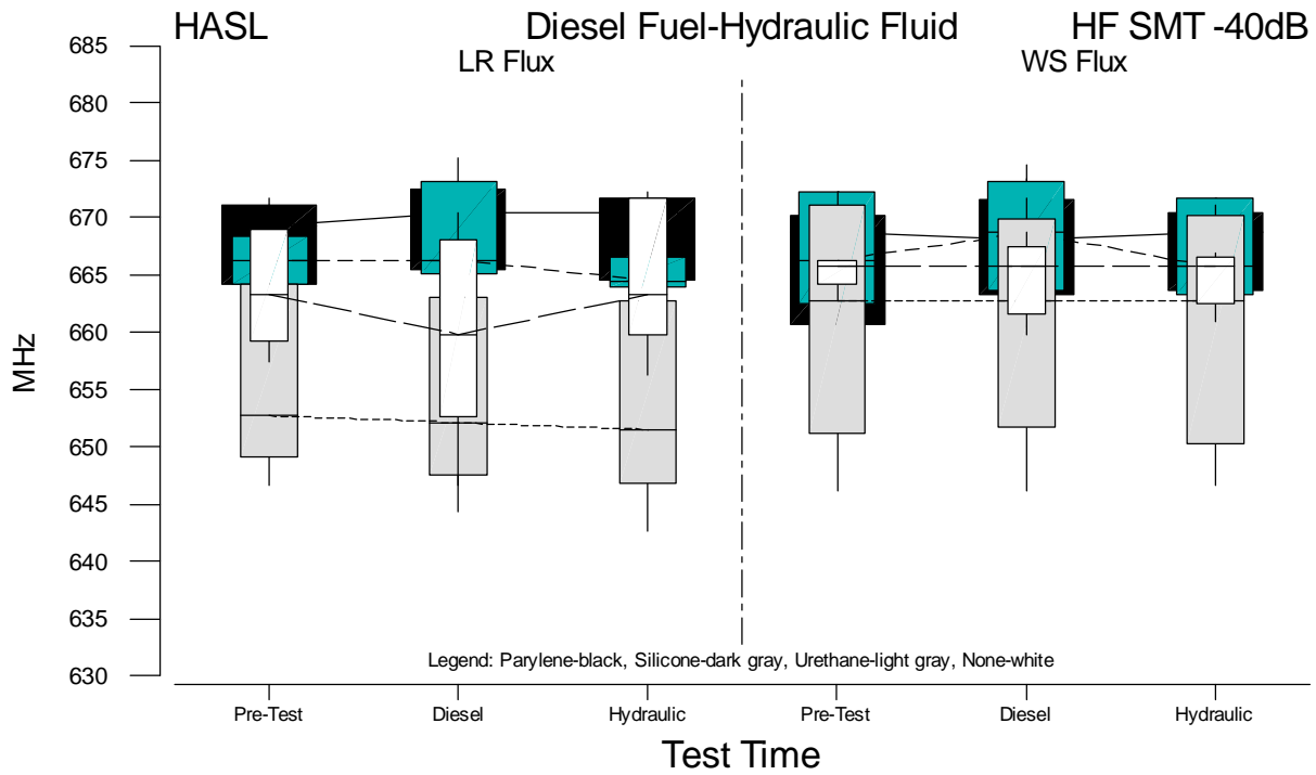
Figure B.45 Boxplots of HF SMT f(-40dB) Measurements for HASL versus Test Time
