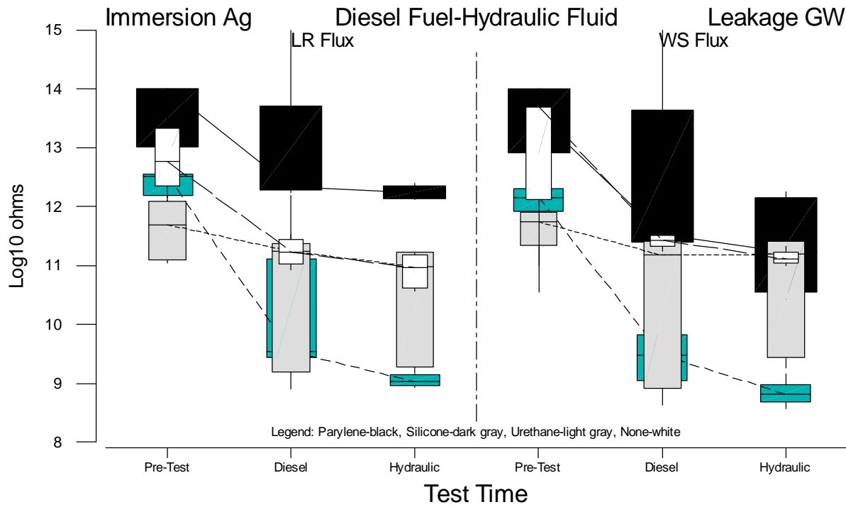
Figure B.83 Boxplots of Gull Wing Leakage Measurements for Immersion Ag versus Test Time
