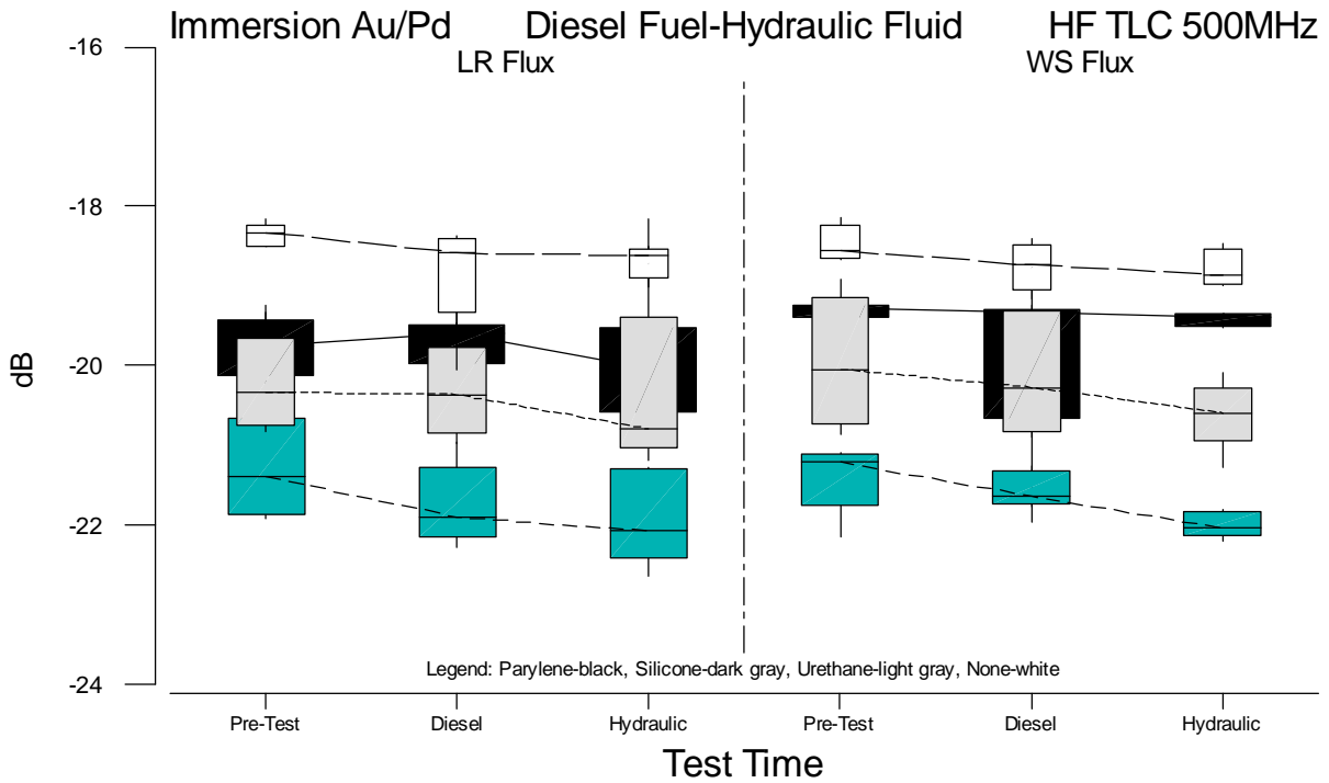
Figure B.56 Boxplots of HF TLC 500MHz Measurements for Immersion Au/Pd versus Test Time
