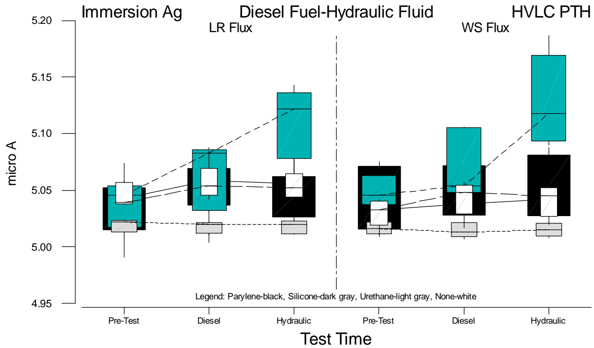
Figure B.11 Boxplots of HVLC PTH Current Measurements for Immersion Ag versus Test Time
