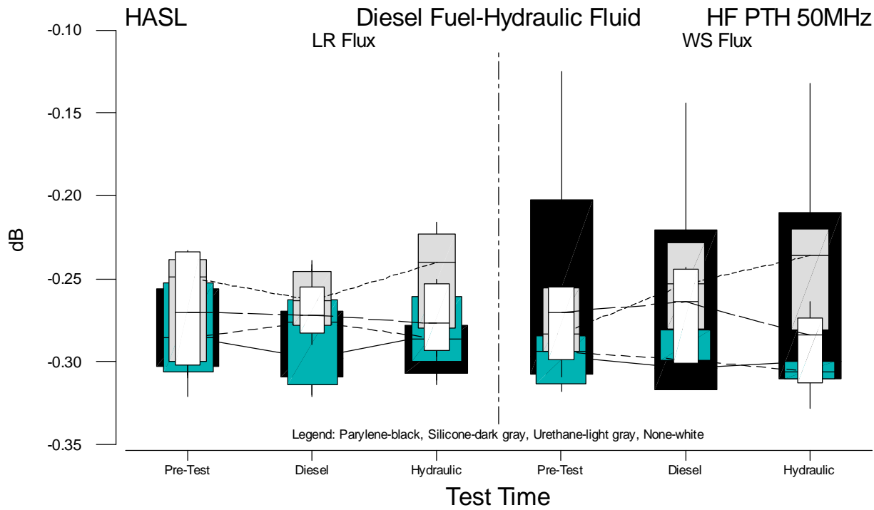
Figure B.25 Boxplots of HF PTH 50MHz Measurements for HASL versus Test Time
