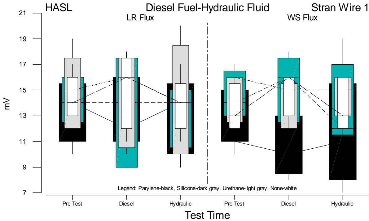
Figure B.85 Boxplots of Stranded Wire 1 Voltage Measurements for HASL versus Test Time
