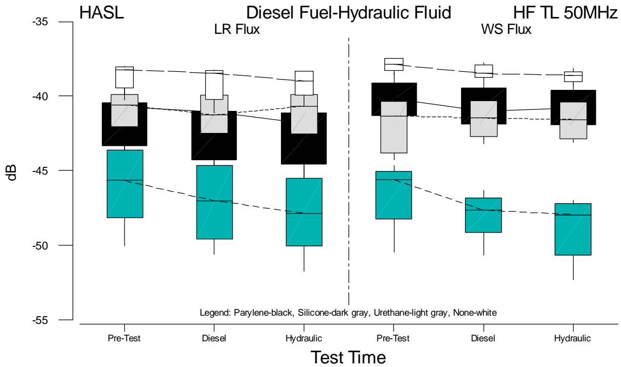
Figure B.49 Boxplots of HF TLC 50MHz Measurements for HASL versus Test Time
