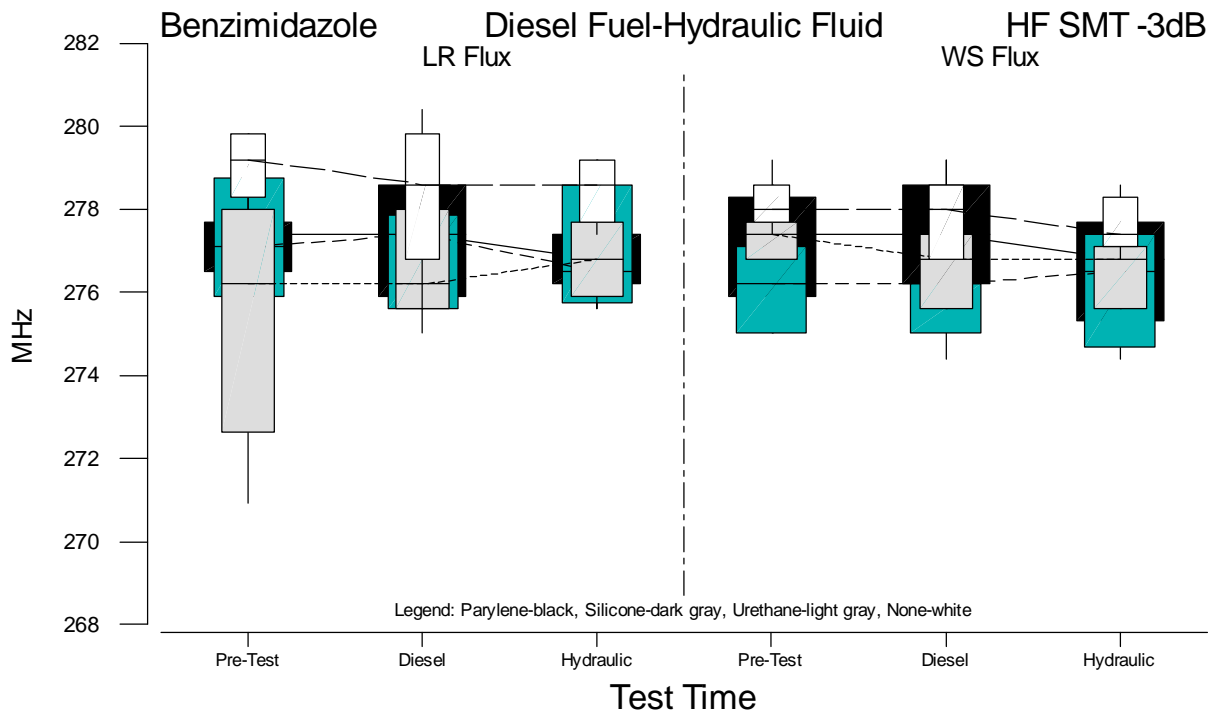
Figure B.42 Boxplots of HF SMT f(-3dB) Measurements for Benzimidazole versus Test Time
