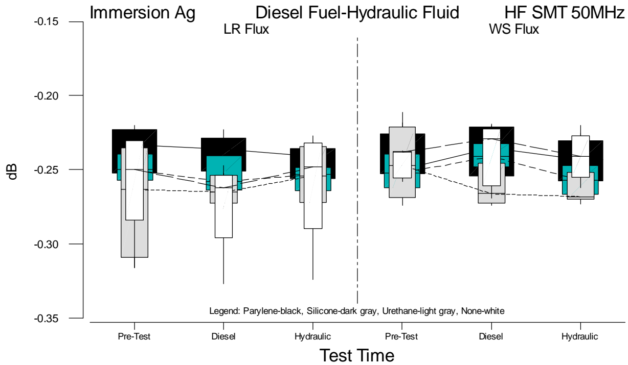
Figure B.39 Boxplots of HF SMT 50MHz Measurements for Immersion Ag versus Test Time
