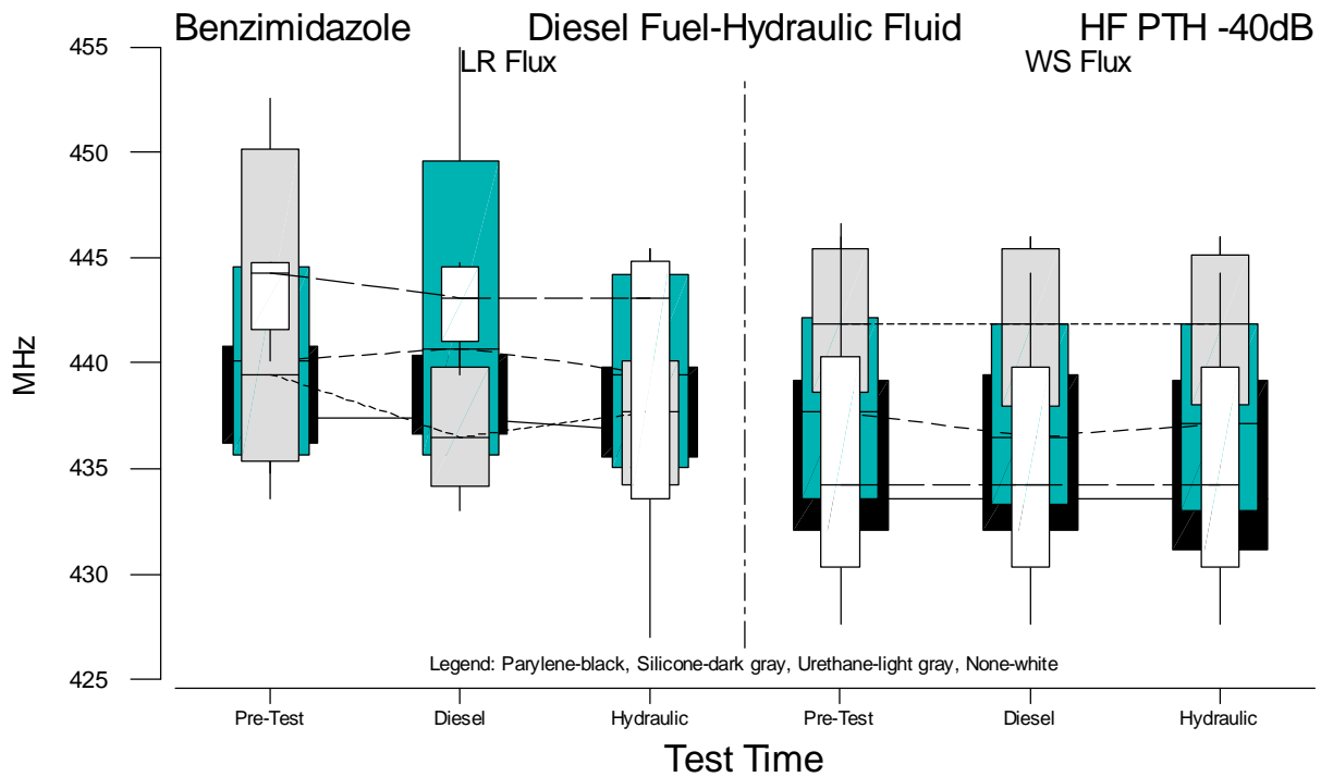
Figure B.34 Boxplots of HF PTH f(-40B) Measurements for Benzimidazole versus Test Time
