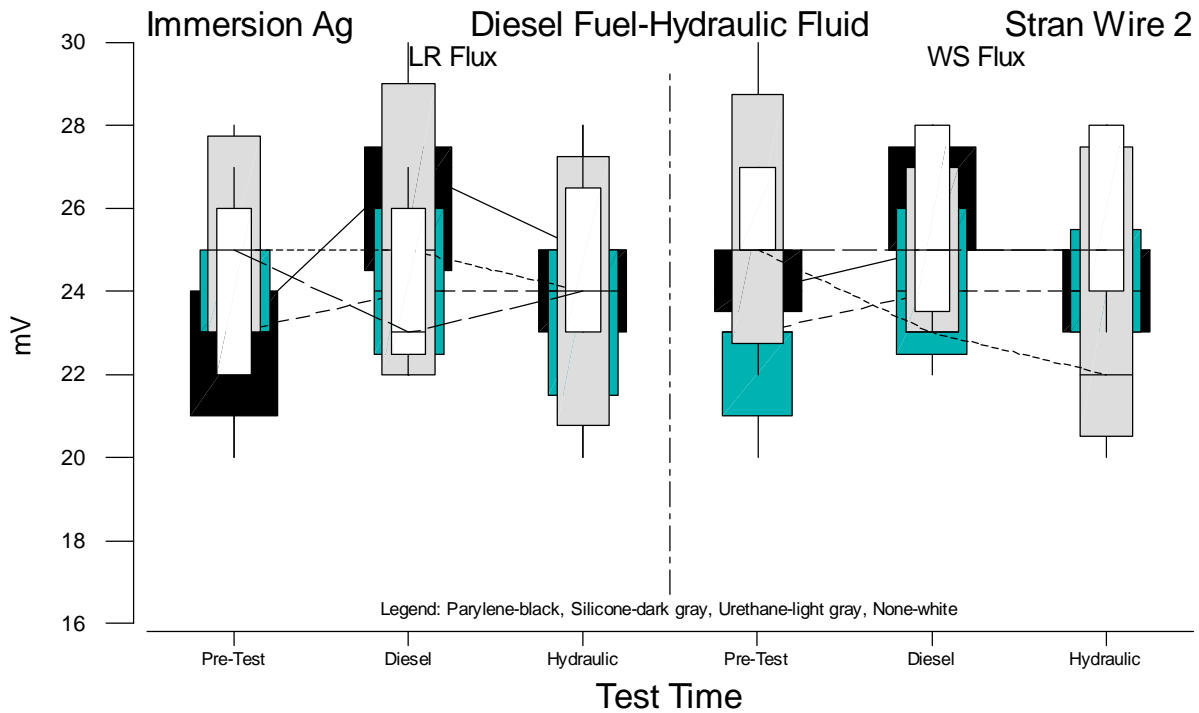
Figure B.91 Boxplots of Stranded Wire 2 Voltage Measurements for Immersion Ag versus Test Time
