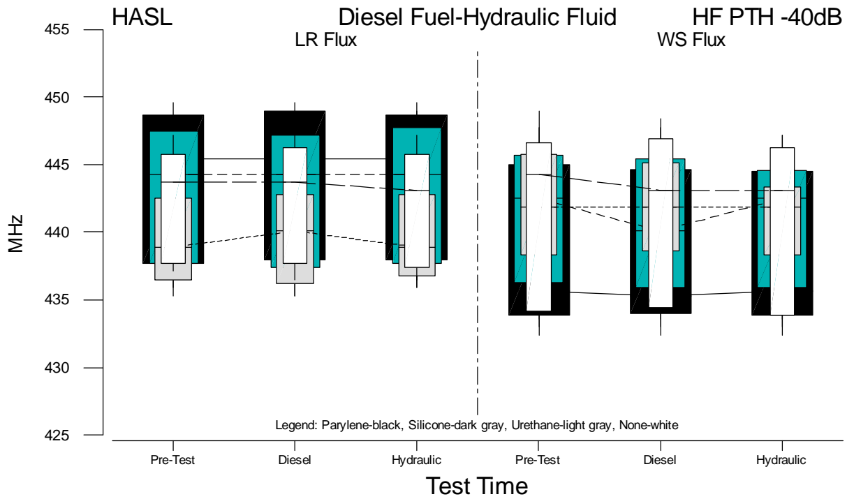
Figure B.33 Boxplots of HF PTH f(-40B) Measurements for HASL versus Test Time
