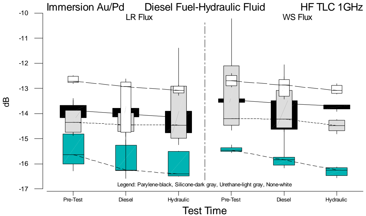
Figure B.60 Boxplots of HF TLC 1GHz Measurements for Immersion Au/Pd versus Test Time
