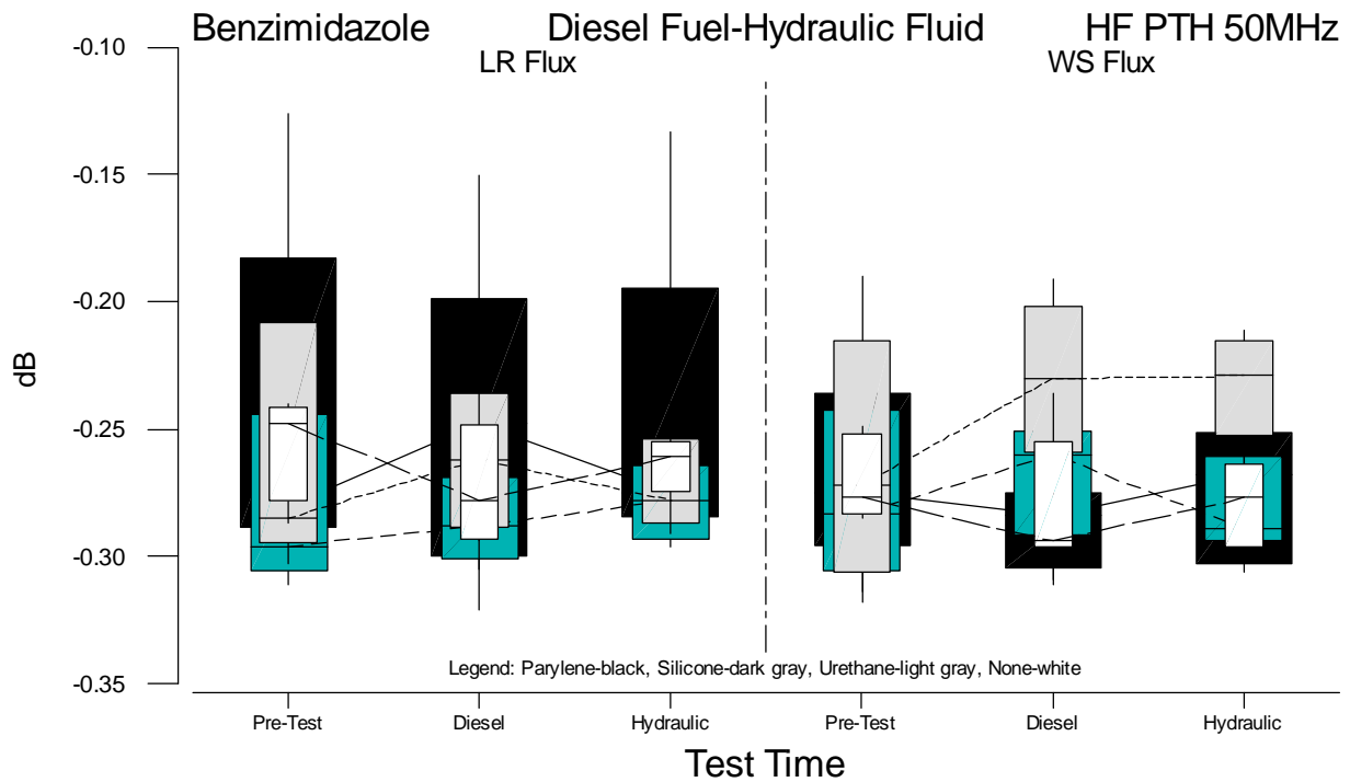
Figure B.26 Boxplots of HF PTH 50MHz Measurements for Benzimidazole versus Test Time
