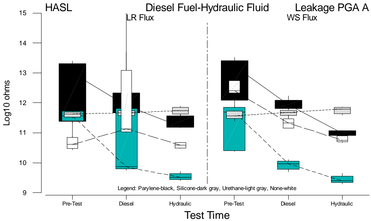
Figure B.73 Boxplots of PGA-A Leakage Measurements for HASL versus Test Time
