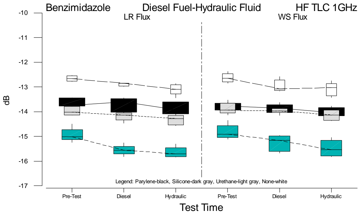
Figure B.58 Boxplots of HF TLC 1GHz Measurements for Benzimidazole versus Test Time
