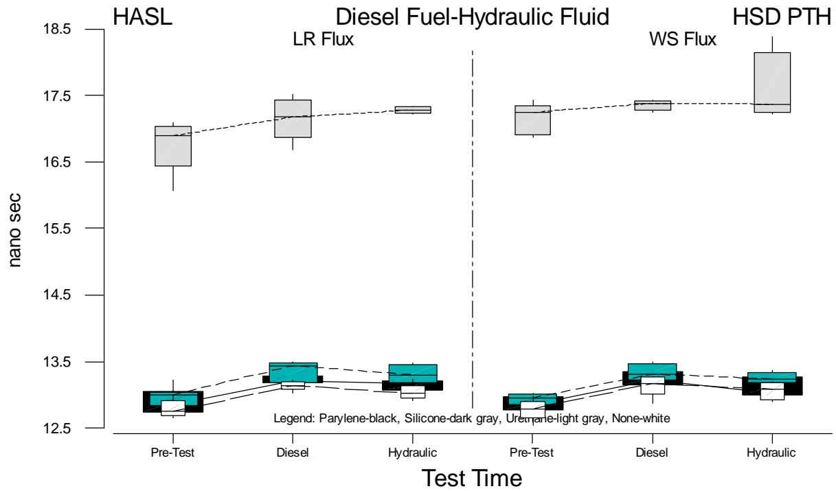
Figure B.17 Boxplots of HSD PTH Propagation Delay Measurements for HASL versus Test Time
