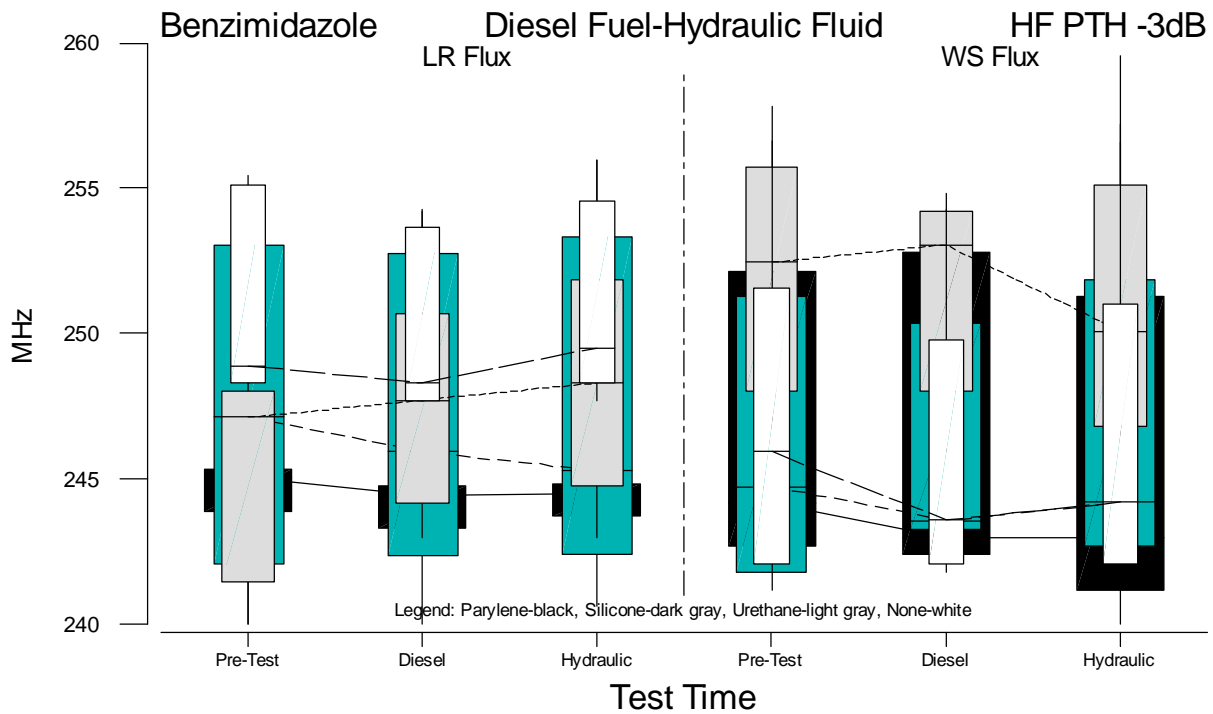
Figure B.30 Boxplots of HF PTH f(-3dB) Measurements for Benzimidazole versus Test Time
