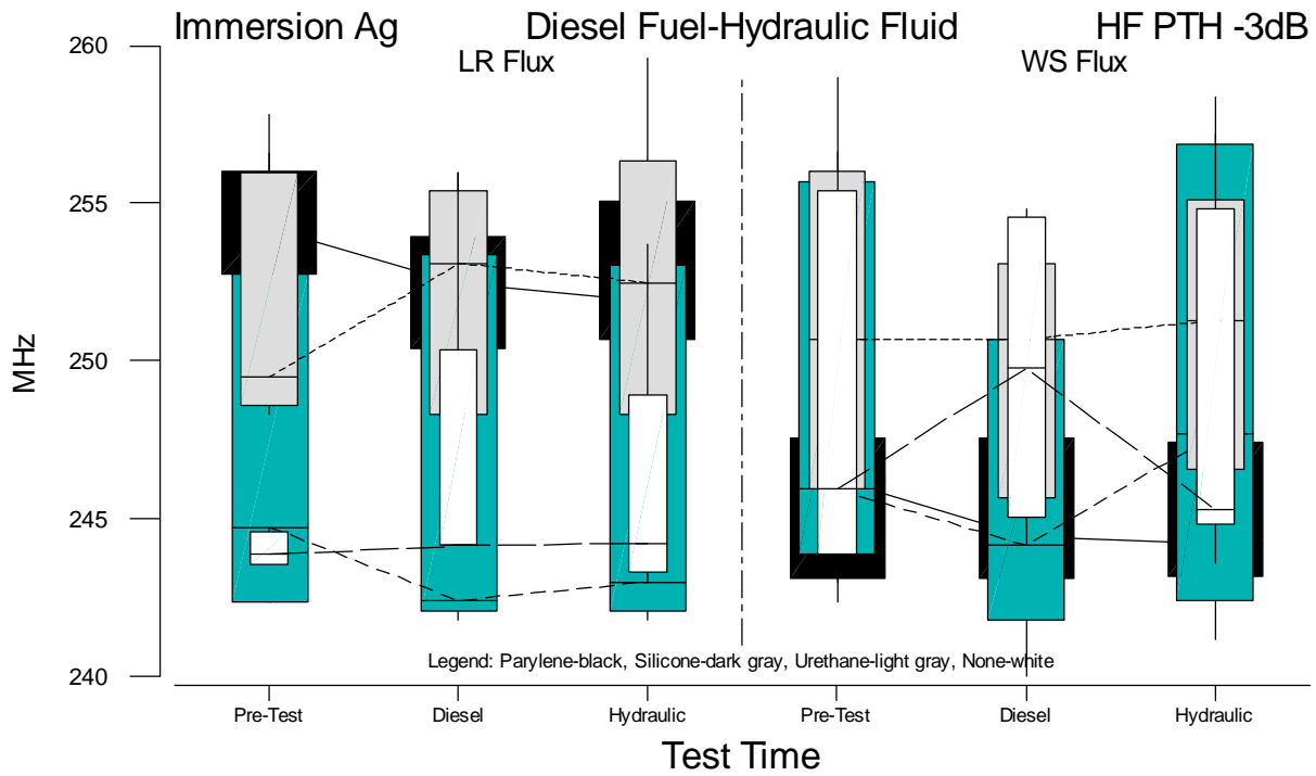
Figure B.31 Boxplots of HF PTH f(-3dB) Measurements for Immersion Ag versus Test Time
