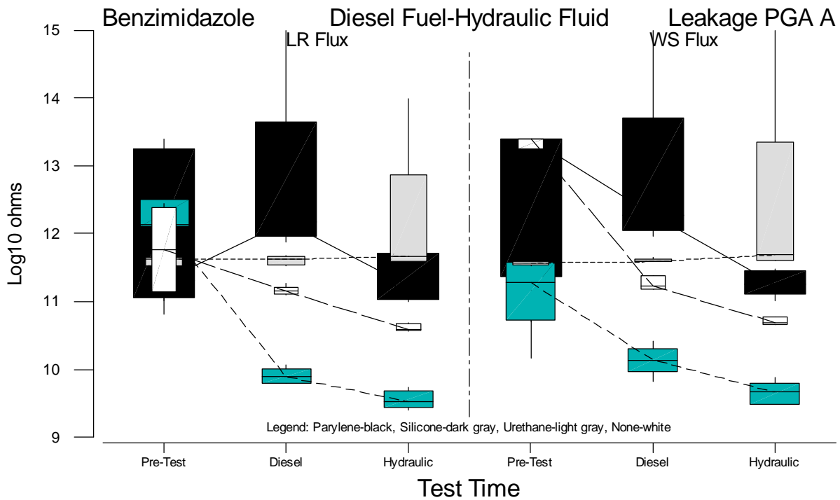
Figure B.74 Boxplots of PGA-A Leakage Measurements for Benzimidazole versus Test Time
