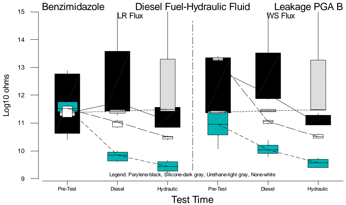
Figure B.78 Boxplots of PGA-B Leakage Measurements for Benzimidazole versus Test Time
