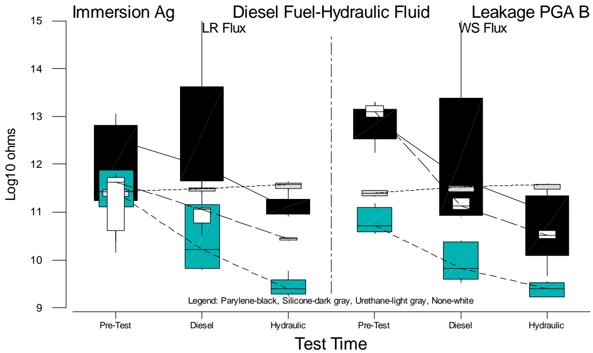
Figure B.79 Boxplots of PGA-B Leakage Measurements for Immersion Ag versus Test Time
