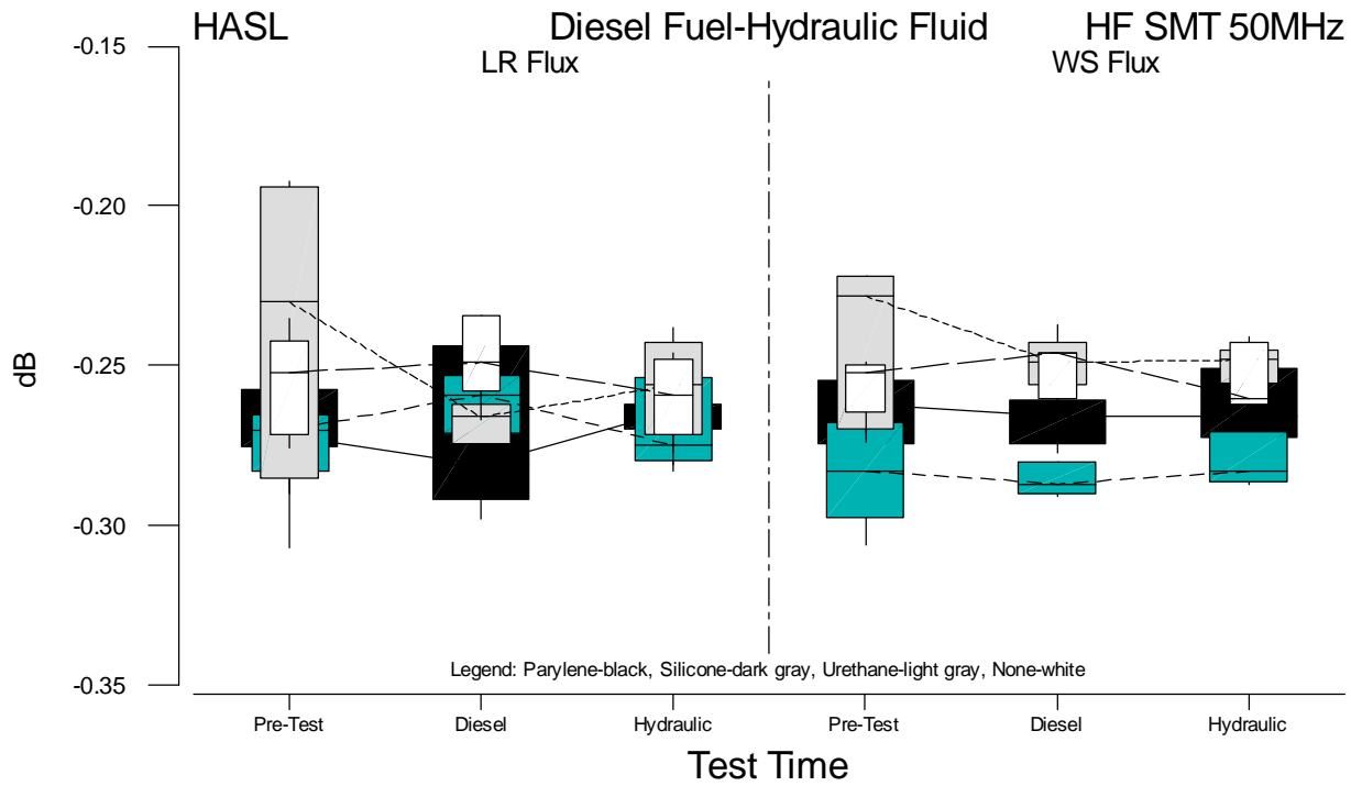
Figure B.37 Boxplots of HF SMT 50MHz Measurements for HASL versus Test Time
