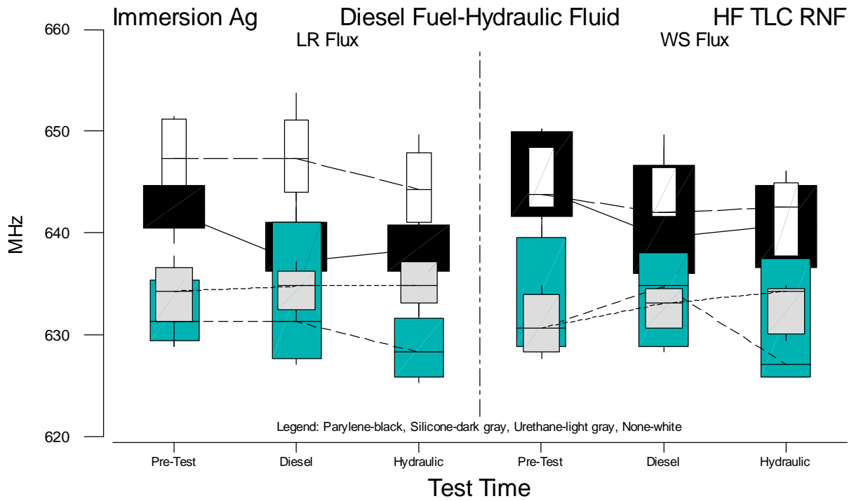
Figure B.63 Boxplots of HF TLC Rev. Null Frequency Measurements for Immersion Ag vs. Test Time
