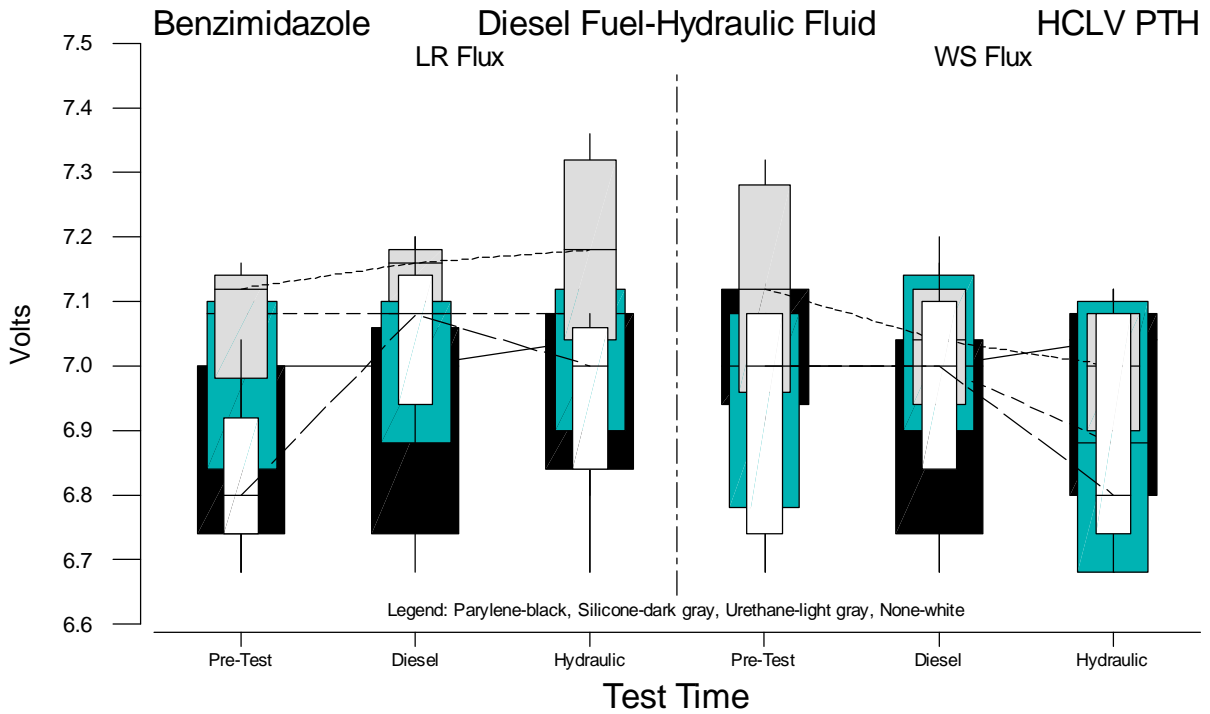
Figure B.2 Boxplots of HCLV PTH Voltage Measurements for Benzimidazole versus Test Time
