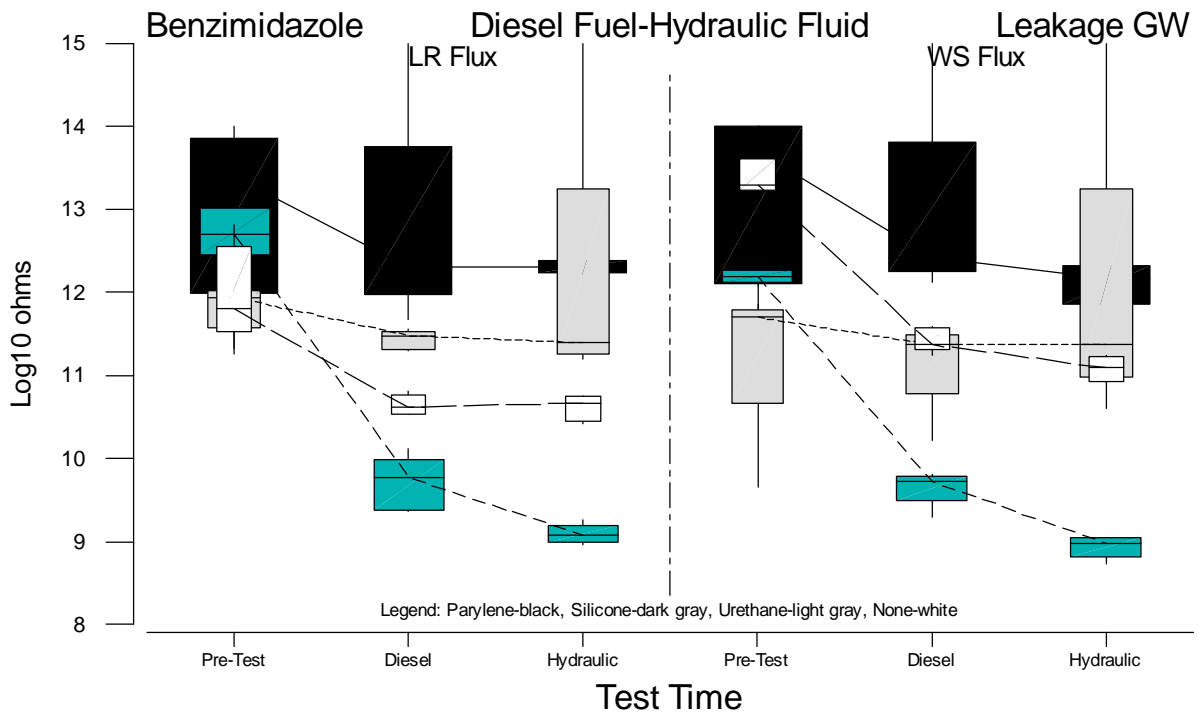
Figure B.82 Boxplots of Gull Wing Leakage Measurements for Benzimidazole versus Test Time
