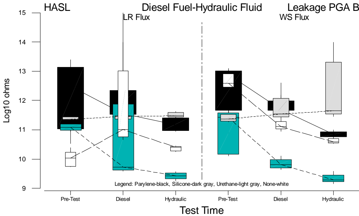
Figure B.77 Boxplots of PGA-B Leakage Measurements for HASL versus Test Time
