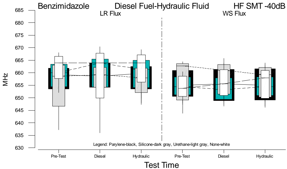
Figure B.46 Boxplots of HF SMT f(-40dB) Measurements for Benzimidazole versus Test Time
