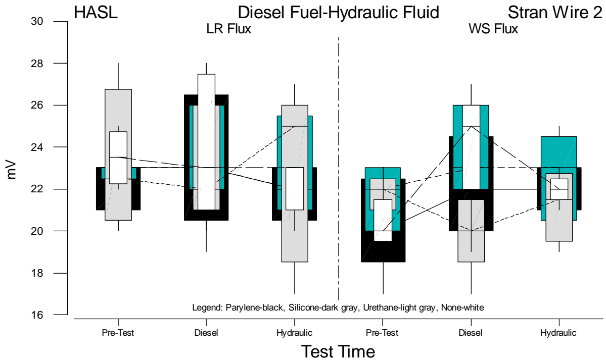
Figure B.89 Boxplots of Stranded Wire 2 Voltage Measurements for HASL versus Test Time
