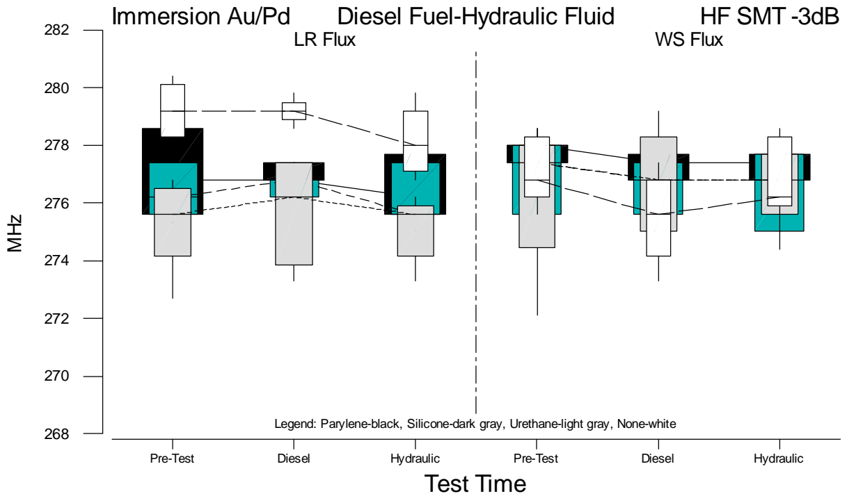
Figure B.44 Boxplots of HF SMT f(-3dB) Measurements for Immersion Au/Pd versus Test Time
