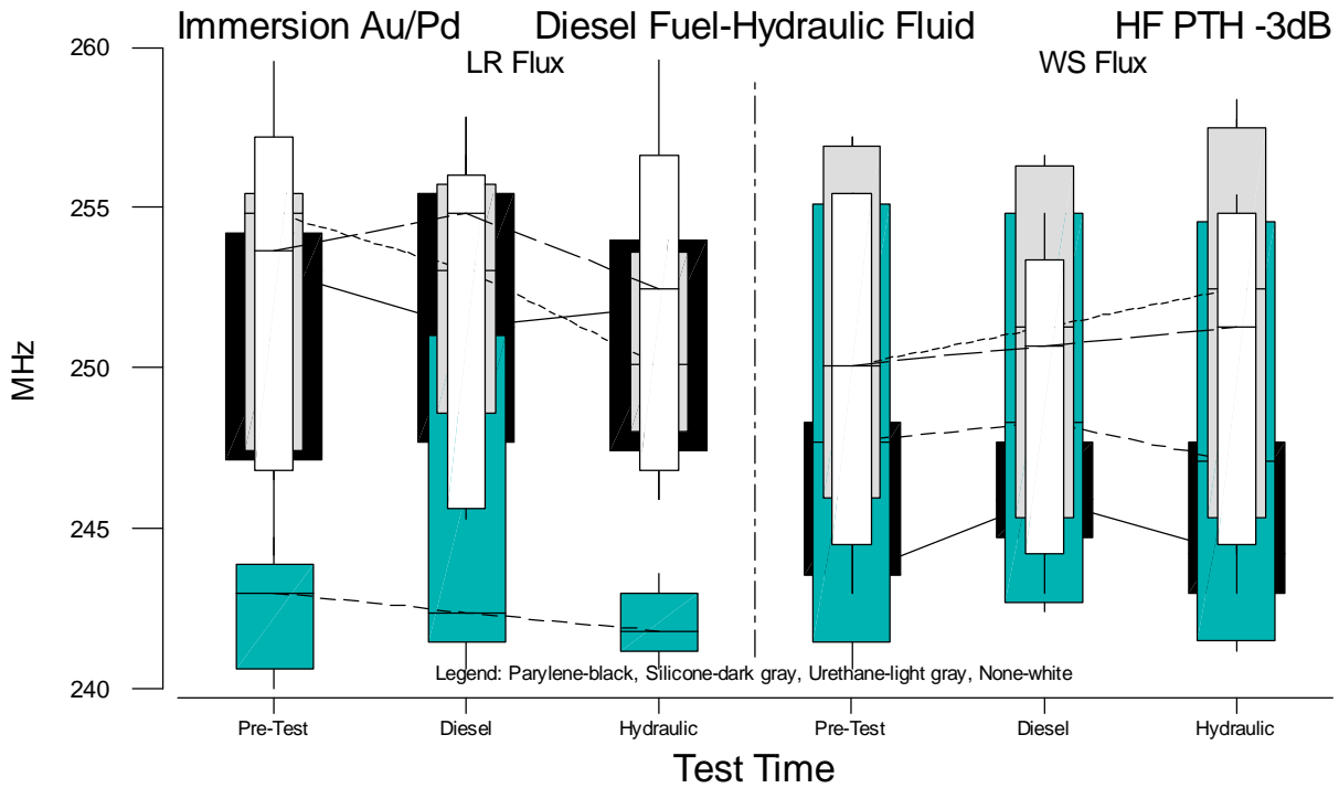
Figure B.32 Boxplots of HF PTH f(-3dB) Measurements for Immersion Au/Pd versus Test Time
