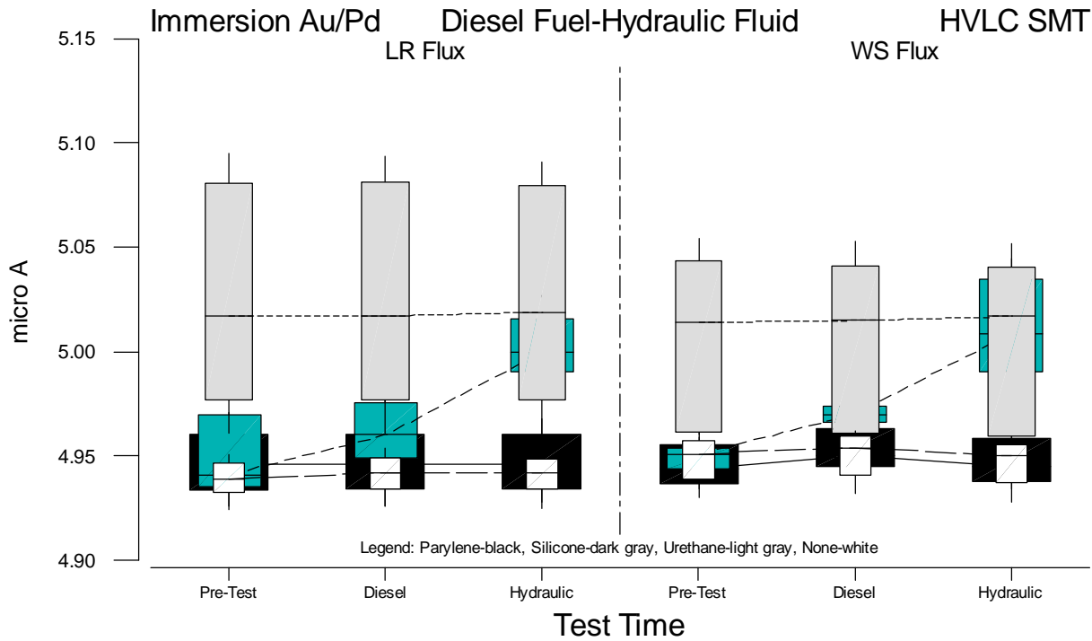
Figure B.16 Boxplots of HVLC SMT Current Measurements for Immersion Au/Pd vs. Test Time
