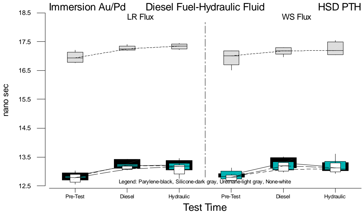
Figure B.20 Boxplots of HSD PTH Propagation Delay Measurements for Immersion Au/Pd vs. Test Time
