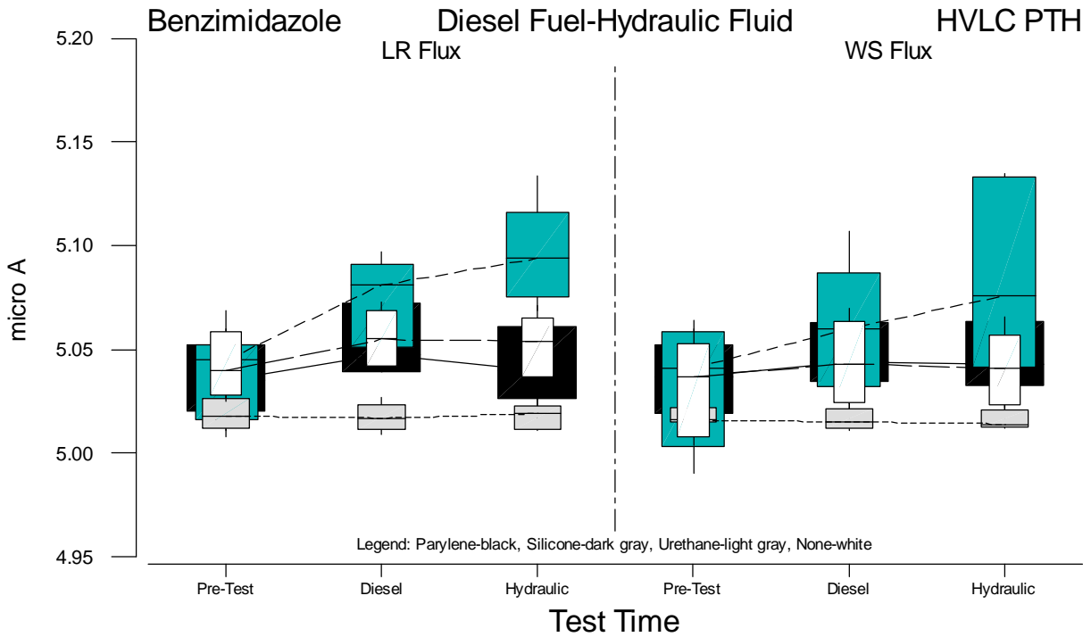
Figure B.10 Boxplots of HVLC PTH Current Measurements for Benzimidazole versus Test Time
