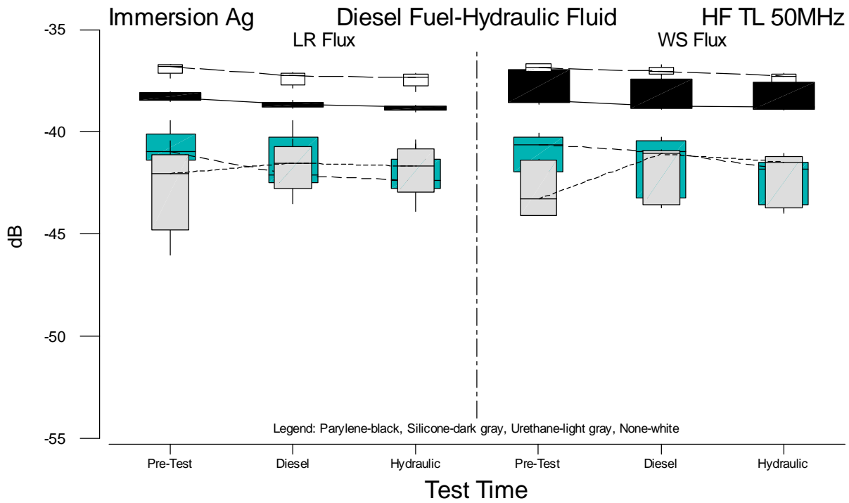
Figure B.51 Boxplots of HF TLC 50MHz Measurements for Immersion Ag versus Test Time
