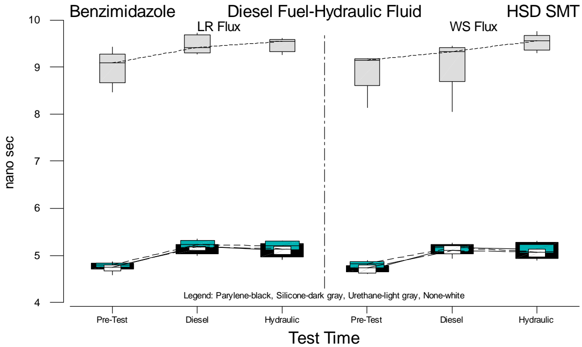
Figure B.22 Boxplots of HSD SMT Propagation Delay Measurements for Benzimidazole versus Test Time
