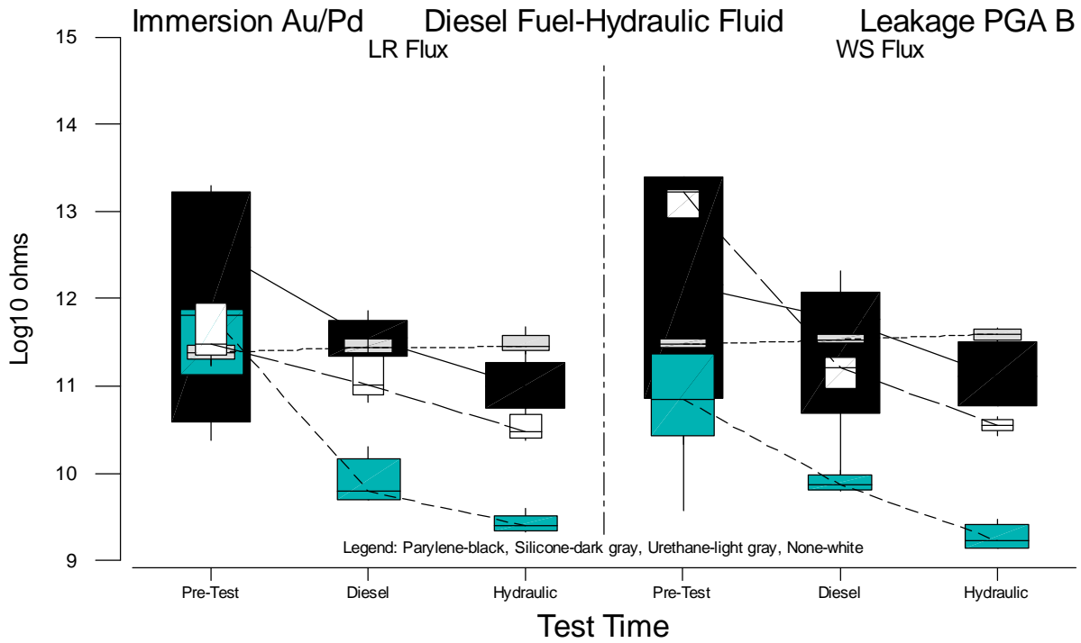
Figure B.80 Boxplots of PGA-B Leakage Measurements for Immersion Au/Pd versus Test Time
