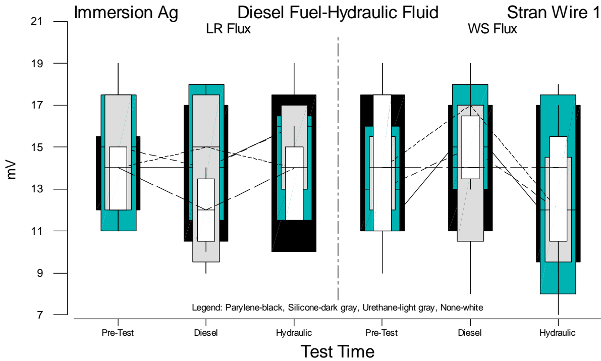
Figure B.87 Boxplots of Stranded Wire 1 Voltage Measurements for Immersion Ag versus Test Time
