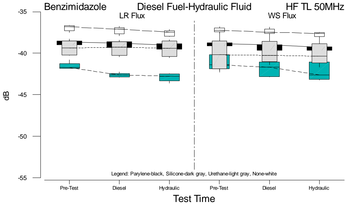
Figure B.50 Boxplots of HF TLC 50MHz Measurements for Benzimidazole versus Test Time
