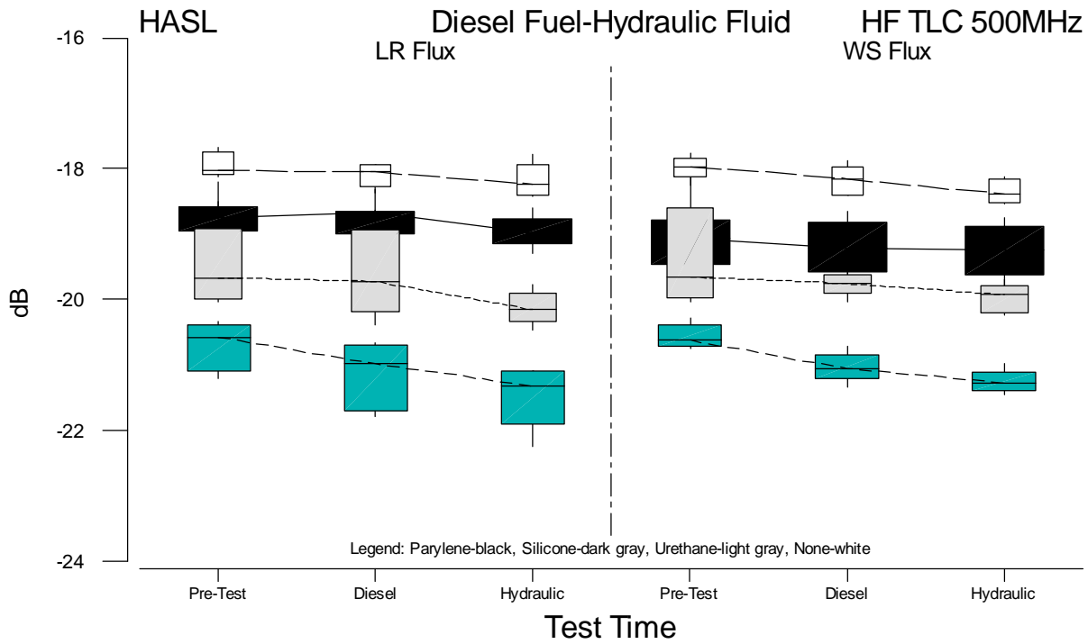
Figure B.53 Boxplots of HF TLC 500MHz Measurements for HASL versus Test Time
