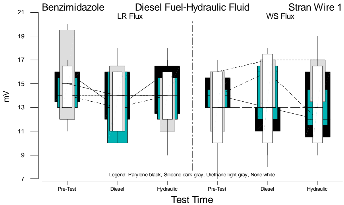
Figure B.86 Boxplots of Stranded Wire 1 Voltage Measurements for Benzimidazole versus Test Time
