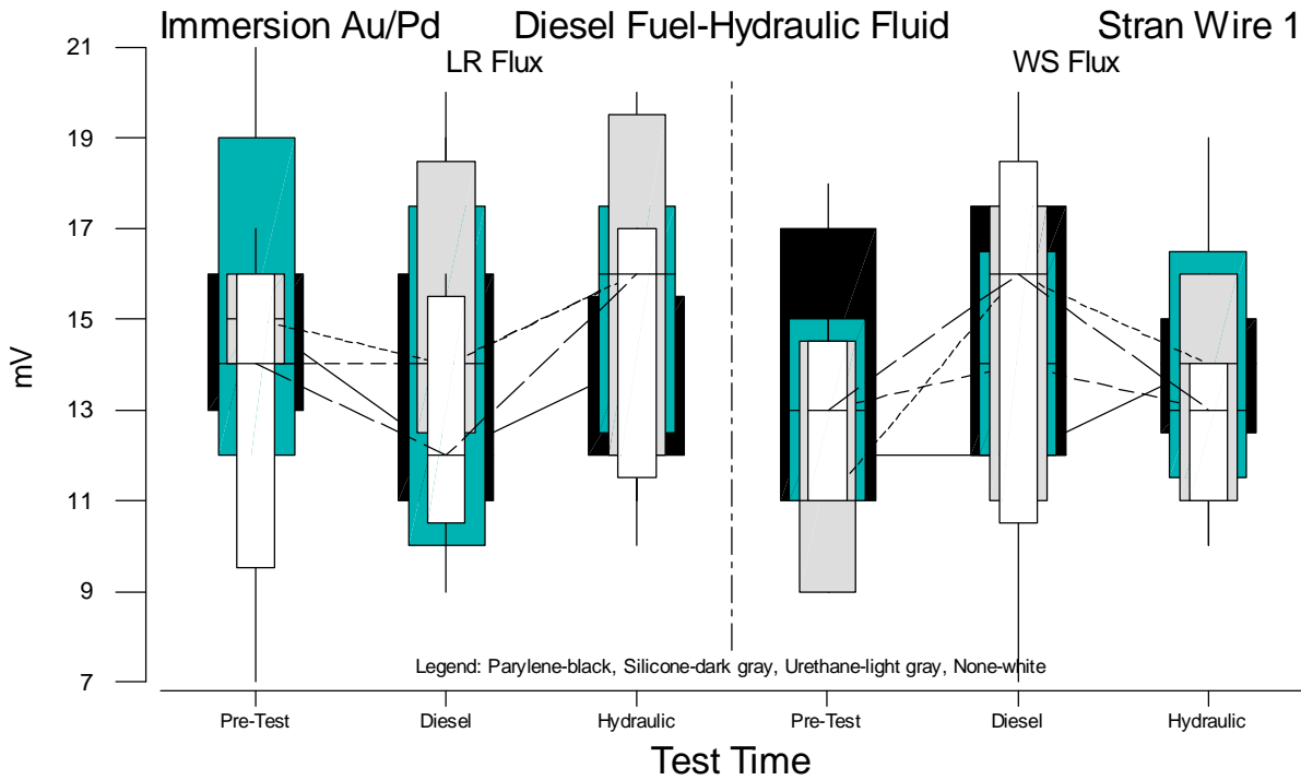
Figure B.88 Boxplots of Stranded Wire 1 Voltage Measurements for Immersion Au/Pd versus Test Time
