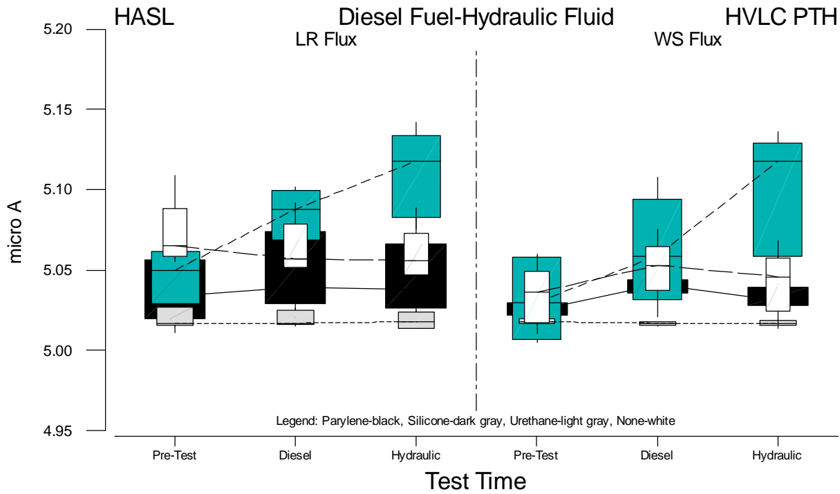
Figure B.9 Boxplots of HVLC PTH Current Measurements for HASL versus Test Time
