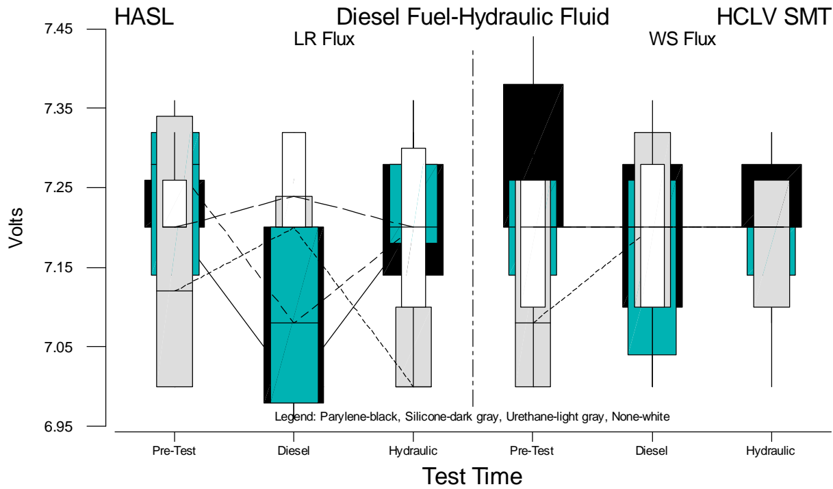
Figure B.5 Boxplots of HCLV SMT Voltage Measurements for HASL versus Test Time
