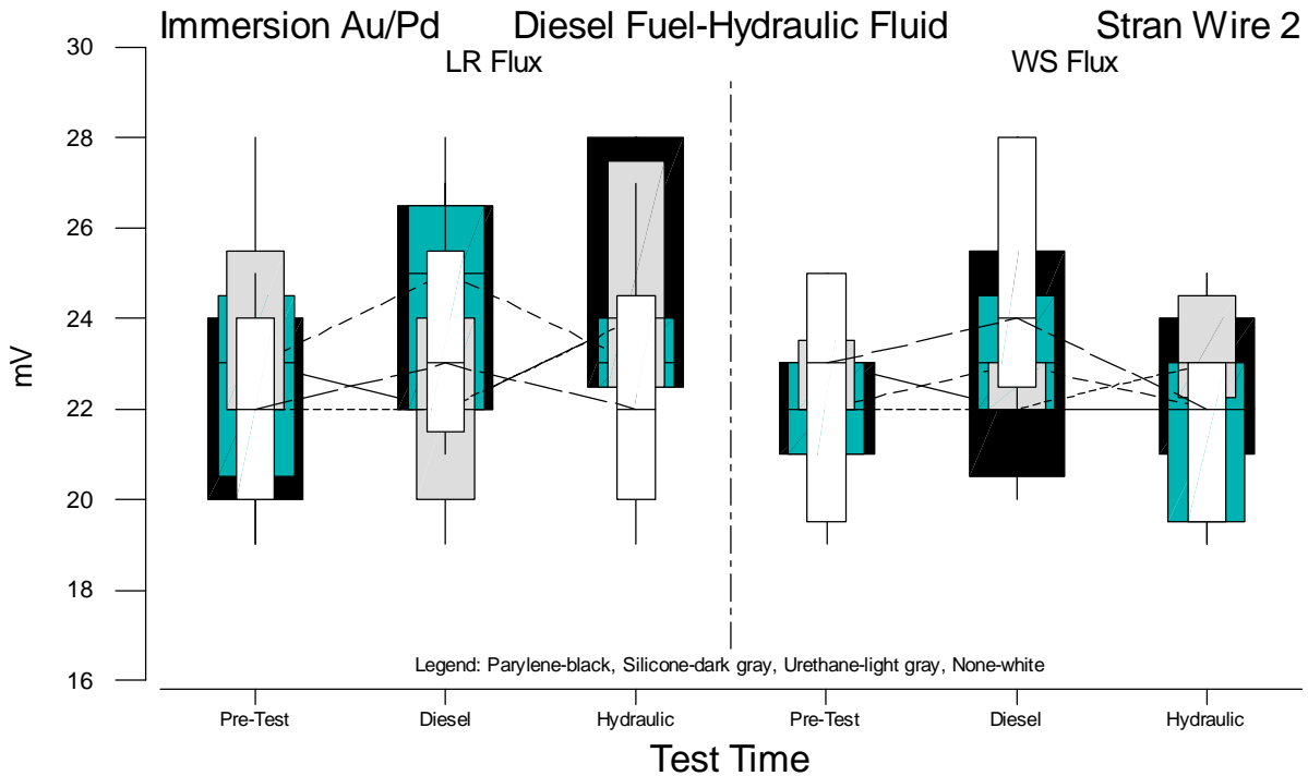
Figure B.92 Boxplots of Stranded Wire 2 Voltage Measurements for Immersion Au/Pd versus Test Time
