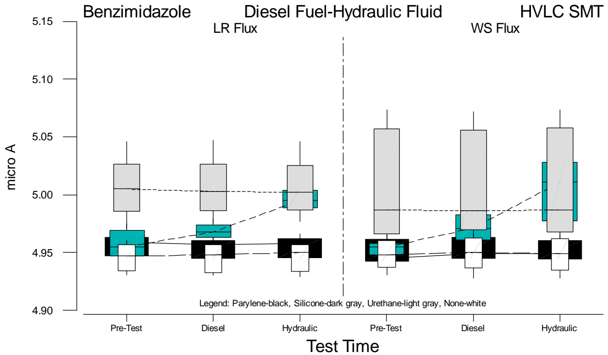
Figure B.14 Boxplots of HVLC SMT Current Measurements for Benzimidazole versus Test Time
