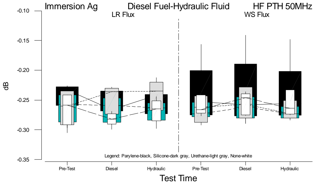
Figure B.27 Boxplots of HF PTH 50MHz Measurements for Immersion Ag versus Test Time
