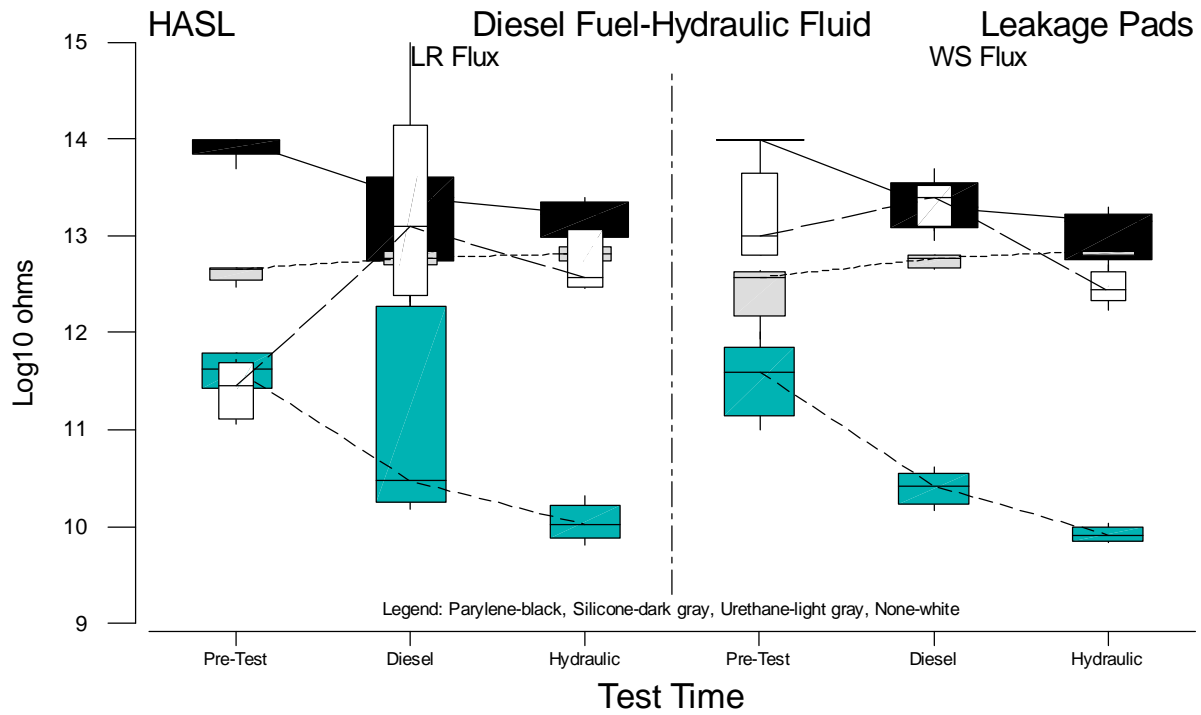
Figure B.69 Boxplots of 10-Mil Leakage Measurements for HASL versus Test Time
