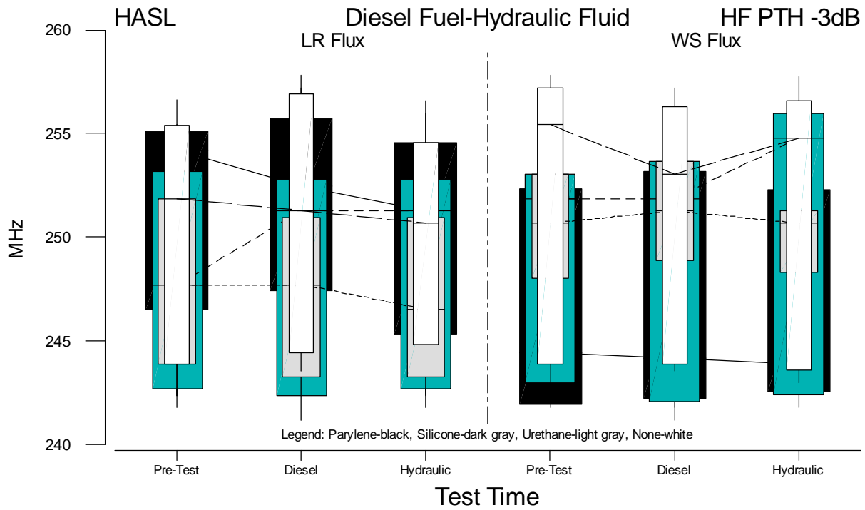
Figure B.29 Boxplots of HF PTH f(-3dB) Measurements for HASL versus Test Time
