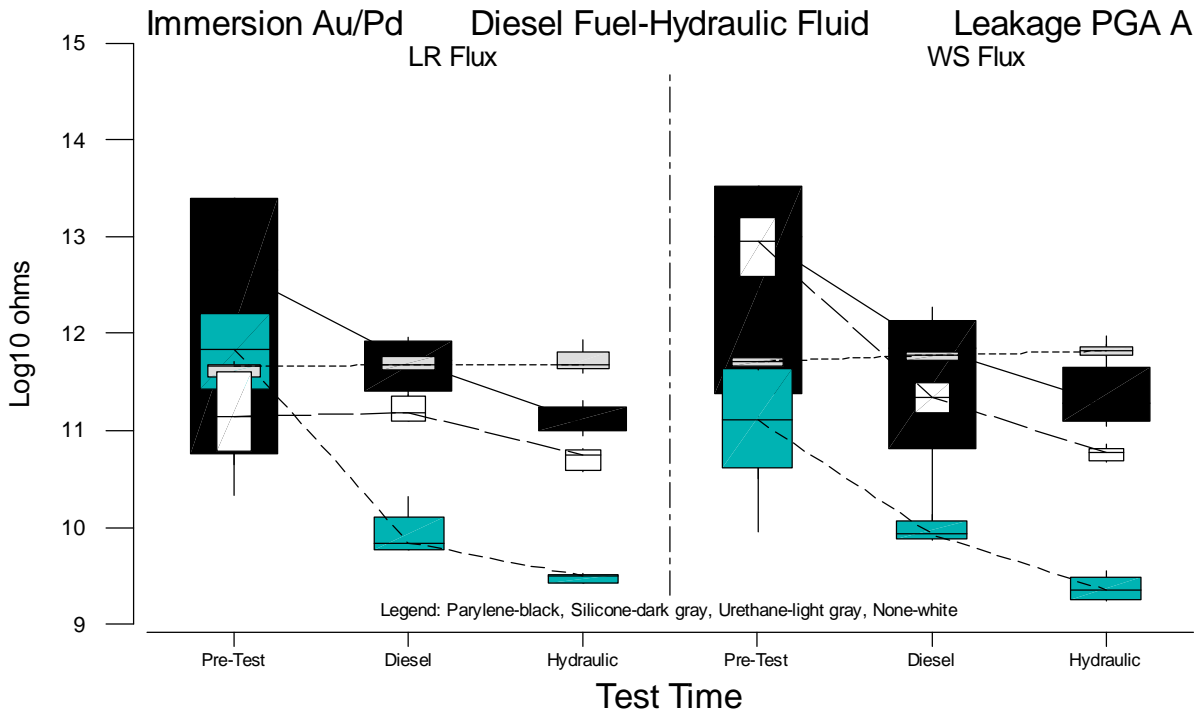
Figure B.76 Boxplots of PGA-A Leakage Measurements for Immersion Au/Pd vs. Test Time
