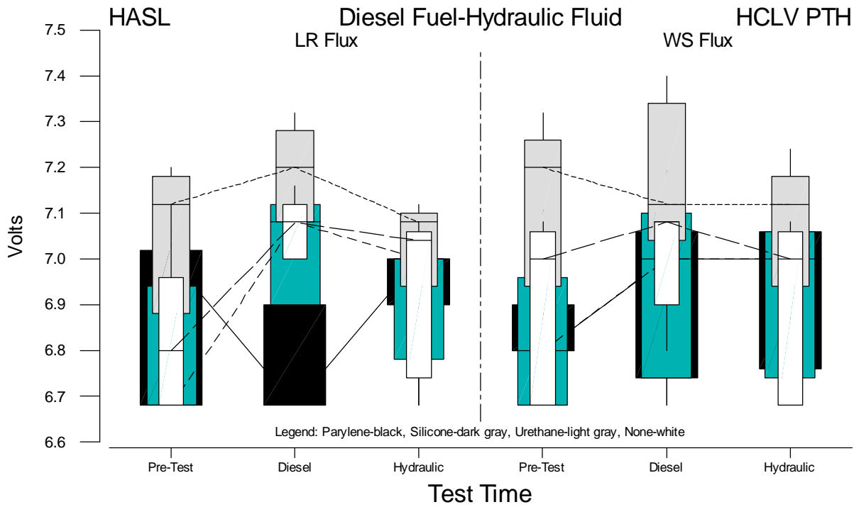
Figure B.1 Boxplots of HCLV PTH Voltage Measurements for HASL versus Test Time
