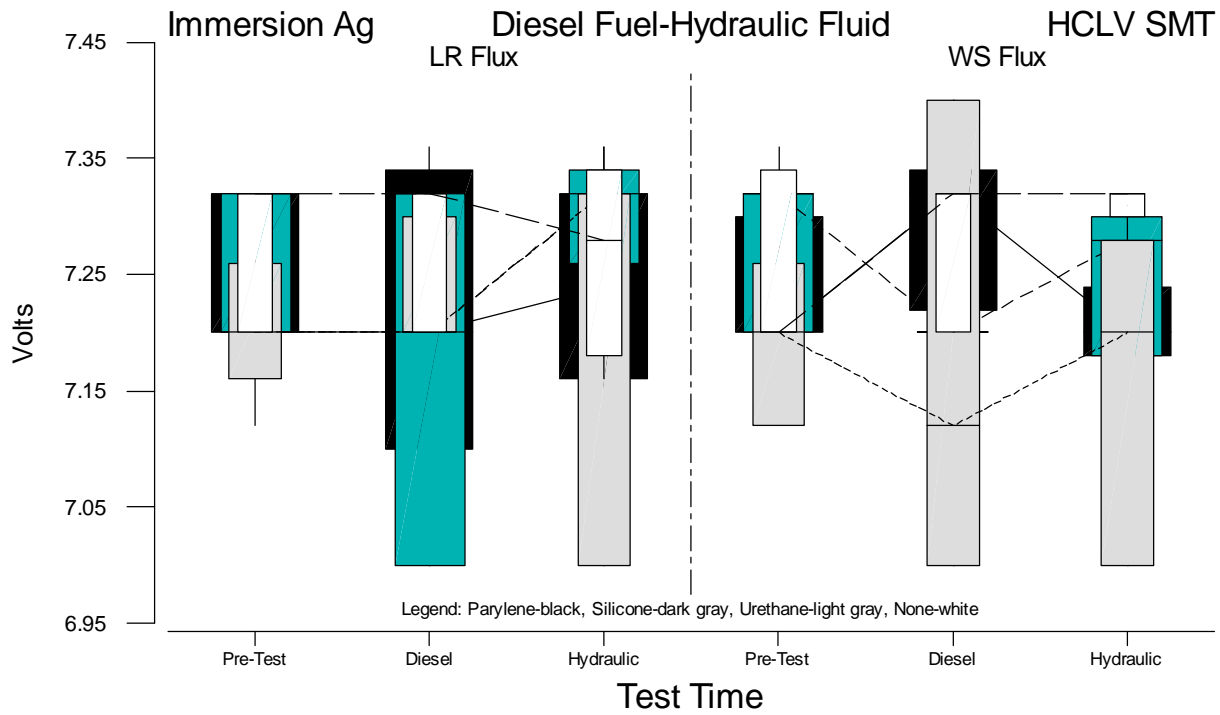
Figure B.7 Boxplots of HCLV SMT Voltage Measurements for Immersion Ag versus Test Time
