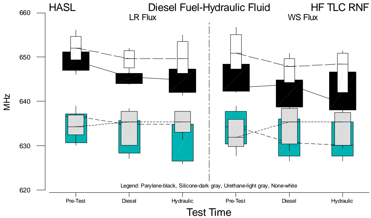
Figure B.61 Boxplots of HF TLC Rev. Null Frequency Measurements for HASL versus Test Time
