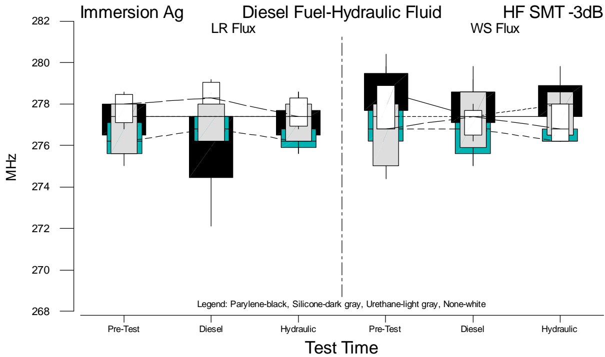
Figure B.43 Boxplots of HF SMT f(-3dB) Measurements for Immersion Ag versus Test Time
