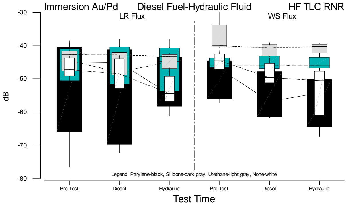
Figure B.68 Boxplots of HF TLC Rev. Null Response Measurements for Immersion Au/Pd vs. Test Time
