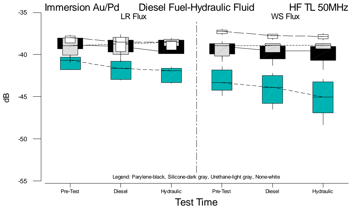
Figure B.52 Boxplots of HF TLC 50MHz Measurements for Immersion Au/Pd versus Test Time
