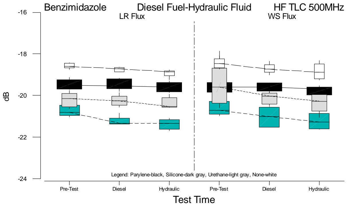
Figure B.54 Boxplots of HF TLC 500MHz Measurements for Benzimidazole versus Test Time
