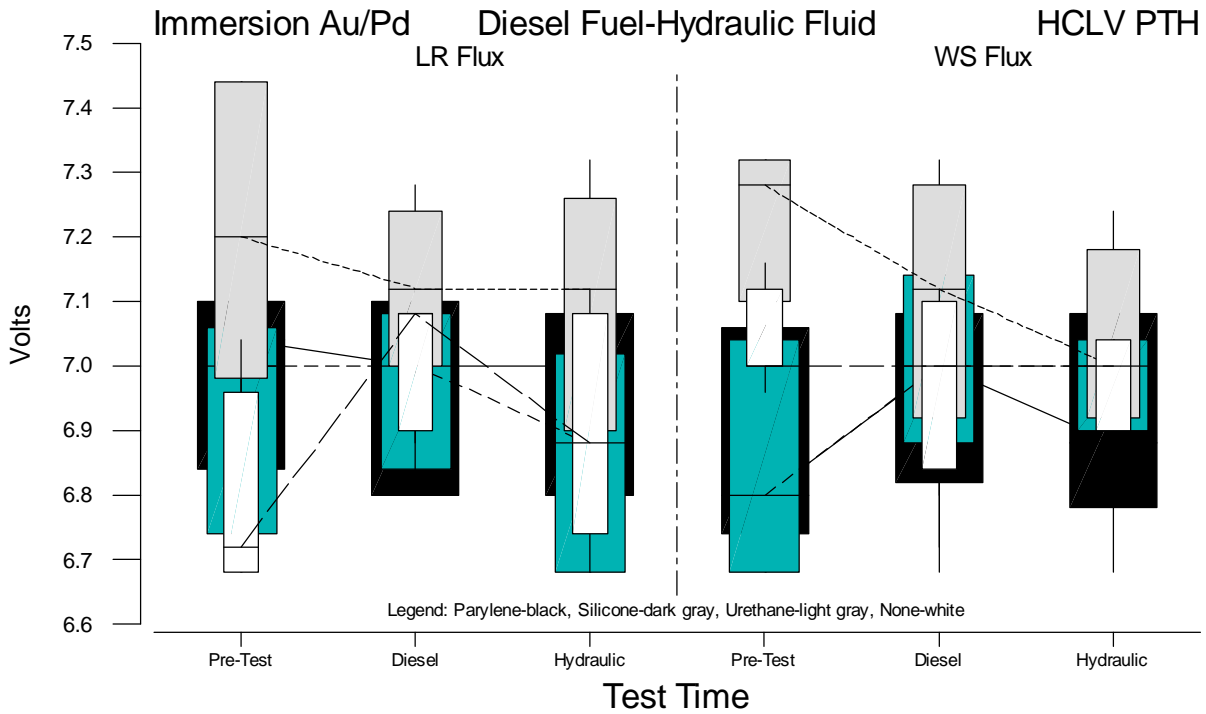
Figure B.4 Boxplots of HCLV PTH Voltage Measurements for Immersion Au/Pd versus Test Time
