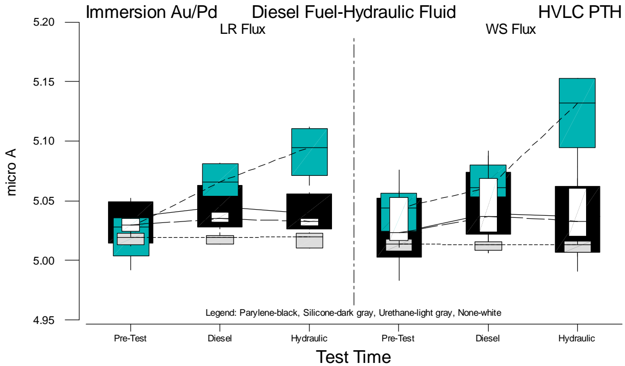
Figure B.12 Boxplots of HVLC PTH Current Measurements for Immersion Au/Pd versus Test Time
