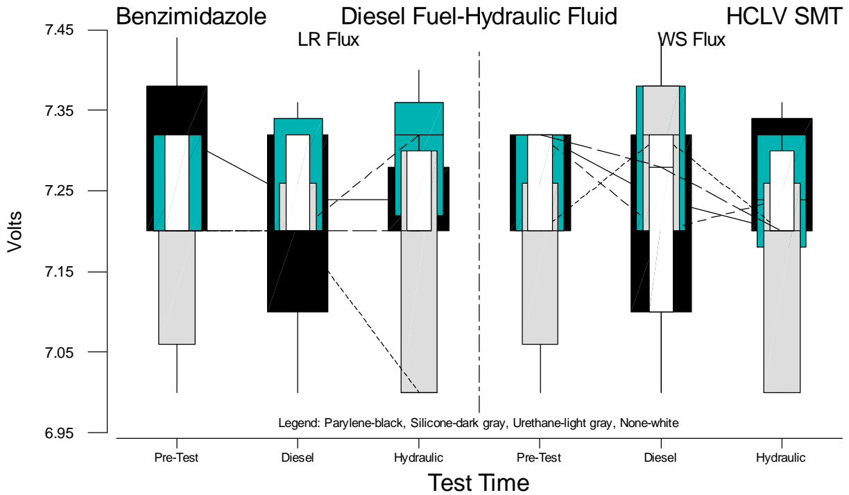
Figure B.6 Boxplots of HCLV SMT Voltage Measurements for Benzimidazole versus Test Time
