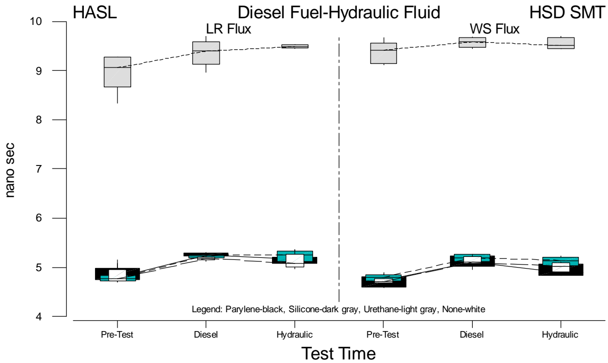
Figure B.21 Boxplots of HSD SMT Propagation Delay Measurements for HASL versus Test Time
