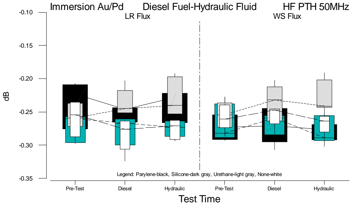
Figure B.28 Boxplots of HF PTH 50MHz Measurements for Immersion Au/Pd versus Test Time
