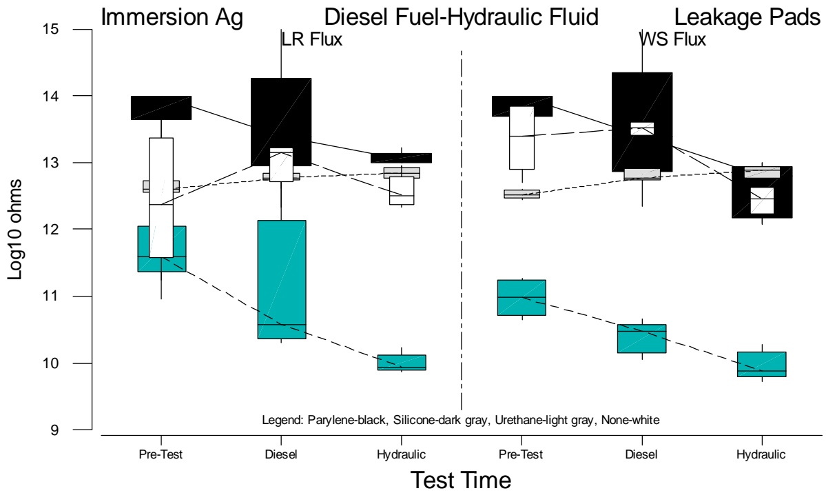
Figure B.71 Boxplots of 10-Mil Leakage Measurements for Immersion Ag versus Test Time
