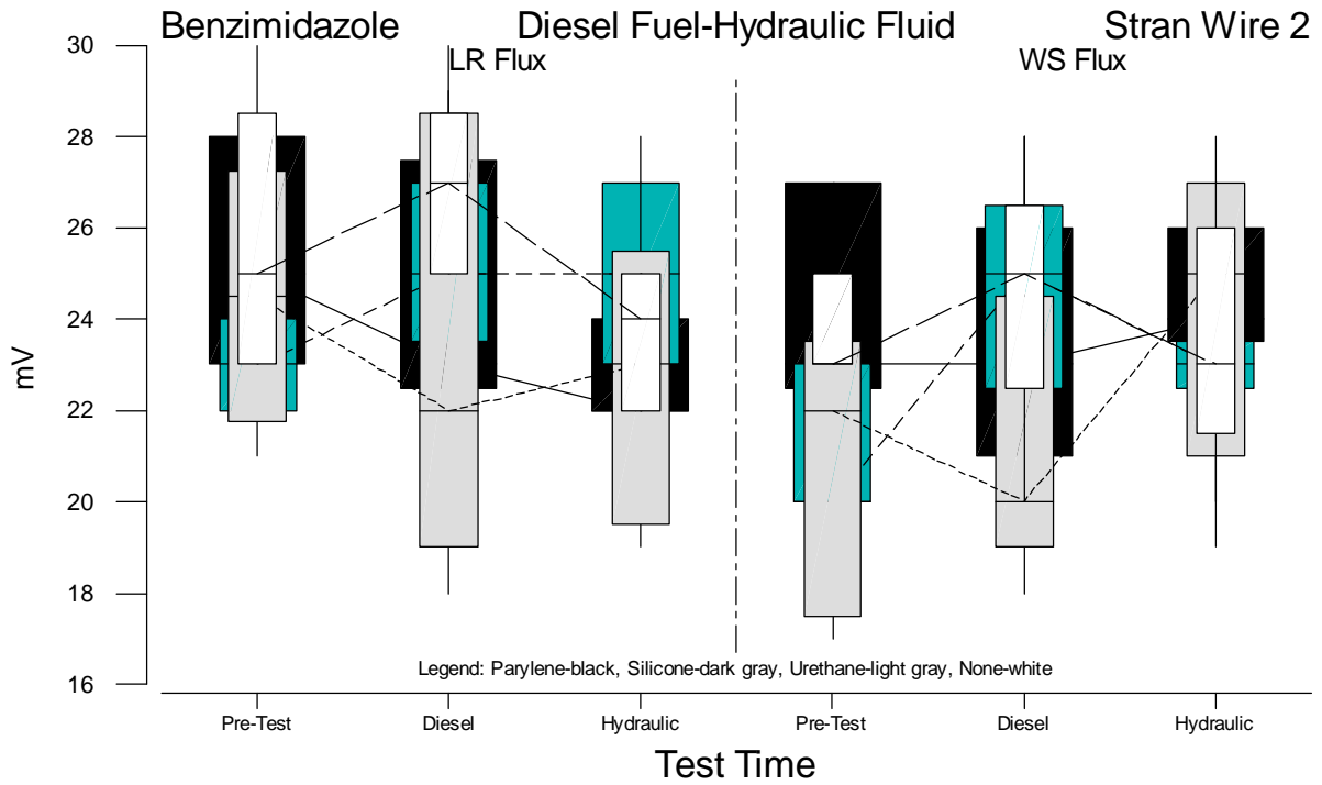
Figure B.90 Boxplots of Stranded Wire 2 Voltage Measurements for Benzimidazole versus Test Time
