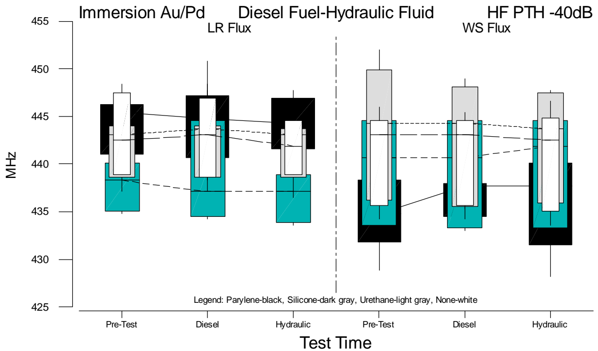
Figure B.36 Boxplots of HF PTH f(-40B) Measurements for Immersion Au/Pd versus Test Time
