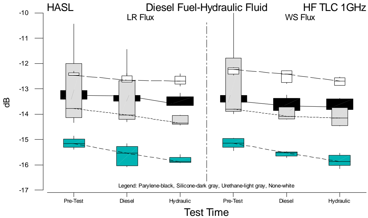
Figure B.57 Boxplots of HF TLC 1GHz Measurements for HASL versus Test Time
