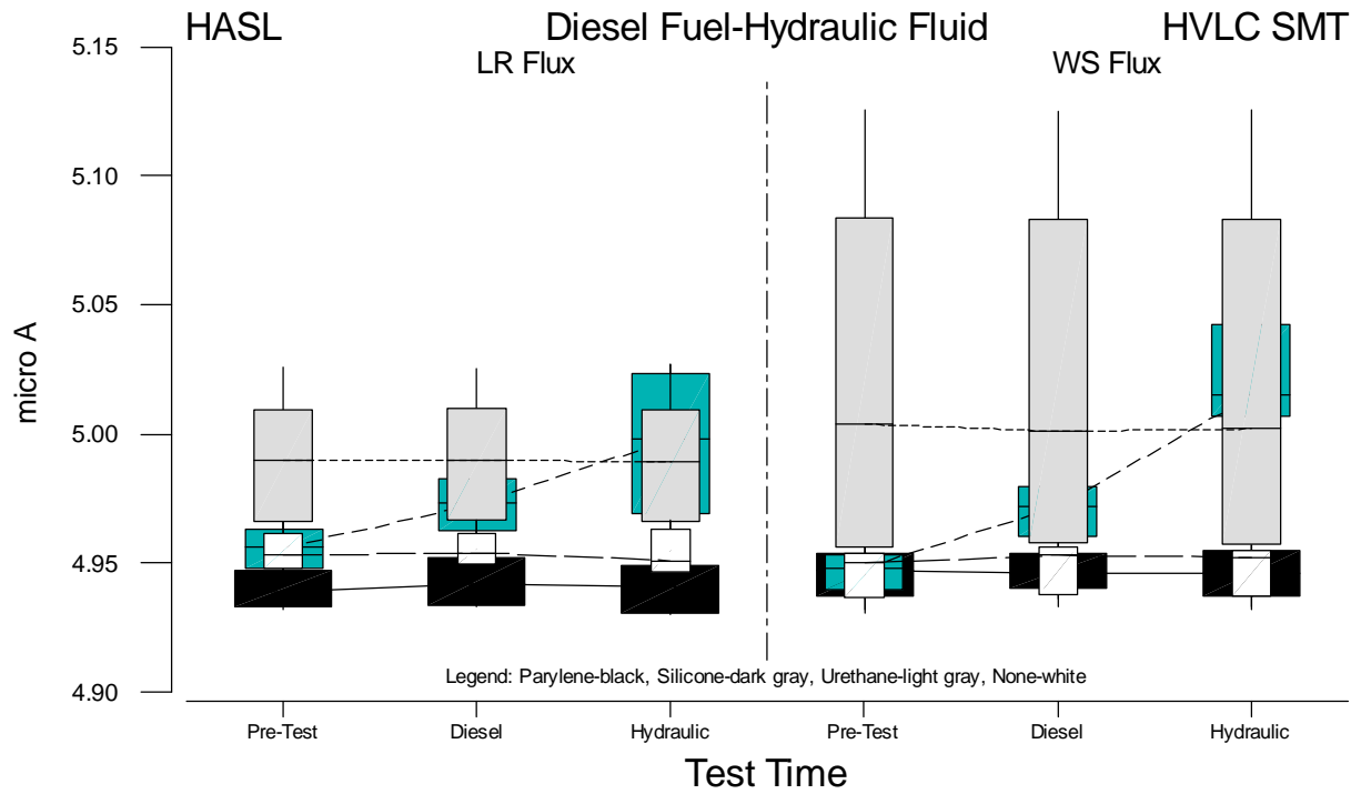
Figure B.13 Boxplots of HVLC SMT Current Measurements for HASL versus Test Time
