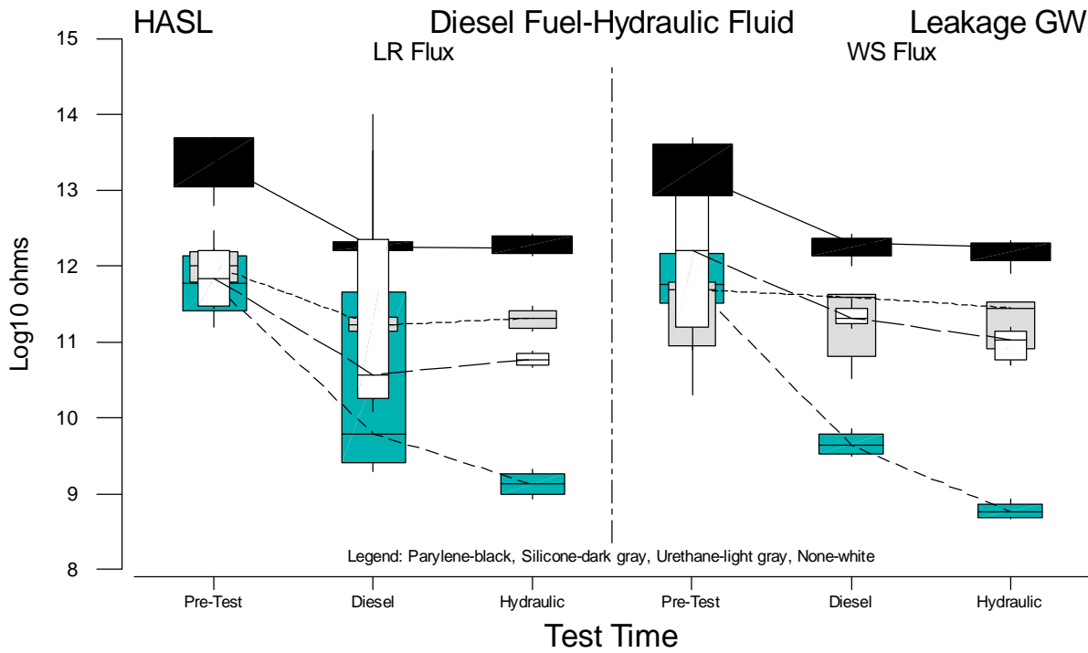
Figure B.81 Boxplots of Gull Wing Leakage Measurements for HASL versus Test Time
