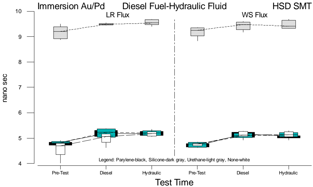
Figure B.24 Boxplots of HSD SMT Propagation Delay Measurements for Immersion Au/Pd vs. Test Time
