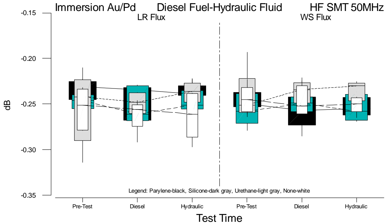
Figure B.40 Boxplots of HF SMT 50MHz Measurements for Immersion Au/Pd versus Test Time
