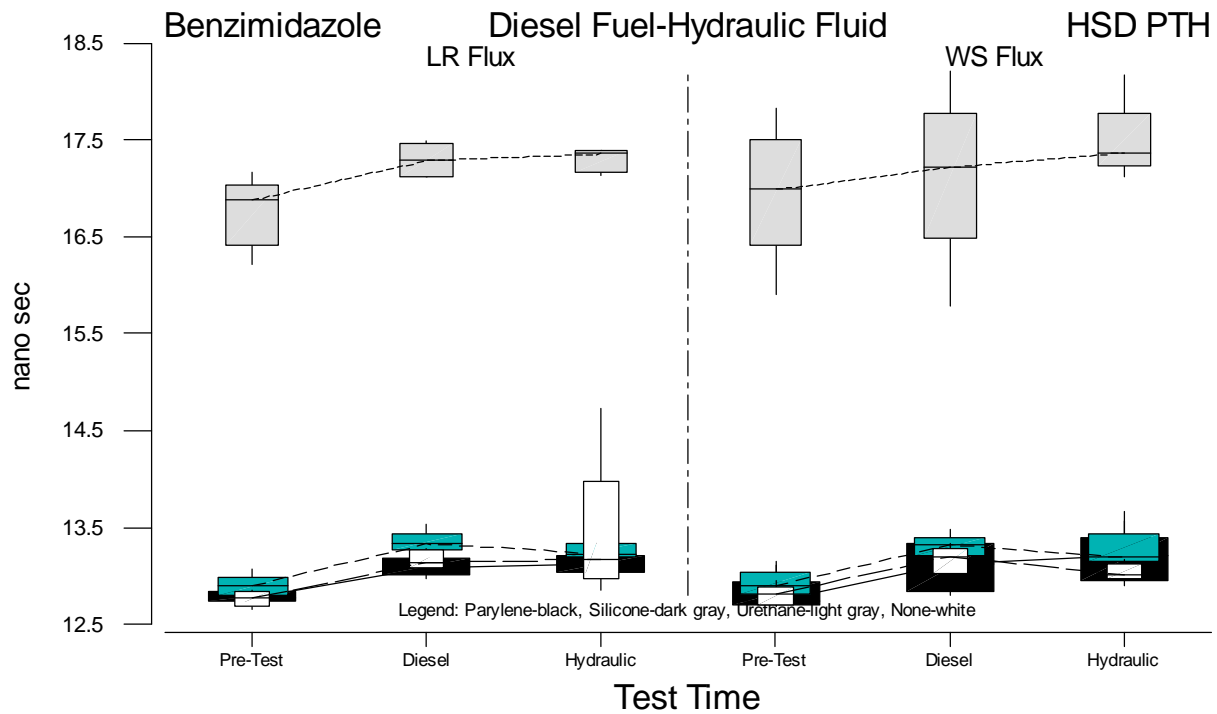
Figure B.18 Boxplots of HSD PTH Propagation Delay Measurements for Benzimidazole versus Test Time
