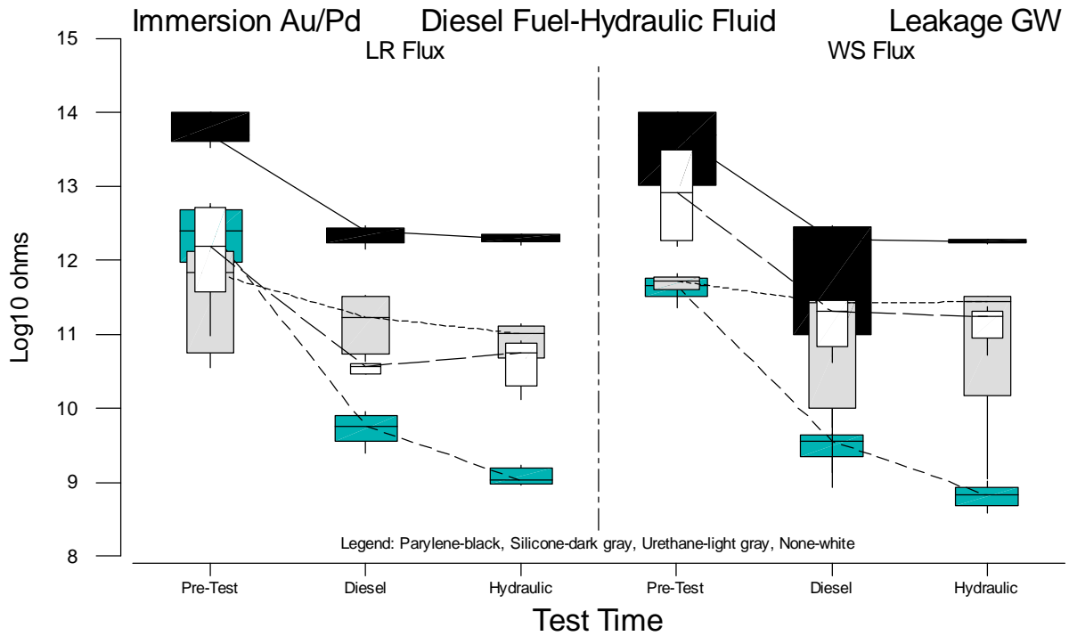
Figure B.84 Boxplots of Gull Wing Leakage Measurements for Immersion Au/Pd vs. Test Time
