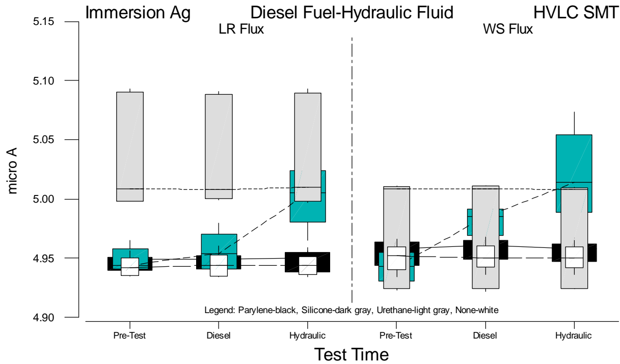
Figure B.15 Boxplots of HVLC SMT Current Voltage Measurements for Immersion Ag versus Test Time
